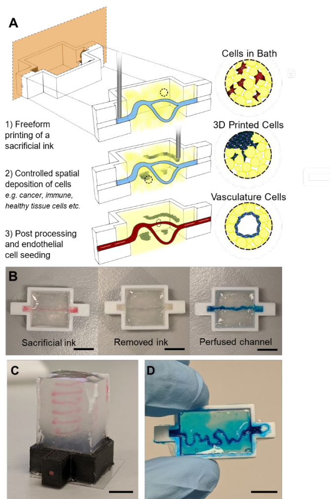
Figure 1. Photocrosslinking to stabilize suspension microgels allows for complex organization of cells in three distinct ways. A) (1) An uncrosslinked microgel suspension, with or without cells, is placed in a reactor where a sacrificial ink is freely printed. (2) More cell types can further be printed as different shapes and sizes at various proximities to the sacrificial ink. (3) The suspension is photocrosslinked followed by removal of the sacrificial ink and subsequent seeding of endothelial cells on the hollow channel walls. B) Macro images of the three stages of hollow channel formation: printing of the ink, photocrosslink and
