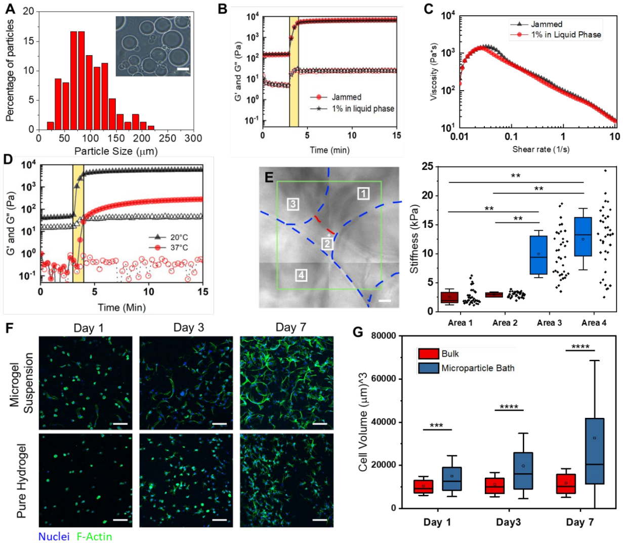
Figure 2. Characterization of GelMa microparticle support suspensions for 3D printing. A) Size distribution ( n=100 ) of the 10 wt% GelMa microparticles. Inset image is a representative optical image of the microparticles. B) Rheological analysis of the gelation of suspensions with (red markers) and without (black markers) a 1 wt% GelMa filler in the liquid phase. Closed markers are the storage modulus ( G' ) and open markers are the loss modulus ( G'' ). The yellow bar indicates UV crosslinking. C) Uncrosslinked microgel viscosity as a function of Shear rate for suspensions with (red markers) and without (black markers) filler. D) Effect of melting a microgel suspension (red markers) on the storage modulus ( G' ) when compared to unmelted heterogenous suspension (black markers). The yellow bar indicates UV crosslinking. E) Contact mode atomic force microscopy (AFM) over 4 regions of a suspension bath surface. Force curves ( n = 36 per square) were taken at each 10\mu\text{m} \times 10\mu\text{m} region of the surface where the analyzed young's modulus is plotted for each region's curves. F) Z-stack Projections ( 100\mu\text{m} z-stacks of 50 slices) of ADSCs stained with Hoechst (blue) and Phalloidin (green) in microgel suspensions and a pure hydrogel (10 wt% GelMa). G) Box plots of cell volume quantification of microgel suspensions vs pure hydrogels over 7 days. Scale bars: 10\mu\text{m} (E), 100\mu\text{m} (F).
