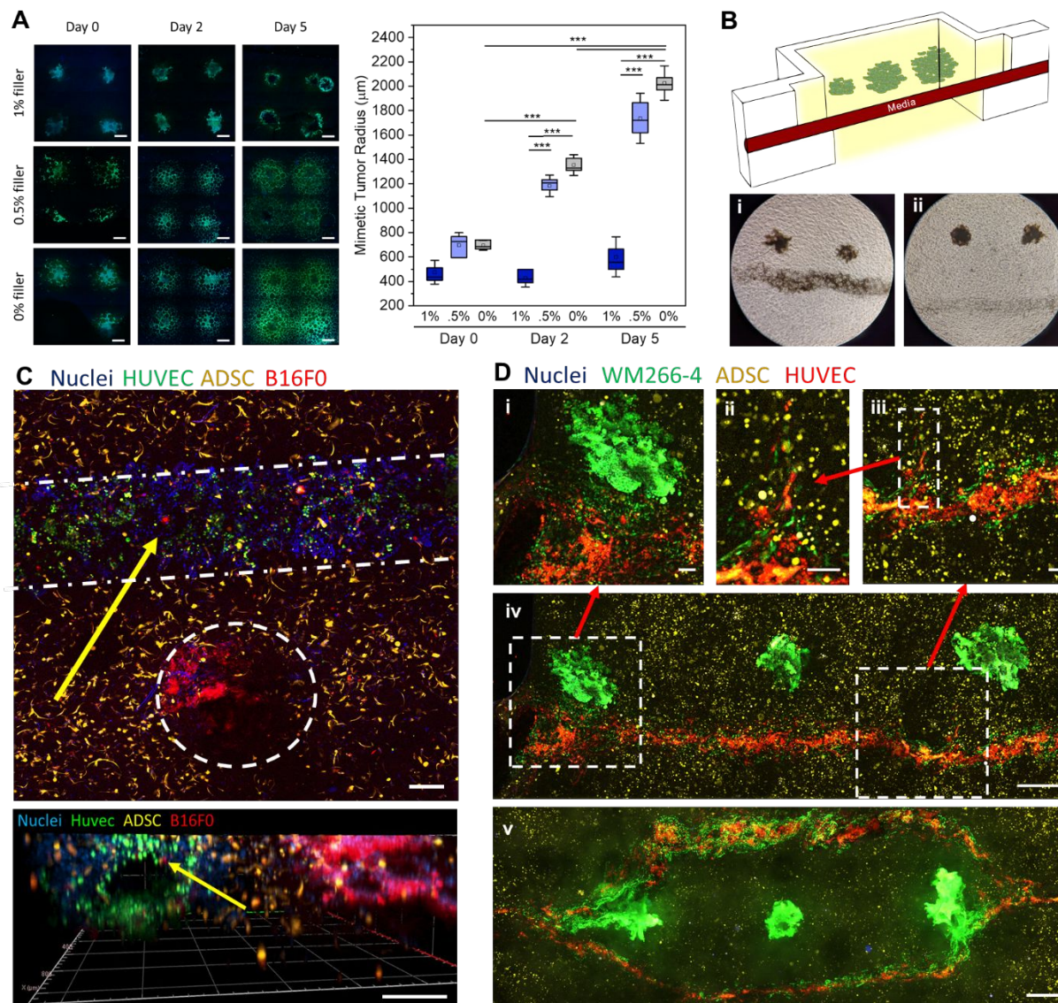
Figure 5. Printed cancer cell properties and triculture metastasis models. A) Confocal images of WM266-4 cancer cells printed into granular gels with 3 varied filler percentages at times points of 0, 2, and 5 days. Mimetic tumor radii were quantified at each time point and plot ( n=5-12 , P<0.0001 ). B) A schematic of the tumor invasion model without perfusion (left) and phase contrast images of tumors printed close (i) and far (ii) from the vasculature. A 10x phase contrast image of tumor cells migrating towards vasculature in a close print (iii). C) Confocal Z-projection of a triculture of ADSCs, HUVECs in a channel, and printed B16F0 cell pellets (top) along with a 3D projection (Zen blue, Zeiss) of that same gel (bottom). D) Printed WM266-4 melanoma cells near straight (iv) and bifurcated (v) endothelial lined vasculatures. (i) represents a zoom in of cell migration from tumor to vasculature while (ii-iii) represent two successive zoom ins of endothelial angiogenesis. Scale bars: 100 \mu\text{m} (D (i, ii, iii)), 200 \mu\text{m} (C), 400 \mu\text{m} (A), 500 \mu\text{m} (D (iv, v)).
