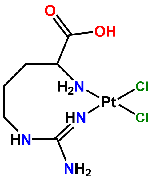
NN_s Binding Mode
