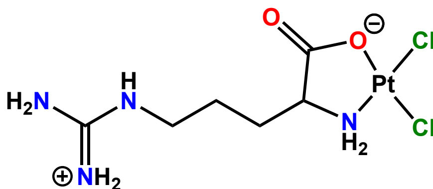
NO^- Binding Mode
