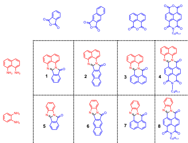
Figure 1. Structures of the molecules investigated in this study.
