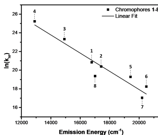
Figure 6. Energy-gap law plot of chromophores 1-8.
