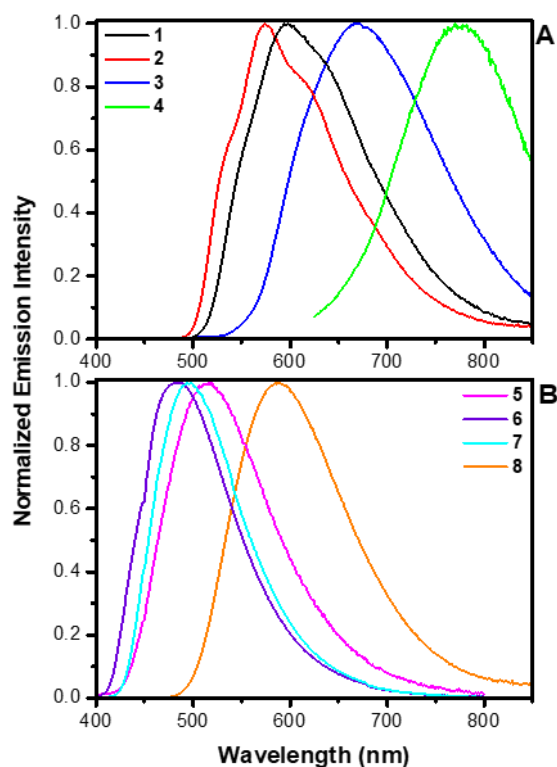
Figure 5. Photoluminescence spectra of 1-4 (A) and 5-8 (B) in aerated THF.
