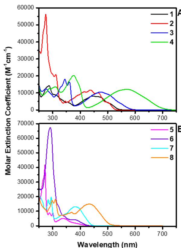
Figure 4. Electronic spectra of 1-4 (A) and 5-8 (B) in THF.
