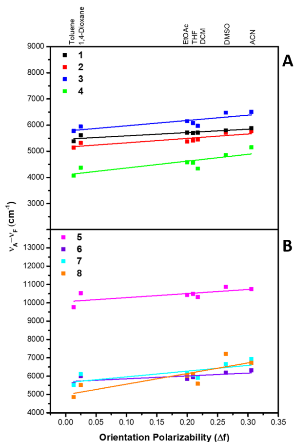
Figure 8. Lippert-Mataga plots of chromophores 1-4 (A) and 5-8 (B) in aprotic solvents.
