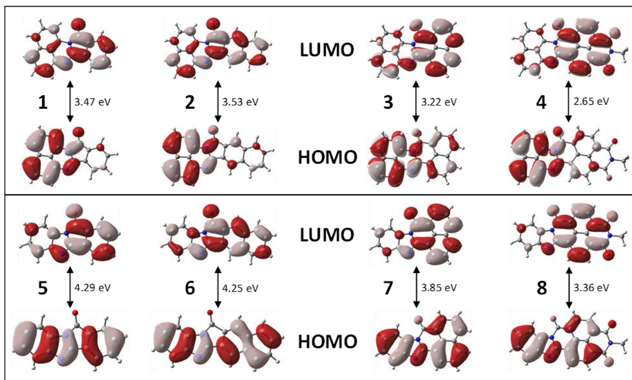
Figure 3. Pictorial representations of highest occupied and lowest unoccupied molecular orbitals for 1-8 . Calculations performed at M06-D3/Def2-TZVP level of theory with PCM correction.
