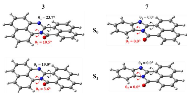
Figure 2. Optimized geometries of S_0 (top) and S_1 (bottom) of 3 (left) and 7 (right). Geometry optimizations performed at M06-D3/Def2-TZVP level of theory.
