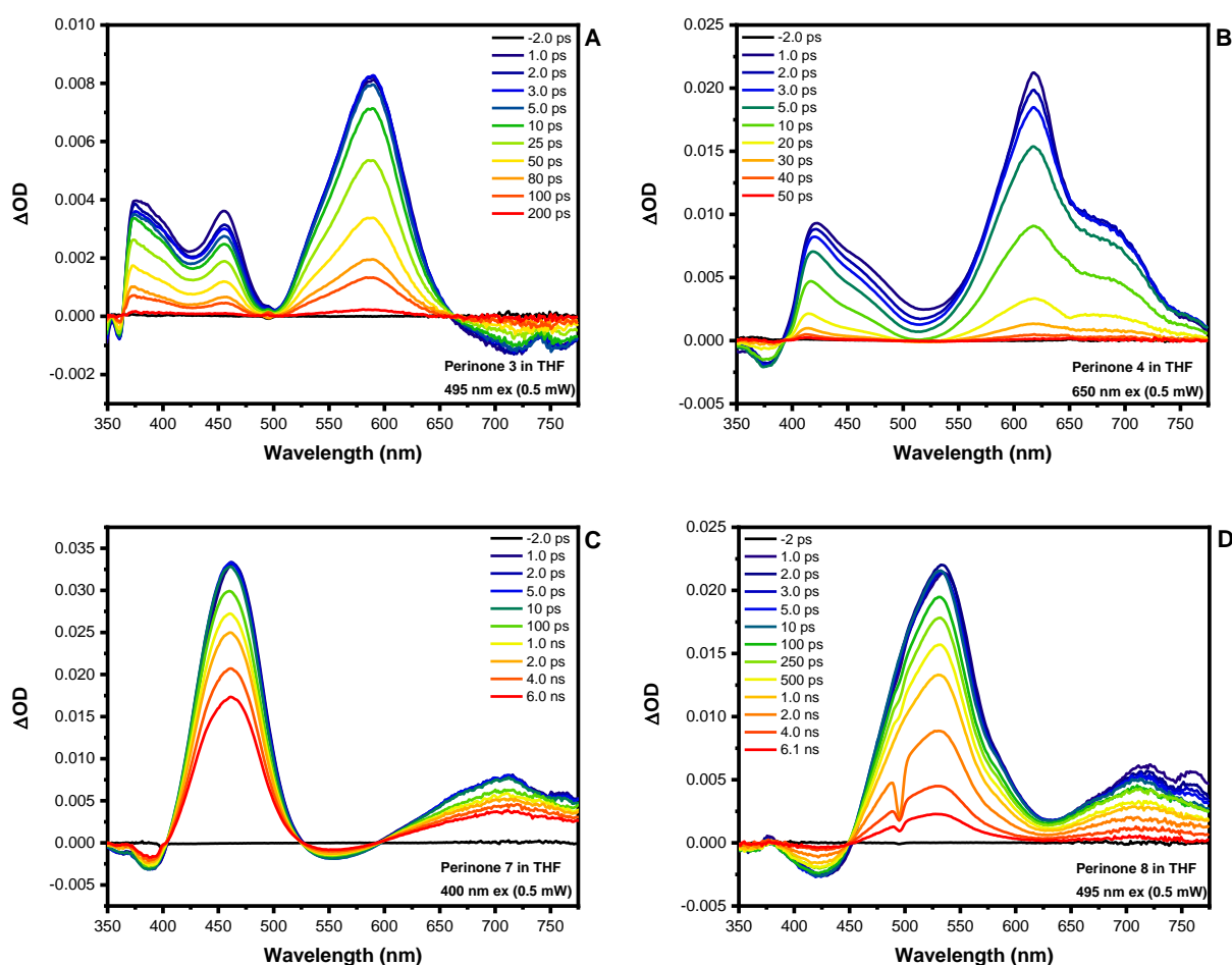
Figure 7. Excited-state difference spectra of 3 (A) in THF following 495 nm pulsed excitation, 4 (B) in THF following 650 nm pulsed excitation, 7 (C) in THF following 400 nm pulsed excitation, and 8 (D) in THF following 495 nm pulsed excitation (105 fs fwhm).
