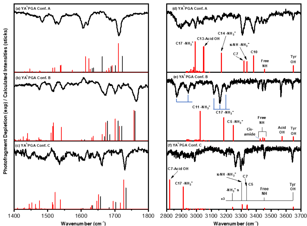
Figure 4. Conformation Specific Infrared Spectra of [YA^L\text{PGA} + H]^+ . (a-c): Corresponding experimental and calculated spectra in the 1400\text{--}1800\text{ cm}^{-1} region. The black stick spectra are the results of a harmonic treatment using a single scale factor for all vibrations in the 1600\text{--}1800\text{ cm}^{-1} region, while the red stick spectra are those resulting from the local mode Hamiltonian model. See text for further discussion. (d-f): Conformation specific infrared spectrum of the three observed conformers of [YA^L\text{PGA} + H]^+ (black) in the hydride stretch region, compared to the calculated vibrational frequencies and infrared intensities of the best-fit conformations.
