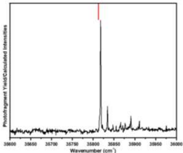
Figure 5. UV photofragment spectrum of cryo-cooled [\text{YAA}^{\text{D}}\text{PGAAA}+\text{H}]^+ in the S_0 - S_1 origin region with corresponding TD-DFT calculated electronic origin of assigned conformation in red.
