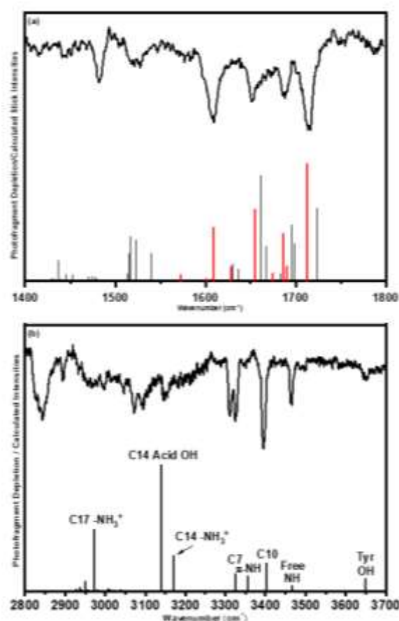
Figure 2. IR spectrum of \text{YA}^{\text{D}}\text{PGA} with calculated sticks. (a) Corresponding experimental and calculated spectra in the 1400 - 1800 \text{ cm}^{-1} region. The black stick spectra are the results of a harmonic treatment using a single scale factor for all vibrations in the 1600 - 1800 \text{ cm}^{-1} region, while the red stick spectra are those resulting from the local mode Hamiltonian model. See text for further discussion. (b) Conformation specific infrared spectrum of the single conformer of [\text{YA}^{\text{D}}\text{PGA} + \text{H}]^+ (black) in the hydride stretch region, compared to the calculated vibrational frequencies and infrared intensities of the best-fit conformation, which is also the global minimum.
