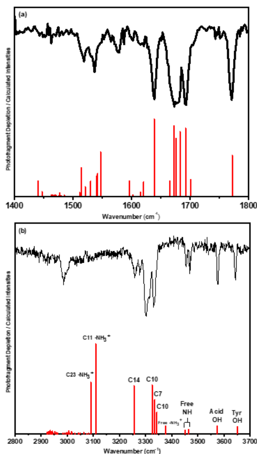
Figure 6. Infrared spectrum of [\text{YAA}^{\text{D}}\text{PGAAA}+\text{H}]^+ . (a) Corresponding experimental and calculated spectra in the 1400 - 1800\text{ cm}^{-1} region using the local mode Hamiltonian model. (b) Conformation specific infrared spectrum of the single observed conformer of [\text{YAA}^{\text{D}}\text{PGAAA}+\text{H}]^+ (black) in the hydride stretch region, compared to the calculated vibrational frequencies and infrared intensities of the best-fit conformation, which is also the global minimum.
