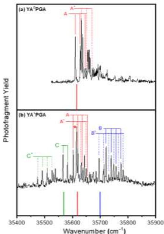
Figure 1. UV spectra of \text{YA}^{\text{D}}\text{PGA} and \text{YA}^{\text{L}}\text{PGA} . UV action spectra of (a) [\text{YA}^{\text{D}}\text{PGA} + \text{H}]^+ and (b) [\text{YA}^{\text{L}}\text{PGA} + \text{H}]^+ . The origins and Franck-Condon progressions of the different conformers are labelled A, B, and C with the asterisk denoting transitions due to tyrosine rotamers of the conformer. Below each UV spectrum is a colored stick denoting the TD-DFT calculated (M052X/6-31+g(d)) electronic origin of the assigned conformation, after scaling by 0.8443. See text for further discussion.
