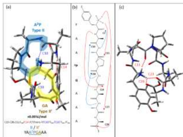
Figure 7. (a) Calculated lowest energy structure of [\text{YAA}^{\text{D}}\text{PGAAA} + \text{H}]^+ showing the sequential \beta -turns from a side view. The individual turns are highlighted in blue and yellow. (b) Stick structure with highlighted hydrogen bonding pattern. A red arrow indicates an N-to-C terminal \text{NH}\cdots\text{O}=\text{C} hydrogen bond while a blue arrow is indicative of the opposite. (c) Top-down view of the structure highlighting the binding pocket surrounding the \text{NH}_3^+ .
