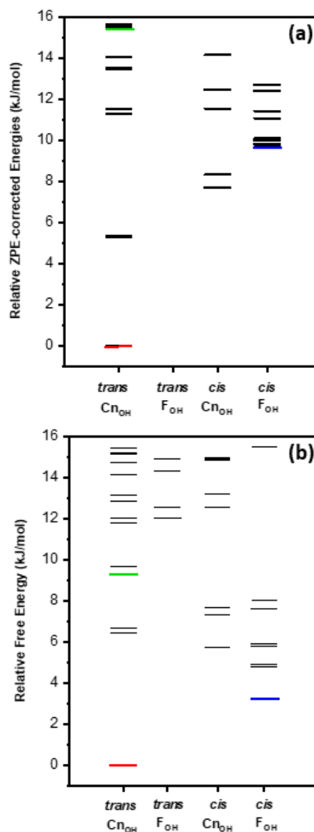
Figure 8. (a) Relative energies at 0 K, including vibrational zero-point energy corrections, for the conformers of [\text{YA}^{\text{L}}\text{PGA} + \text{H}]^+ . The horizontal axis divides the structures into groups based upon the presence or absence of a cis amide bond in the non-Pro amino acids ( cis/trans ) and whether the acid OH is in a hydrogen bond ( \text{Cn}_{\text{OH}} ) or not ( \text{F}_{\text{OH}} ). Each line in the figure represents the energy of a calculated structure while the energies of the three conformers that have best fits to the observed conformers are shown in red (conformers A), blue (conformer B), and green (conformer C). (b) Gibbs Free Energy ( \Delta G 298K) level diagram for [\text{YA}^{\text{L}}\text{PGA} + \text{H}]^+ with relative energy on the y-axis. The lines labeled in red (conformer A), blue (conformer B), and green (conformer C) mark the energies of the best fit structures to each infrared spectrum.
