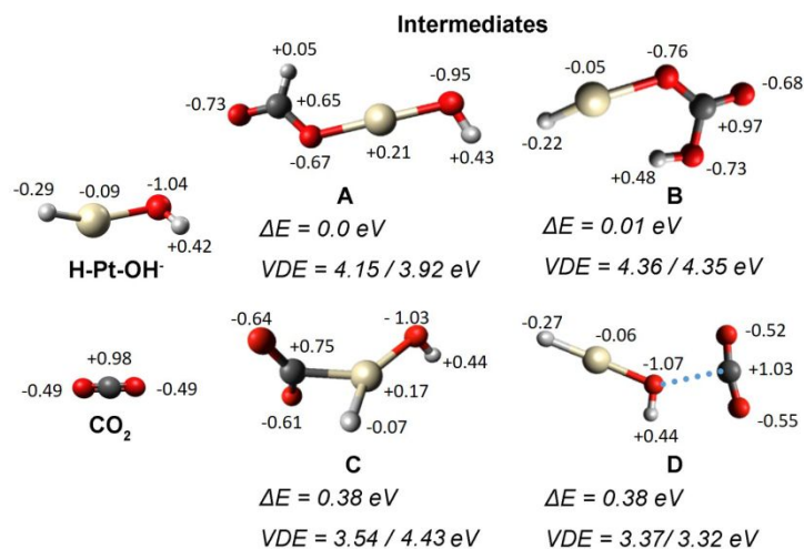
Figure 3. Optimized structures for H-Pt-OH - , CO 2 , and [H-Pt-OH(CO 2 )] - . The relative energies of [H-Pt-OH(CO 2 )] - and their calculated VDEs to singlet and triplet neutrals are shown below each structure. The Natural Bond Orbital (NBO) charge on each atom is also provided.
