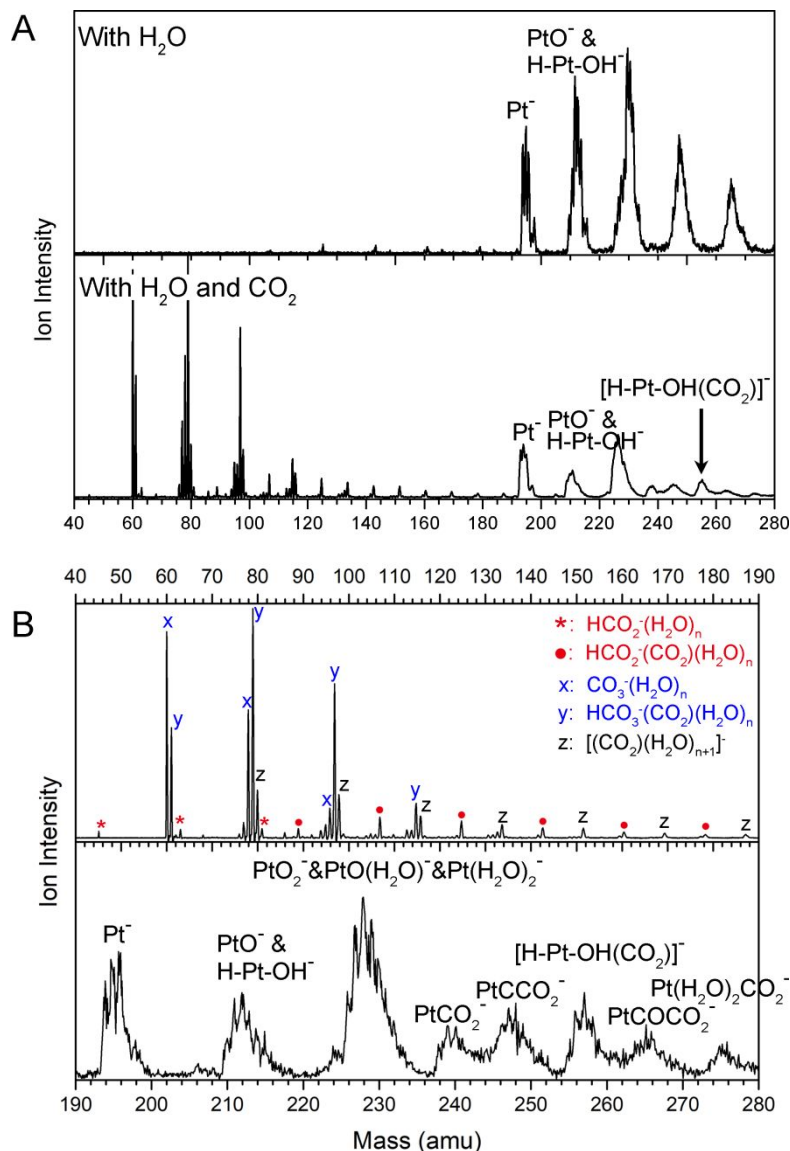
Figure 1. (A) Mass spectra of Pt - reacting with H 2 O (top panel) and with H 2 O and CO 2 (bottom panel). (B) The mass spectrum of Pt - with H 2 O and CO 2 is bisected into the lower (top panel) and higher (bottom panel) mass regions for a closer view of the reaction products.
