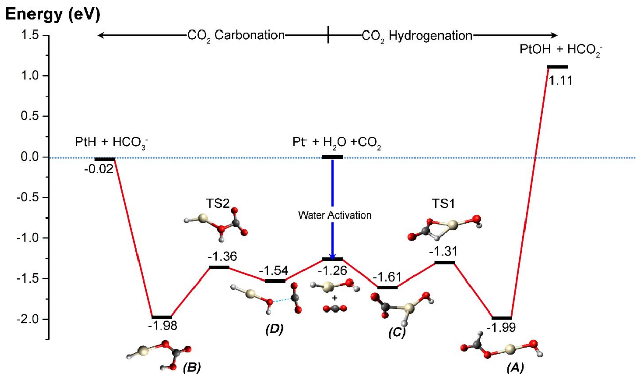
Figure 4. Profile of the molecular-level CO 2 RR mediated by anionic Pt atoms. Zero-point corrected energies are given in eV. The letters in parentheses correspond to their labels in Figure 3. The potential energy surface is referenced to the total energy of isolated Pt - , H 2 O, and CO 2 .
