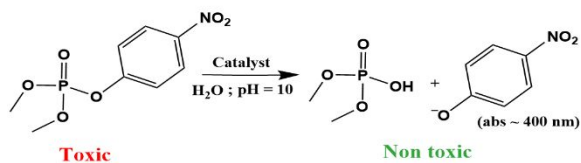
Figure 1. Hydrolysis of DMNP, simulant of nerve agent Soman (GD), using a catalyst under basic buffer conditions.
