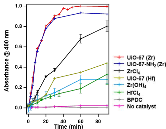
Figure 2. Progress of DMNP hydrolysis catalyzed by UiO-67 MOFs and their precursors monitored by the formation of 4-nitrophenolate using UV-vis spectroscopy.
