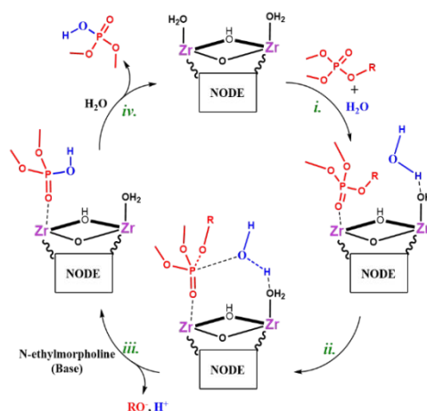
Figure 4. Mechanism of base catalyzed hydrolysis of DMNP by zirconium oxy-hydroxide. (In figure, R: 4- nitrophenyl)
