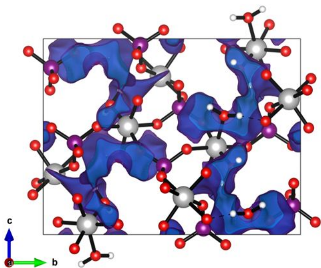
Figure 8. Projection of bond valence energy landscape calculated for onto (bc) plane. Darker colours are assigned for inner isosurface levels ( > 0.7 eV) while the lighter hues indicate the outer levels ( < 0.65 eV).
