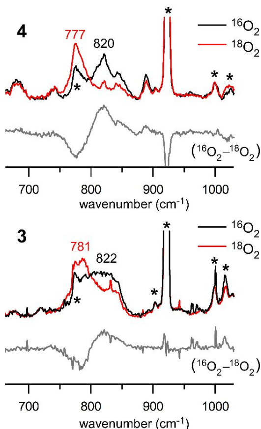
Figure 5. Resonance Raman spectra of 4 (top) and 3 (bottom) in frozen \text{CH}_3\text{CN} (77 K). Samples were prepared using either ^{16}\text{O}_2 (black lines) or ^{18}\text{O}_2 (red lines). Derivative-shaped features in the ^{16}\text{O}_2 - ^{18}\text{O}_2 difference spectra (gray lines) are due to isotopically-active peaks. All spectra were measured using 501.7 nm laser excitation at a power of 20 – 30 mW at the sample. The solvent-derived features marked with an asterisk (*) were used to normalize spectral intensities.
