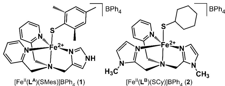
Scheme 2. Structures of complexes 1 and 2 .
