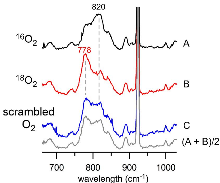
Figure 6. Resonance Raman spectra of 4 in frozen \text{CH}_3\text{CN} collected using 501.7 nm excitation (24–30 mW at sample). The samples were prepared by treating 10 mM solutions of 2 with ^{16}\text{O}_2 (A, black line), ^{18}\text{O}_2 (B, red line), or scrambled \text{O}_2 (C, blue line). The bottom spectrum (gray line), generated by digital addition, is half the sum of spectra A and B. Solvent-derived peaks were used to normalize spectral intensities.
