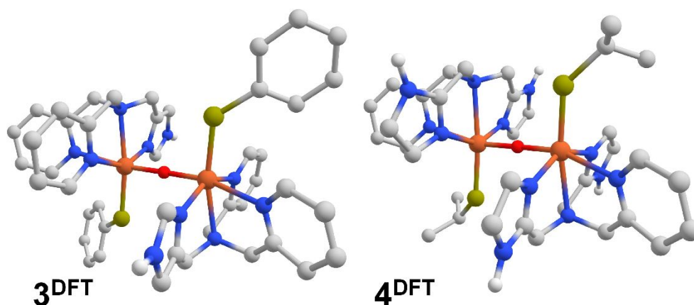
Figure 8. DFT geometry-optimized models of intermediates 3 and 4 . Most hydrogen atoms are omitted for the sake of clarity. The thiolate ligands have been modified as described in Computational Methods. Atomic colors: C, gray; N, blue; O, red; S, yellow; Fe, orange.
