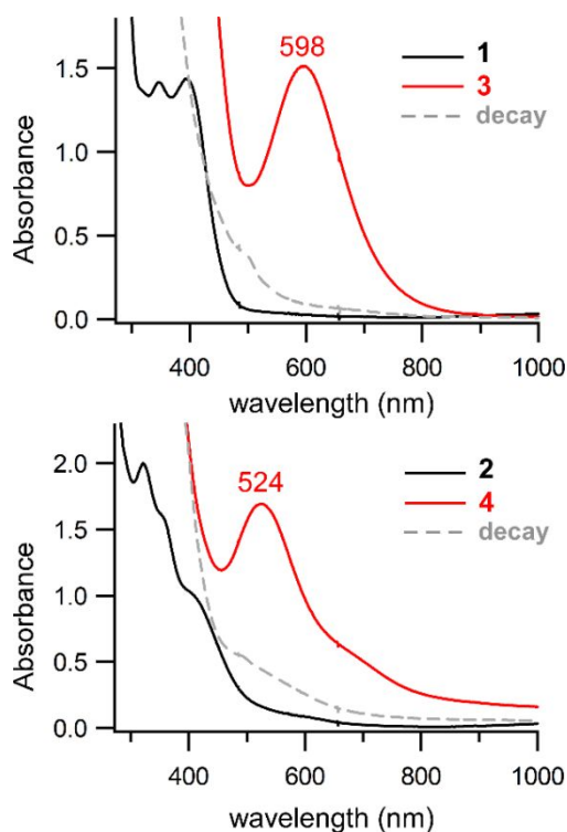
Figure 1. UV-vis absorption spectra of the reaction of 1 (top) and 2 (bottom) with O 2 in CH 3 CN at -40 °C. Spectra of the Fe(II) precursors ( 1 and 2 ) and O 2 -generated intermediates ( 3 and 4 ) are shown as black and red lines, respectively. The initial concentrations of 1 and 2 were 1.3 mM. The decay spectra (gray dashed lines) were obtained by warming solutions of 3 and 4 from -40 °C to room temperature.
