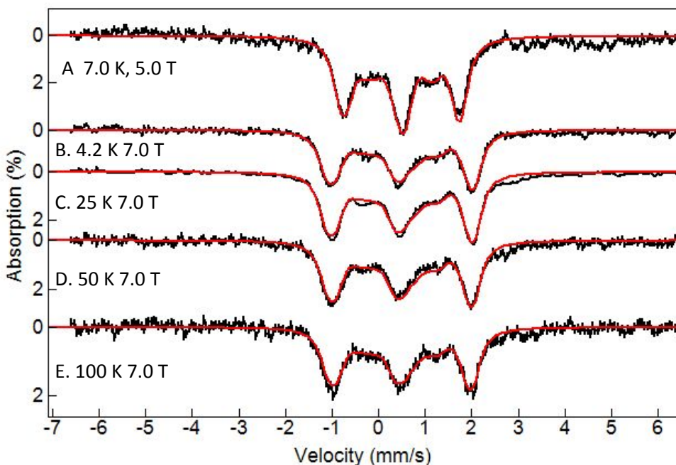
Figure 4. Variable-field, variable-temperature Mössbauer spectra of complex 4 . The hatch marks are the experimental data, and the colored lines are spectral fits generated with the parameters in Table 1 as described in Experimental Methods.
