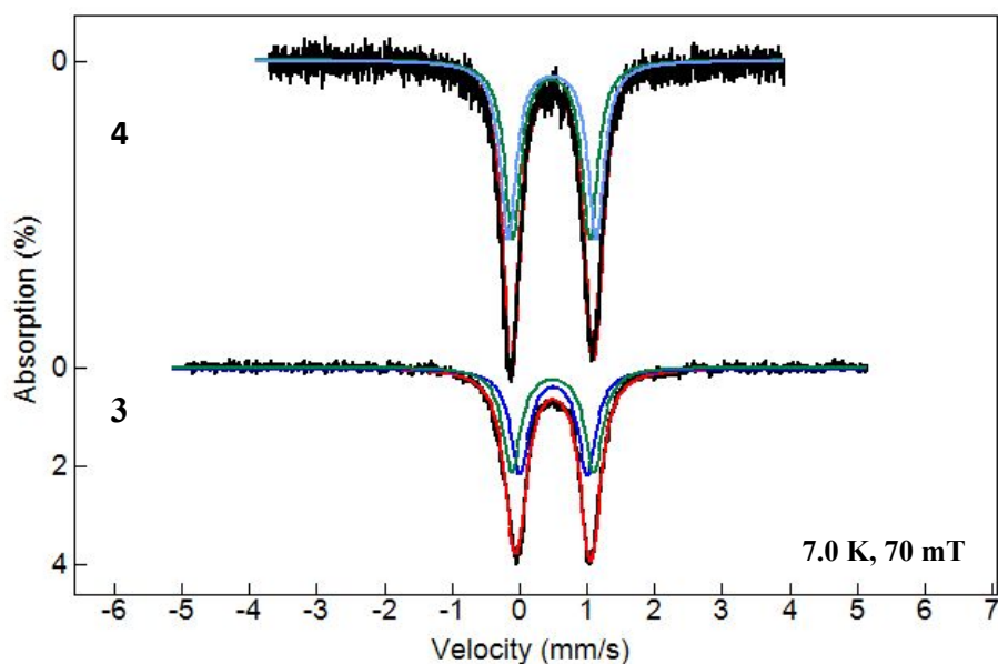
Figure 3. Mössbauer spectra of complexes 3 and 4 measured at 7.0 K and 70 mT, prepared as described in the text. The hatch marks are the experimental data, and the colored lines are spectral fits generated with the parameters in Table 1. For clarity, both spectra were prepared by removing the unreacted Fe(II) species from the raw data.
