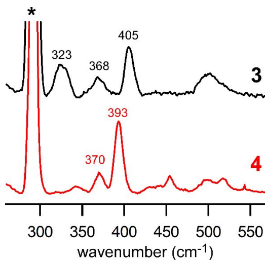
Figure 7. Resonance Raman spectra of 3 and 4 in frozen \text{CD}_2\text{Cl}_2 (77 K). Spectra were collected with laser excitation of 514.5 nm ( 3 ) and 501.7 nm ( 4 ). Samples were prepared by addition of \text{O}_2 to solutions of the precursor complexes. The solvent-derived peak marked with an asterisk (*) was used to normalize spectral intensities.
