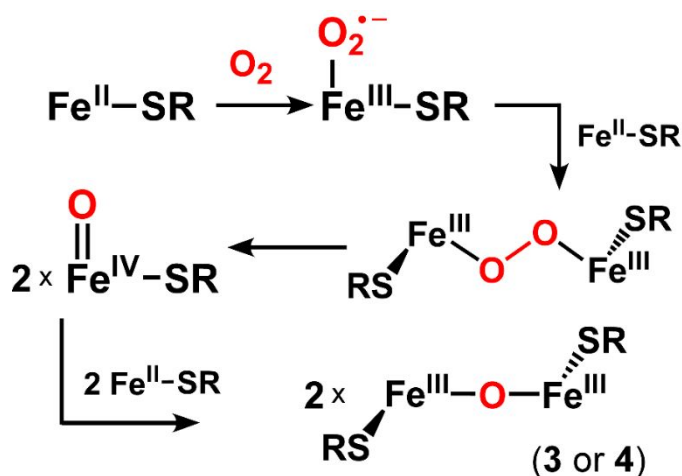
Scheme 3. Proposed Mechanism for Formation of Intermediates 3 and 4 .
