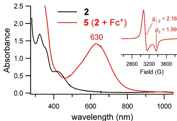
Figure 2. UV-vis spectra of the oxidation of complex 2 (black line) to 5 (red line) via addition of one equivalent of [\text{Fc}]\text{PF}_6 . The reaction occurred in \text{CH}_3\text{CN} at -40\text{ }^\circ\text{C} . The initial concentration of 2 was 0.90 mM. Inset: X-band EPR spectrum of 5 measured at 10 K in frozen \text{CH}_3\text{CN} . Data were collected at a frequency of 9.39 GHz and power of 2.0 mW.
