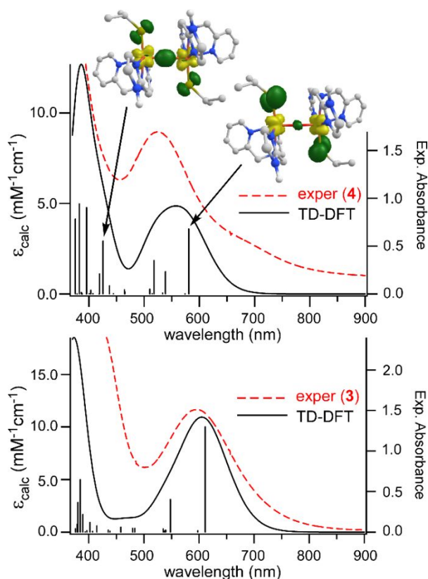
Figure 9. TD-DFT computed absorption spectra (solid black lines) of intermediates 4 (top) and 3 (bottom). The black sticks correspond to the energies and intensities of computed transitions. The TD-DFT spectra are compared to experimental spectra (dashed red lines) measured in CH 3 CN at -40 °C (initial Fe concentration of 1.3 mM). The inset displays electron density difference maps for two intense transitions in the computed spectrum of 4 . The green and yellow areas represent the loss and gain, respectively, of electron density during the excitation.
