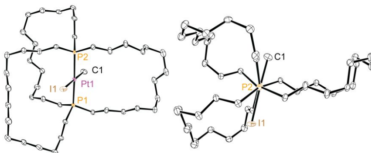
Figure 4. Thermal ellipsoid plots of the molecular structure of trans-10c (50% probability level, dominant conformation).
