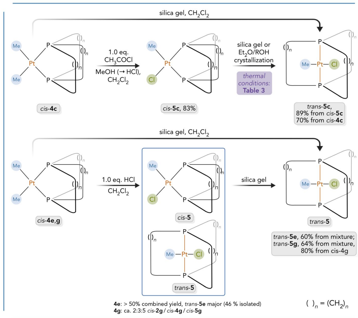
Scheme 5. Introduction of halide ligands and attendant isomerization.
