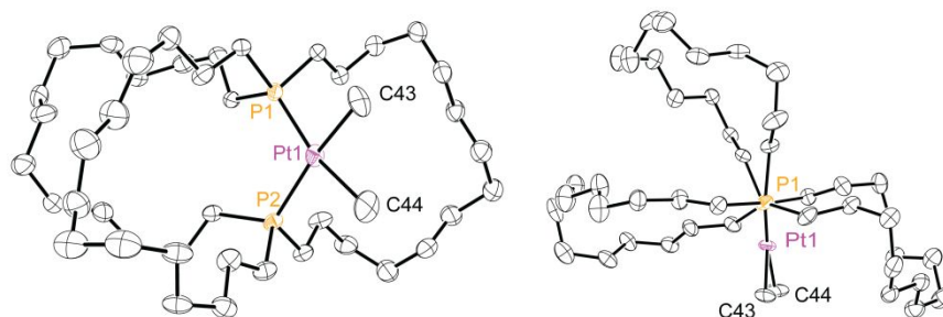
Figure 1. Thermal ellipsoid plots of the molecular structure of cis-4c (50% probability level, dominant conformation).
