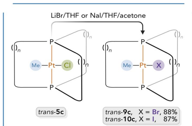
Scheme 8. Halide substitution reactions.
