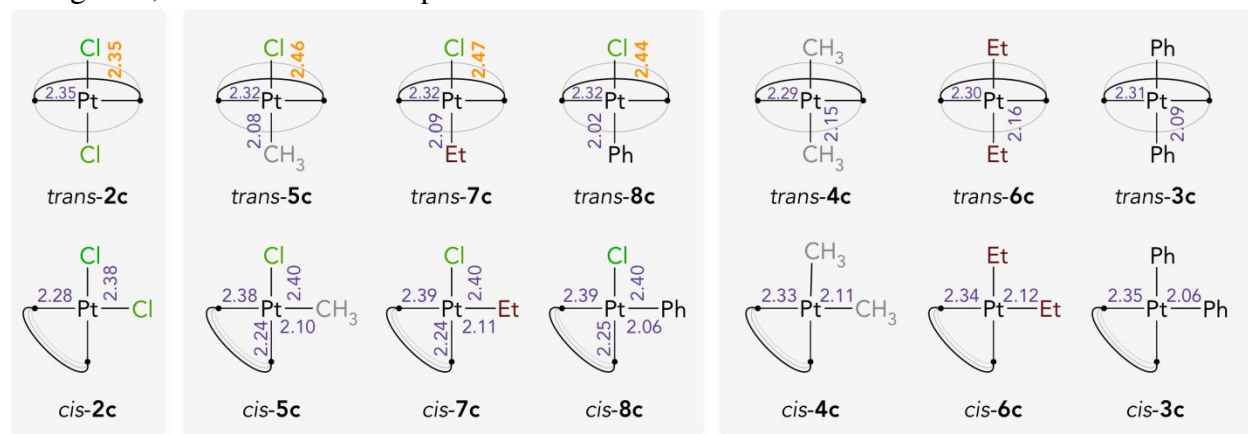
Figure 7. Platinum-ligand bond lengths (Å) for computed trans /gyroscope and cis /parachute complexes.
