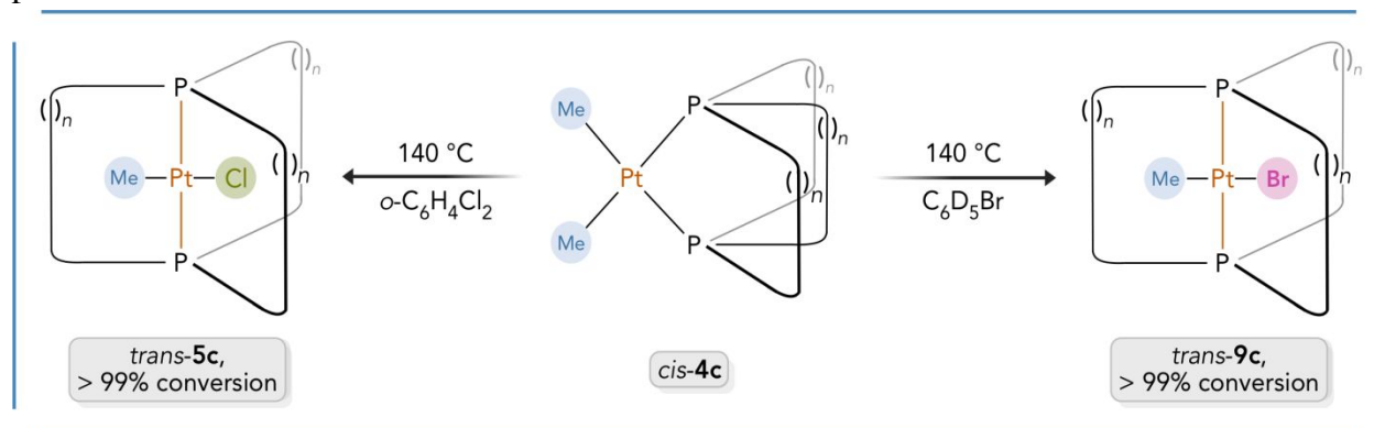
Scheme 9. Thermolyses that afford well defined complex/solvent reactions.
