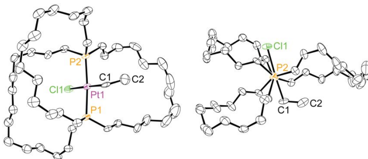
Figure 3. Thermal ellipsoid plots of the molecular structure of trans-7c (50% probability level, one of three independent molecules).
