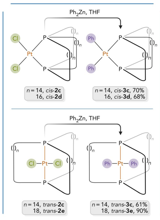
Scheme 3. Stereospecific substitution of chloride ligands by phenyl ligands in trans and cis platinum complexes.
