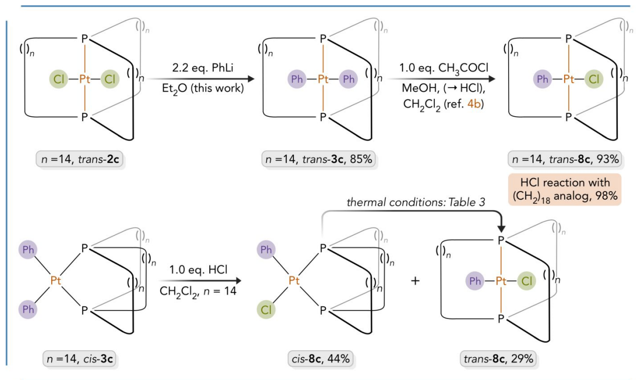
Scheme 7. Substitution and isomerization reactions involving phenyl ligands.
