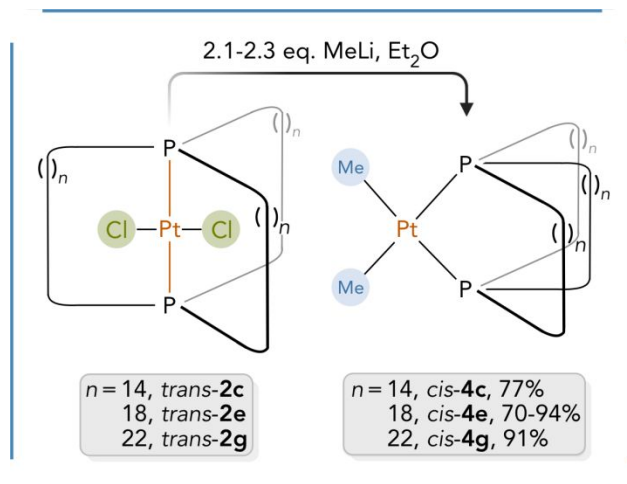
Scheme 4. Substitution of the chloride ligands in trans - 2c,e,g by methyl ligands with isomerization.
