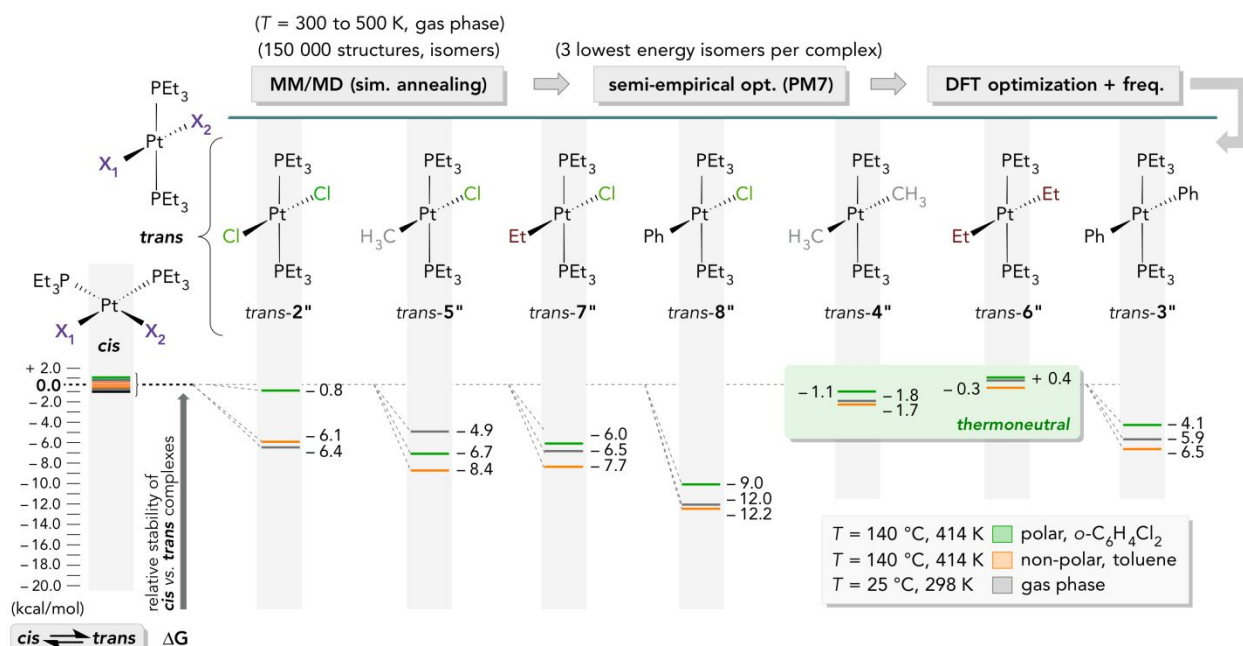
Figure 6. Relative energies ( \Delta G , kcal/mol) of isomeric cis and trans platinum complexes with acyclic triethylphosphine ligands as computed by DFT (gas phase or toluene or o -C 6 H 4 Cl 2 solutions) preceded by molecular dynamics and semi-empirical (PM7) computations.
