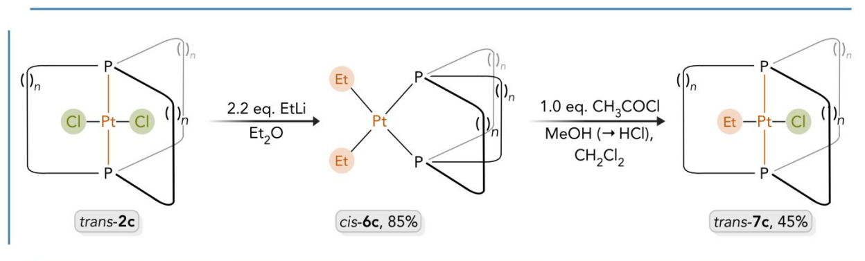
Scheme 6. Substitution and isomerization reactions involving ethyl ligands.
