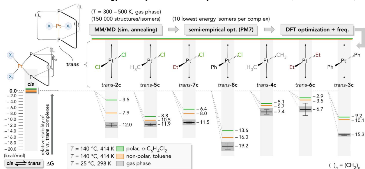
Figure 5. Relative energies ( \Delta G , kcal/mol) of isomeric cis /parachute and trans /gyroscope platinum complexes as computed by DFT (gas phase or toluene or o\text{-C}_6\text{H}_4\text{Cl}_2 solutions) preceded by molecular dynamics and semi-empirical (PM7) computations.
