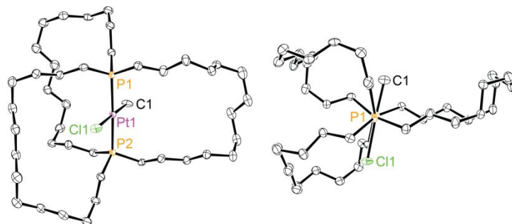
Figure 2. Thermal ellipsoid plots of the molecular structure of trans-5c (50% probability level, dominant conformation).
