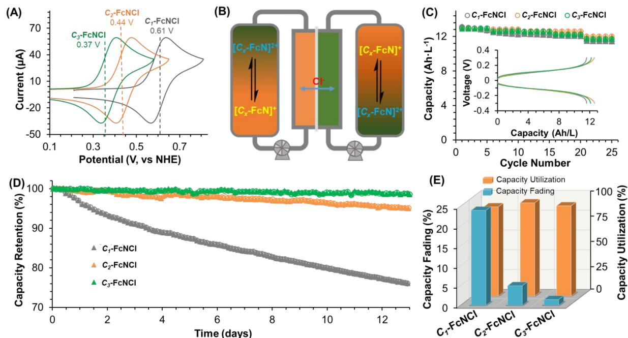
Figure 2. Cyclic voltammograms and half-cell RFB studies of the C_x -FcNCl catholytes. (A) Cyclic voltammograms of the Fc derivatives; (B) The scheme of C_x -FcNCl half-cell RFBs; (C) Charge ( \circ ) and discharge ( \blacktriangle ) capacity versus cycling number at from 10 to 50 \text{mA}/\text{cm}^2 current densities for 0.50 M C_1 -FcNCl (gray), C_2 -FcNCl (orange), and C_3 -FcNCl (green) half-cell RFBs; Inset: representative charge and discharge profiles at 40 \text{ mA}/\text{cm}^2 ; (D) Capacity retention of 0.50 M C_x -FcNCl half-cell RFBs at 40 \text{ mA}/\text{cm}^2 during 13 testing days: C_1 -FcNCl (gray), C_2 -FcNCl (orange), and C_3 -FcNCl (green); (E) Comparison of initial capacity utilization (orange) and capacity fading percentages (blue) of the C_x -FcNCl half-cell RFBs at 40 \text{ mA}/\text{cm}^2 in 13 testing days. CV conditions: 2 mM C_x -FcNCl in 0.50 M \text{NH}_4\text{Cl} aqueous solution, 100 \text{mV}/\text{s} scan rate, glassy carbon working and counter electrodes, Ag/AgCl reference electrode. RFB conditions: catholyte, 0.50 M C_x -FcNCl in 1.00 M.
