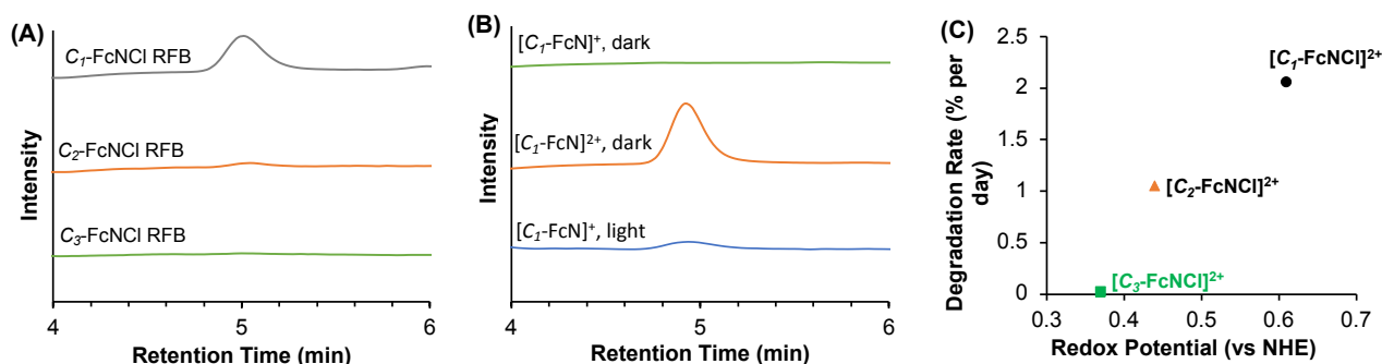
Figure 4. Gas chromatography (GC) studies and correlation of redox potential and stability. (A) GC curves of the gas phase samples collected from electrolyte reservoirs of the C_x\text{-FcNCl} half-cell RFBs after 13 days of cycling. (B) GC curves of gas phase samples upon keeping 0.50 M discharged state [C_1\text{-FcN}]^+ and charged state [C_1\text{-FcN}]^{2+} water solutions in sealed vials for 5 days. (C) The correlation of the degradation rate of the charged state [C_x\text{-FcN}]^{2+} series measured by UV-Vis vs. their redox potential.
