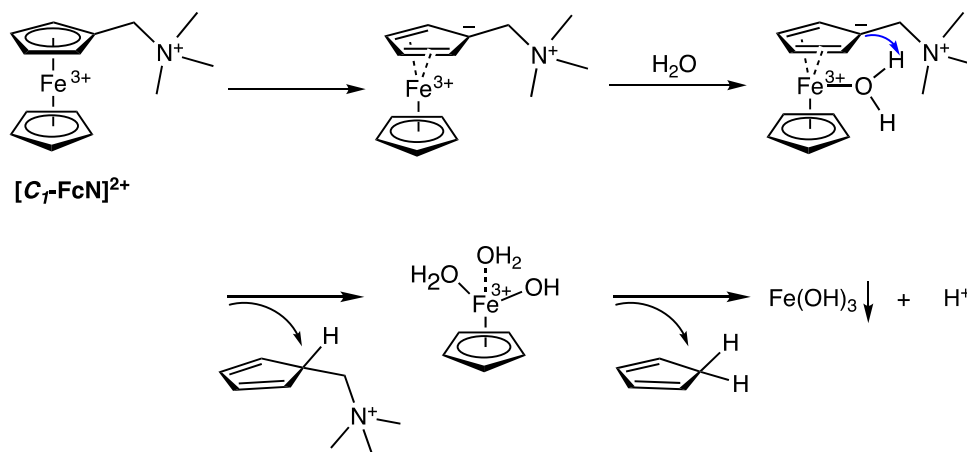
Scheme 1. Proposed thermal degradation mechanism of [C_1-FcN]^{2+} , the charged state of C 1 -FcNCl.
