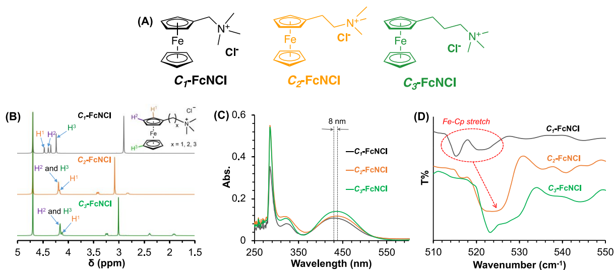
Figure 1. Spectroscopic studies of the Fc derivatives, C_1 -FcNCl (black), C_2 -FcNCl (orange), C_3 -FcNCl (green). (A) Structures of the Fc derivatives; (B) ^1\text{H} -NMR in \text{D}_2\text{O} ; (C) UV-vis absorption; and (D) ATR-IR spectra.
