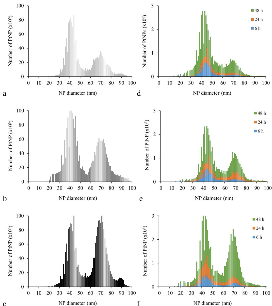
Figure 4. (a-c) Number particle size distribution of and (d-f) the corresponding PtNP accumulation from mixtures of PtNP 40 and PtNP 70 containing: (a) the same mass of PtNP 40 and PtNP 70 ( 25 \mu\text{g L}^{-1} PtNP 40 + 25 \mu\text{g L}^{-1} PtNP 70 ), (b) the same total surface area of PtNP 40 and PtNP 70 ( 25 \mu\text{g L}^{-1} PtNP 40 + 64.25 \mu\text{g L}^{-1} PtNP 70 ), and (c) the same total number of PtNP 40 and PtNP 70 ( 25 \mu\text{g L}^{-1} PtNP 40 + 98.25 \mu\text{g L}^{-1} PtNP 70 ). All measurement were performed by SP-ICP-MS.
