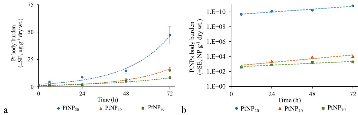
Figure 2. Platinum influx into Leptocierious plumulosus soft tissues after waterborne exposure to 25 \mu\text{g L}^{-1} PtNP 20 , PtNP 40 , and PtNP 70 for 72 h. PtNPs are presented as (a) platinum mass influx ( \mu\text{g g}^{-1} ) and (b) PtNPs number influx ( \text{NP g}^{-1} ). All measurement were performed by SP-ICP-MS. Data points represent mean and standard errors.
