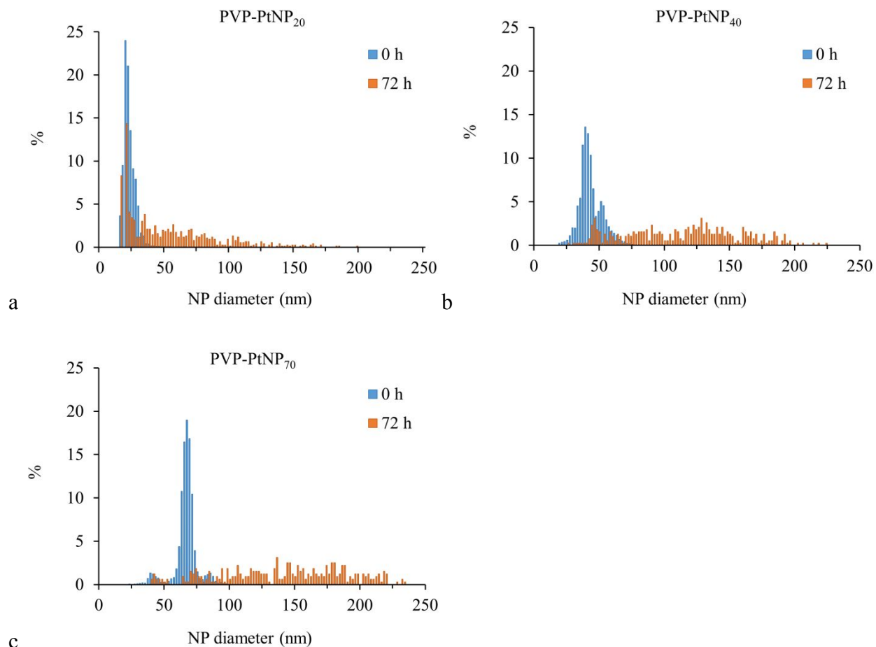
Figure 1. Number particle size distribution of PVP-PtNPs at 0 and 72 h post mixing of 25 \mu\text{g L}^{-1} PtNPs with 15 ppt synthetic seawater without amphipods for (a) PtNP 20 , (b) PtNP 40 , and (c) PtNP 70 . All measurement were performed by SP-ICP-MS.
