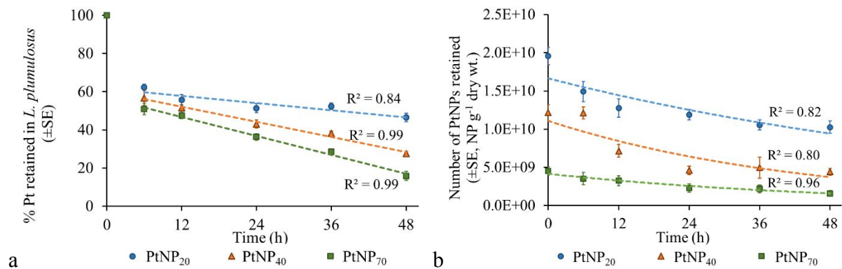
Figure 3. Retention of accumulated Pt in L. plumulosus after 24 h waterborne exposure to 100 \mu\text{g L}^{-1} PtNP 20 , PtNP 40 , and PtNP 70 presented as (a) mass based retention of Pt, and (b) NP number based retention of Pt ( \text{NP g}^{-1} ). All measurement were performed by SP-ICP-MS. Data points represent mean and standard errors.
