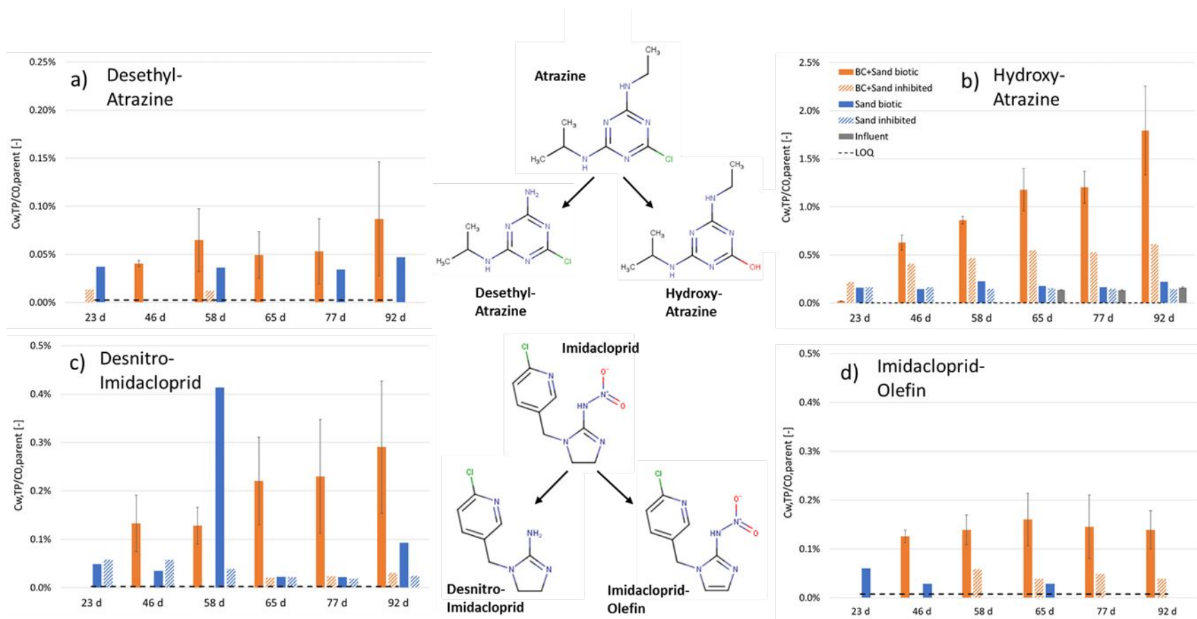
Figure 4: Temporal evolution of transformation products (TPs) of atrazine and imidacloprid in column effluents and influent identified by target LC-QToF-MS analysis: a) desethyl-atrazine, b) 2-hydroxy-atrazine, c) desnitro-imidacloprid, d) imidacloprid-olefin. Y-axis shows TP concentrations in effluent normalized by the average parent influent concentration ( C_{w,TP}/C_{0,parent} ). Dotted black lines represent the limit of quantitation (LOQ) for each TP.
