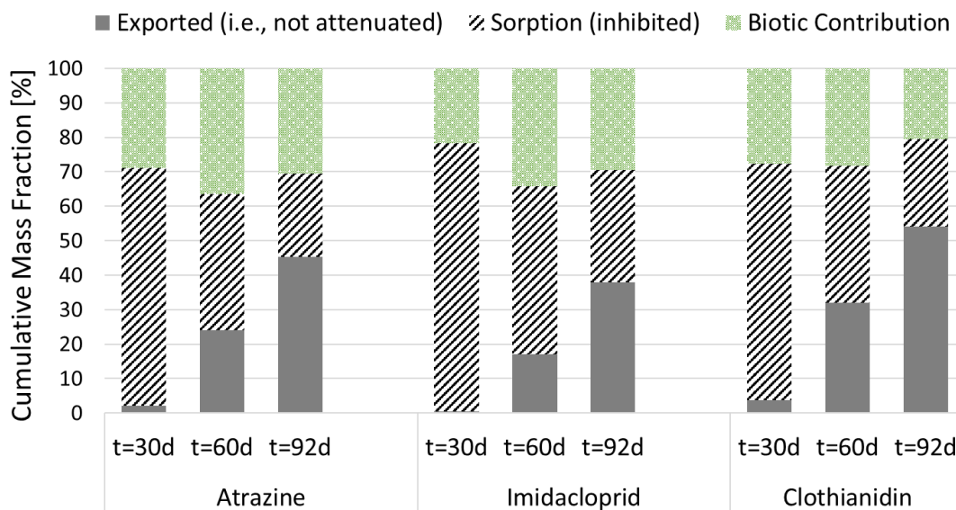
Figure 3: Mass balance of parent effluent data (area under curve calculation). The share of sorption, inhibited (comprising both sorption to the biochar and biosorption) was estimated from the difference between the inhibited Sand and inhibited BC+Sand breakthrough curves. This portion was then subtracted from the biologically enhanced removal observed in the biotic BC+Sand columns to yield the biotic contribution (consisting of both biologically enhanced sorption and biodegradation).
