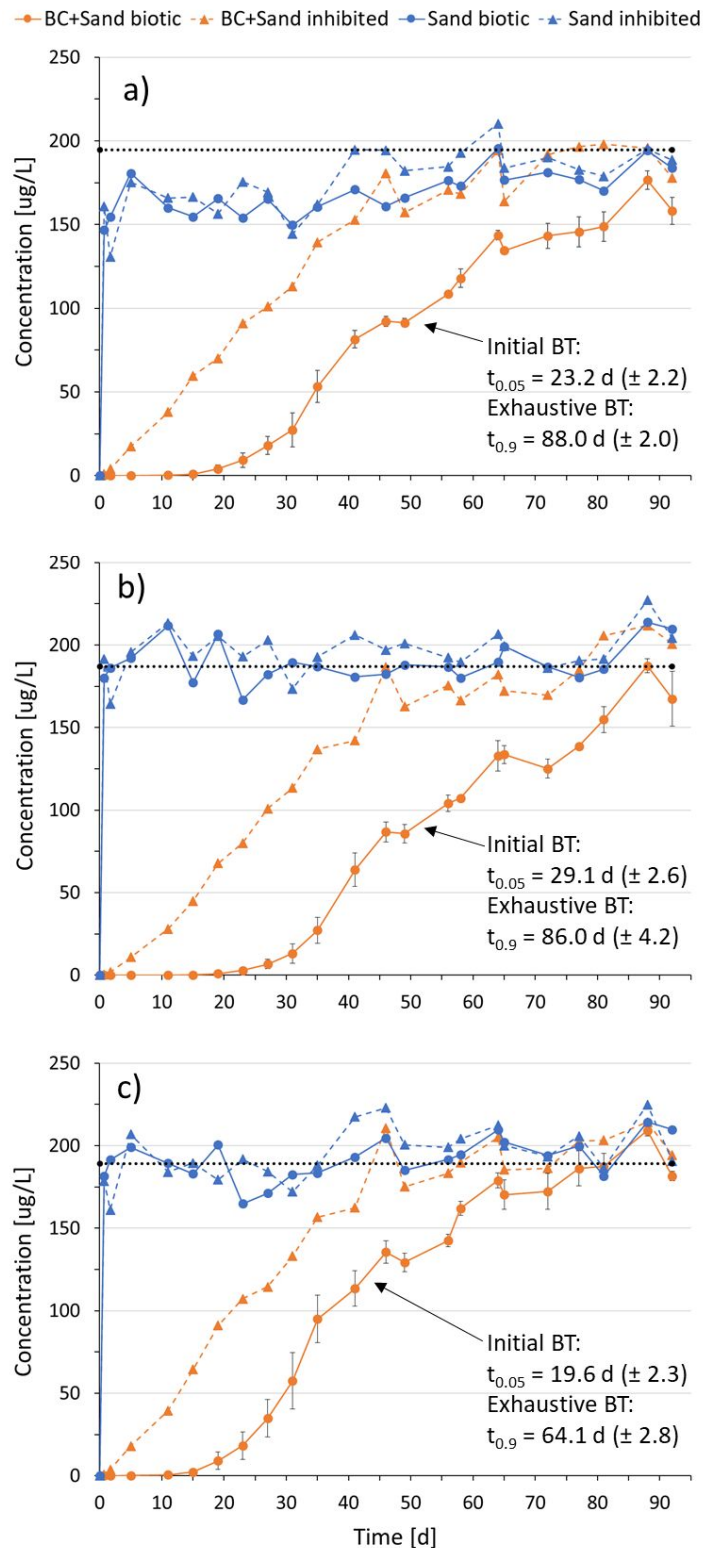
Figure 2: Column effluent concentrations [ \mu\text{g/L} ] over time [days] for the spiked pesticides: a) Atrazine, b) Imidacloprid, c) Clothianidin. Initial breakthrough (BT) is defined as the time when the effluent concentration C_w = 0.05 \cdot C_{\text{influent}} , and exhaustive BT is defined as the time when the effluent concentration C_w = 0.9 \cdot C_{\text{influent}} . BT times for the 'BC+Sand biotic' condition (three replicates) are reported as mean \pm standard deviation. Dotted lines represent the mean influent concentrations.
