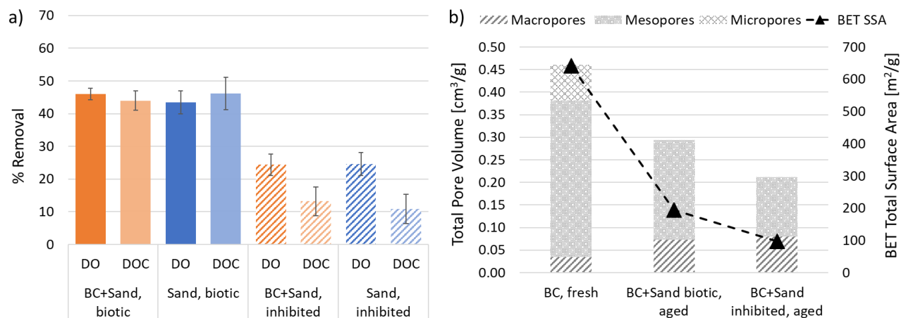
Figure 1: a) Biological activity of columns: Removal of dissolved oxygen (DO) during days 7-110 and removal of dissolved organic carbon (DOC) during days 11-103; shown are the mean and standard error of the mean (SEM) with sample sizes n = 54, 18, 18, 18 , respectively. b) Effect of biofilm and ageing on biochar properties: Brunauer-Emmett-Teller specific surface area (BET SSA) and pore volume distribution of fresh MCG-biochar compared to aged biotic and inhibited samples. Ageing consisted of column conditioning with synthetic stormwater containing \sim 10 mg/L DOC (23 days) followed by injection of synthetic stormwater with \sim 10 mg/L DOC and \sim 200 \mu g/L TOCs (92 days).
