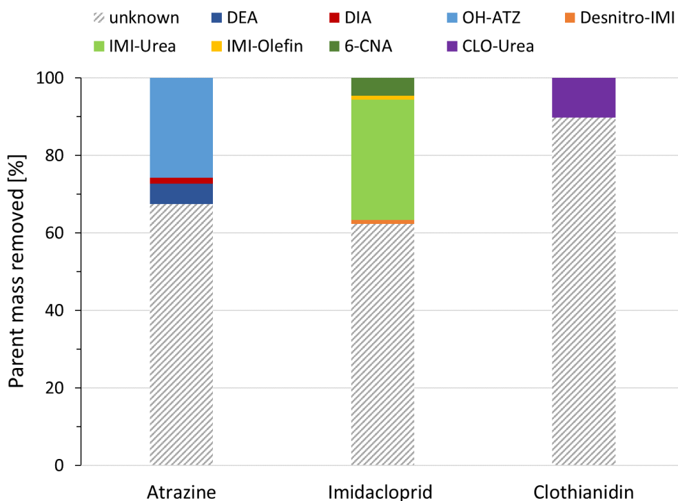
Figure 5: Molar mass balance of microcosm data: Share of transformation products in total parent mass removal at the end of the experiment (369 days). The total parent molar masses removed after 369 days were 71.4 nmol, 119.2 nmol, and 67.8 nmol for atrazine, imidacloprid, and clothianidin, respectively. Initial concentrations for the three compounds were 1923 nM, 1412 nM, and 1458 nM, respectively. "Unknown" indicates that the mass was unaccounted for. Abbreviations: desethyl-atrazine (DEA), desisopropyl-atrazine (DIA), and 2-hydroxy-atrazine (OH-ATZ), desnitro-imidacloprid (desnitro-IMI), imidacloprid-urea (IMI-
