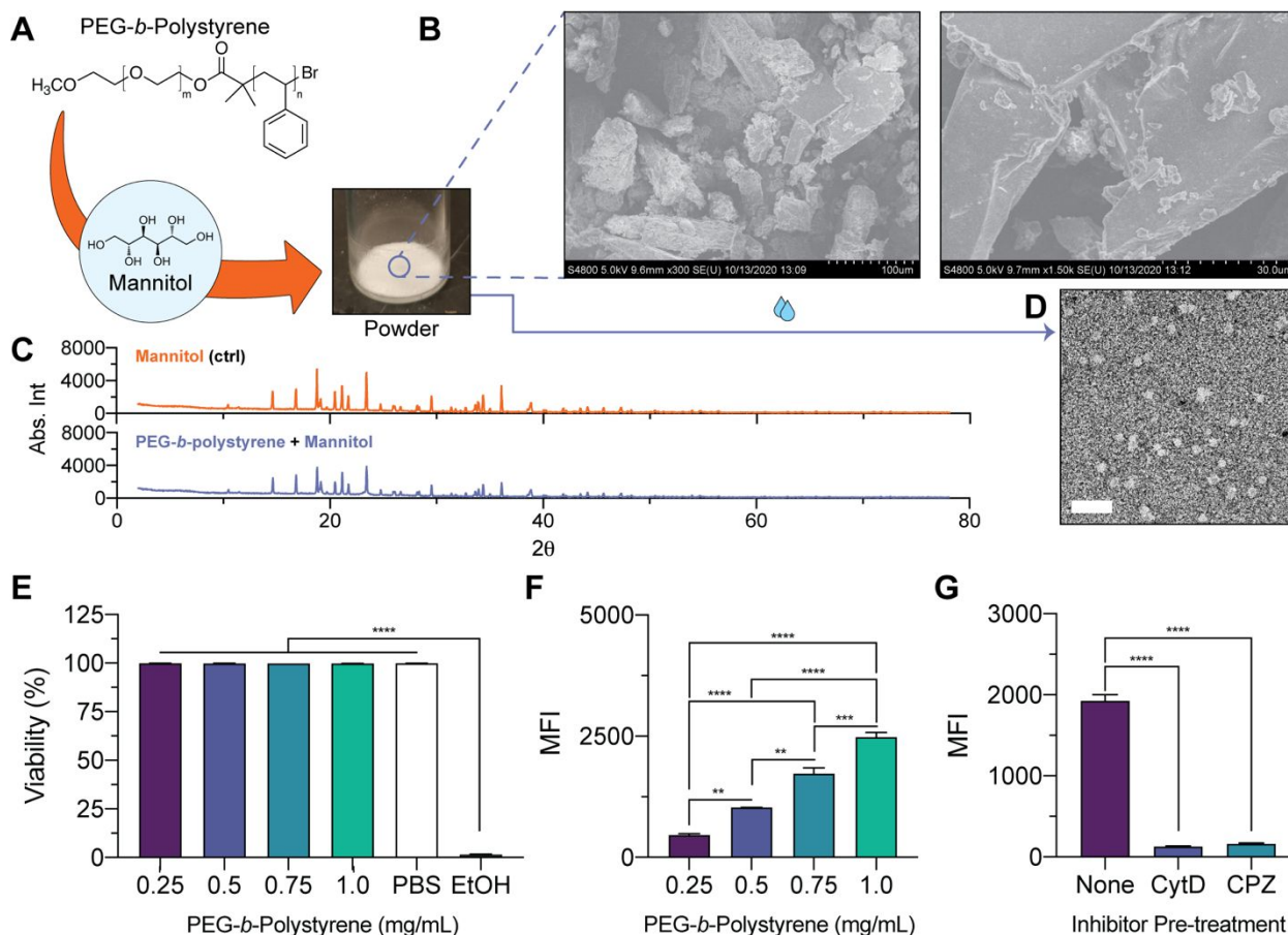
Figure 6. Powdered formulations of a commercially available polymer amphiphile and characterization of resulting nanocarriers that self-assemble upon hydration. (A) Illustration and image of powder formed from mannitol and commercially available PEG- b -polystyrene polymer. (B) SEM micrographs of powders (left = 300X magnification; right = 1500X magnification). (C) Powder XRD of mannitol (control; top) and mannitol coated with PEG- b -polystyrene (bottom). (D) TEM micrograph of hydrated PEG- b -polystyrene micelles (30,000X magnification; Scale bar = 200 nm). (E-G) Cellular viability and uptake studies performed with PEG- b -polystyrene nanocarriers and RAW 264.7 macrophages. (E) Viability of macrophages after 2 h treatment with PEG- b -polystyrene nanocarriers dosed at the specified polymer concentration. PBS- or 70% ethanol (EtOH)-treated cells were included as controls. Significant differences in cell viability versus the EtOH-treated cells were determined by ANOVA with Dunnett's multiple comparisons test and a 5% significance level. (F) Median fluorescence intensity (MFI) of macrophages treated with PEG- b -polystyrene nanocarriers (0.25–1.0 mg/mL polymer concentration) for 2 h. (G) Cellular MFI after pre-treatment with CytD (50 mM) or CPZ (50 mM) endocytosis inhibitors prior to nanocarrier administration. For (F, G), significant differences in cellular uptake were determined by ANOVA with Tukey's multiple comparisons test and a 5% significance level. The mean \pm s.e.m. (n=3) is displayed in E-G.
