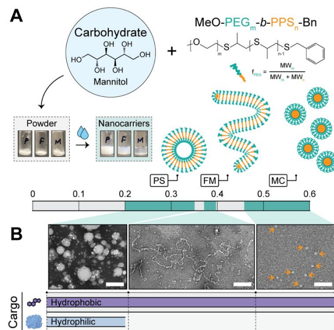
Figure 1. Formation of morphologically diverse nanocarriers upon hydration. (A) Schematic of formulation strategy and illustrative depiction of the resulting PEG- b -PPS nanocarrier morphologies. Powders consisting of PEG- b -PPS polymer and mannitol carbohydrate are prepared. Upon adding water and vortexing, the nanocarriers rapidly self-assemble into the expected morphology based on the hydrophilic (PEG) weight fraction ( f_{PEG} ) range of the polymer. Abbreviations: polymersome (PS); filomicelle (FM); micelle (MC). (B) Transmission electron microscopy (TEM) of negatively stained hydrated nanocarriers (30,000X; scale bar = 200 nm). Orange arrows point to MC. The theoretical cargo loading compatibility is depicted below each micrograph and is experimentally demonstrated later in this manuscript.
