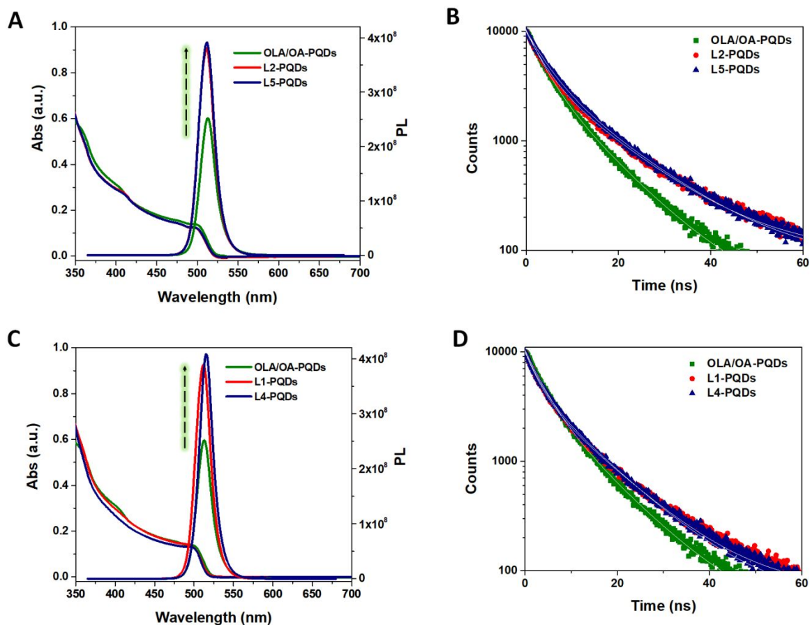
Figure 3: (A) Absorption and fluorescence spectra of OLA/OA–PQDs in hexane along with AMB-PIMA-ODA (L2)–PQDs and IMB-PIMA-ODA (L5)–PQDs dispersed in EtOH. (B) The time-resolved PL decay profiles of the three sets of PQDs shown in A. (C) Absorption and fluorescence spectra collected from dispersions of OLA/OA–PQDs in hexane, L1–PQDs and L4–PQDs dispersed in toluene. (D) The time-resolved PL decay profiles of the three sets of PQDs shown in C.
