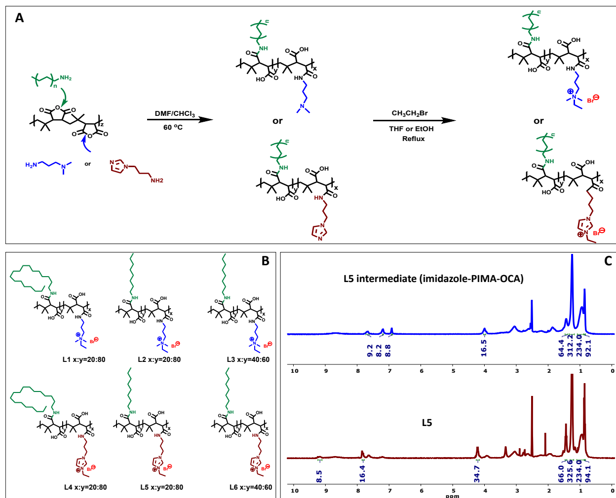
Figure 1: (A) Schematic representation of the nucleophilic addition reaction used to prepare the polysalt ligands. (B) Structures and nomenclature of the ligands prepared and tested in this study. (C) 1 H NMR spectra collected from imidazole-PIMA-OCA (intermediate, top) and the corresponding imidazolium-PIMA-OCA polysalt L5 (bottom). Both compounds were dissolved in DMSO-d 6 .
