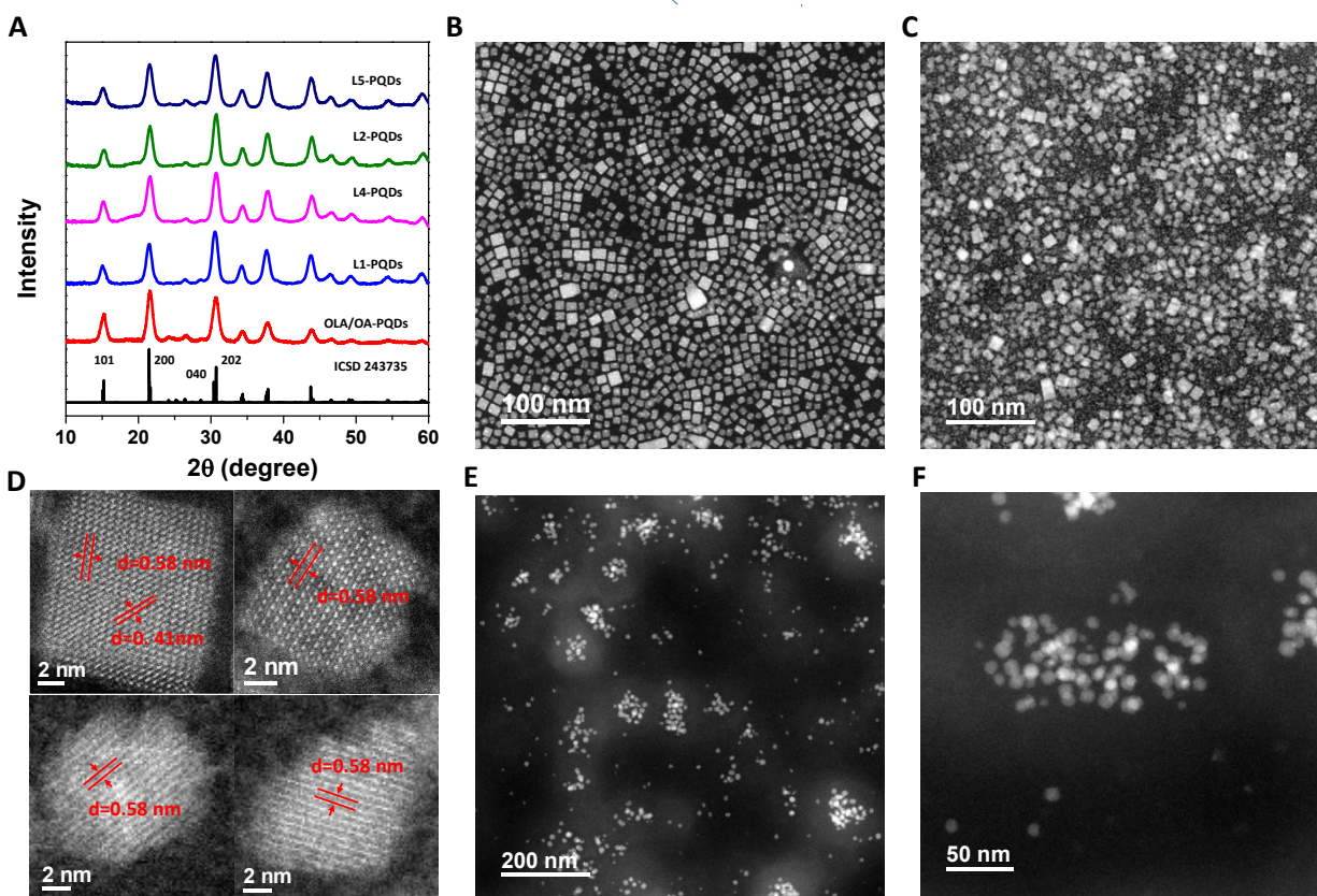
Figure 4: (A) Powder XRD patterns of the native PQDs along with nanocrystals ligand exchanged with various polysalts. (B,C) HAADF-STEM images of OLA/OA-PQDs and AMB20%-PIMA-OCA-PQDs ( L2 ). (D) Representative high resolution TEM images of single perovskite nanocrystals acquired from: OLA/OA-PQDs (top left); L2 (AMB20%-PIMA-OCA)-PQDs (top right); L5 (IMB20%-PIMA-OCA)-PQDs (bottom left and bottom right). (E,F) Lower magnification HAADF-STEM images of L5 (IMB20%-PIMA-OCA)-PQDs. All polysalt-coated PQDs have been aged in EtOH for ~3 months prior to TEM measurements.
