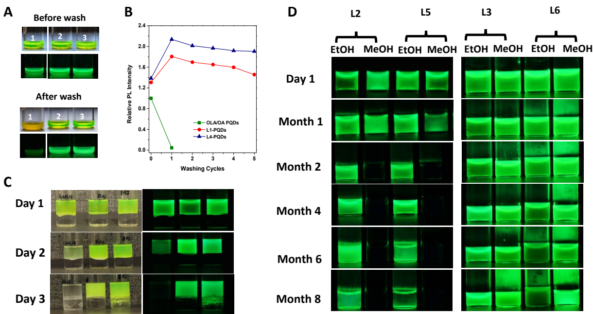
Figure 5: (A) White light and fluorescence images acquired from dispersions of the native PQDs (1) before and after one EtOH wash, along with dispersions of L1-PQDs (2) and L4-PQDs (3), before and after 5 rounds of EtOH wash. (B) Plot of the relative PL intensity measured for pristine OLA/OA-PQDs, or L1-PQDs and L4-PQDs subjected to different EtOH wash cycles. (C) White light and fluorescence images acquired from OLA/OA-, L1- and L4-PQDs taken during the water resistance test; top layer is toluene and bottom layer is DI water. (D) Fluorescence images of AAB-PIMA-OCA (L2 and L3)- and IAB-PIMA-OCA (L5 and L6)-PQDs dispersions in EtOH and MeOH tracked during storage for 8-months.
