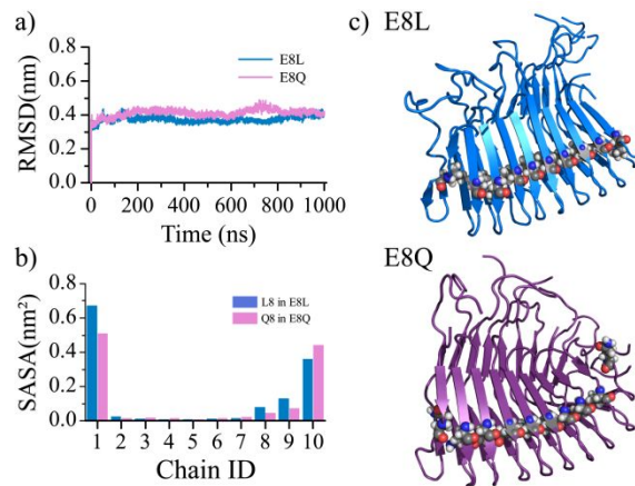
Fig. 5. The structural stability analysis of E8Q and E8L \beta -endorphin mutant fibrils. a) The time evolution of backbone RMSD of two mutant fibrils. For each type of mutant fibrils, a 1000-ns MD simulation was performed. b) The average solvent accessible surface area (SASA) of residue Q8 and L8 in the last 200 ns of corresponding simulations. c) The final structures of the mutant fibrils in MD simulations. Gln8 and Leu8 in each chain are shown in spheres.
