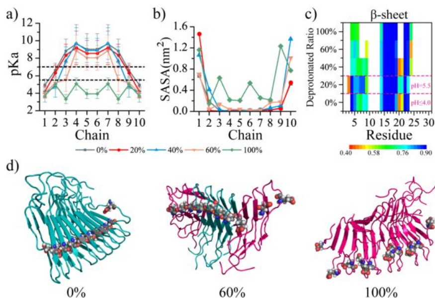
Fig. 4. The conformational analysis caused by progressive deprotonation of Glu8. a) The pKa of Glu8 in each chain predicted using equilibrated conformations in simulations with increasing deprotonation. b) The average solvent accessible surface area (SASA) of Glu8 in each chain based on the equilibrated conformations. c) The average \beta -sheet propensity of each residue from \beta -endorphin peptide. d) The representative final structures of \beta -endorphin fibril with the Glu8 deprotonated ratio of 0%, 60%, and 100%. Glu8 residues are shown in spheres.
