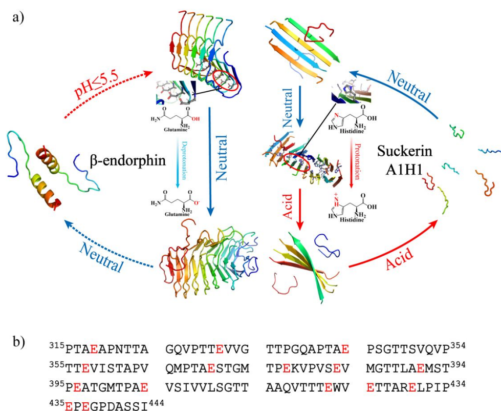
Fig. 6. The schematic diagram illustrates that burying ionizable amino acids as a common strategy to render pH-responsive reversible fibrils for functional amyloids. a) One example is the \beta -endorphin fibrils containing a buried glutamate, which is stable at low pH but disaggregate in neutral pH. The other example is suckerin A1H1 peptide with histidines buried in the core, which could self-assemble into fibrils under neutral pH but disaggregate in the acidic environment 40 . b) The amino acid sequences of Pmel17 repeats, also forming pH-responsive functional amyloids. The ionizable glutamates are highlighted in red.
