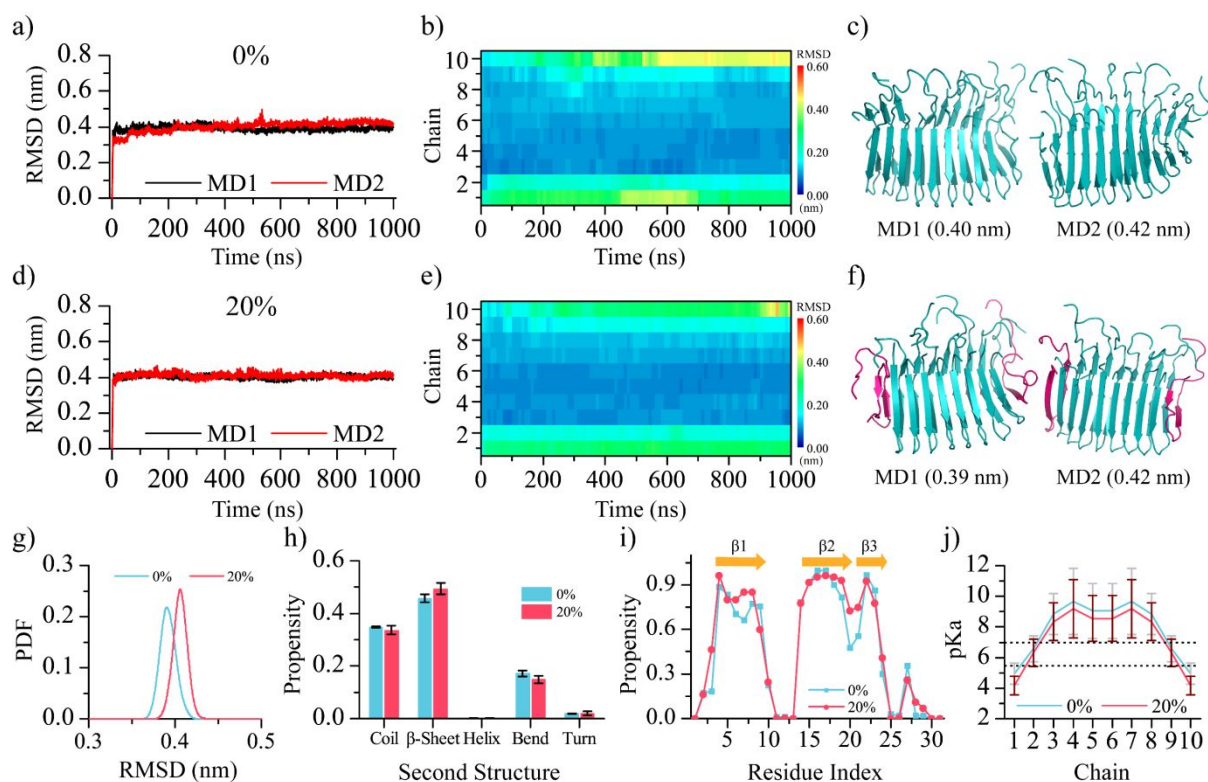
Fig. 2 The structural stability analysis of \beta -endorphin fibrils under acid environment. a) The time evolution of the backbone RMSD of the whole fibril, (b) the backbone RMSD of each chain in the fibril, and (c) the final structures in each of the two independent simulations are presented for the \beta -endorphin with all Glu8 residues protonated (noted as 0% deprotonation). Each independent MD simulation lasted 1000 ns. (d-f) The same results are shown for simulations with two Glu8 residues in the outer layer chains deprotonated (denoted as 20% deprotonation). Chains with Glu8 deprotonated were colored in pink. (g) The probability density distribution as a function of RMSD. Only structures in the last 200 ns simulations were used for the analysis. (h) The average propensities of each secondary structure (including random coil, \beta -sheet, helix, bend and turn) and (i) the probability of each residue to form \beta -sheet in each simulated system. (j) The averaged pKa prediction for Glu8 residues in each chain based on conformation ensembles sampled in the last 50 ns.
