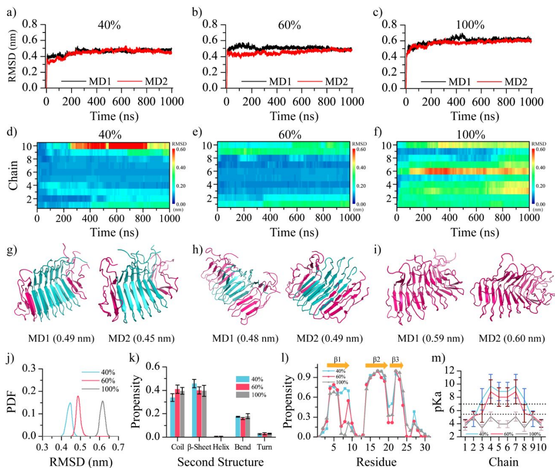
Fig. 3 The structural stability analysis of \beta -endorphin fibrils after switching to neutral pH. a-c) The time evolution of backbone RMSD of the \beta -endorphin fibril with Glu8 residues deprotonated ratio of 40%, 60%, and 100% (denoted as 40%, 60%, and 100%), respectively. For each molecular system, two independent 1000-ns MD simulations were performed. d-f) The backbone RMSD of each chain in the fibril in each simulated system. g-i) The final structures out of each simulation from every system. Chains with corresponding Glu8 deprotonated were colored pink. j) The probability distribution function of backbone RMSD with respect to the initial fibril structure. Only structures from the last 200 ns simulations were used for the analysis. k) The average propensities of each secondary structure (including random coil, \beta -sheet, helix, bend and turn) and (l) the probability of each residue to form \beta -sheet in each simulated system. (m) The averaged pKa prediction for Glu8 residues in each chain based on conformation ensembles sampled in the last 50 ns.
