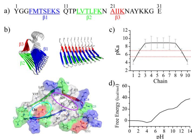
Fig. 1 Experimentally determined \beta -endorphin fibril structure. a) The sequence of \beta -endorphin used in our simulation. Three \beta -strands forming the fibrils are highlighted in blue, green, and red, respectively. b) The reconstructed \beta -endorphin proto-fibril structure comprised of 10 peptides based on prior ssNMR determined fibril structure (PDB ID: 6TUB) is shown in both top and side views. Structural details of a single chain in \beta -endorphin proto-fibril is also shown, highlighting a hydrophobic cluster formed by residues F4, F18, A21, I23, and A26 (indicated by the purple circle); and also a hydrophilic cluster in the core consisted of residues T6, E8, S10, and T16 (the cyan circle). c) The computationally predicted pKa values of Glu8 in each chain based on the experimental structure of the \beta -endorphin fibril. d) The free energy of the \beta -endorphin fibril structure as a function of the pH values.
