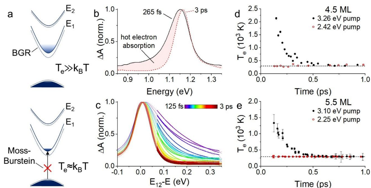
Figure 3. (a) Cartoons of intersubband and interband transitions under conditions of high electron temperature (top) and quasi-equilibrium electron temperature (bottom). BGR stands for band gap renormalization. (b) Spectral line-cuts of transient absorption spectrum of 4.5 ML CQWs photoexcited with 3.26 eV pump photons. (c) Spectral line-cuts of the same sample as a function of time with a normalized energy coordinate ( E_{12}-E ). Thin lines indicate experimental data; thick lines show the region fitted with a Boltzmann distribution. (d, e) Fitted values of T_e for (d) 4.5 ML and (e) 5.5 ML CQW samples under the different pump excitation conditions specified in the caption. The dashed lines in (d) and (e) indicate the ambient temperature of the measurement.
