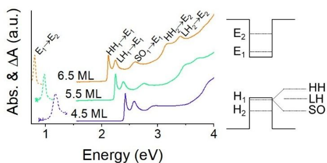
Figure 1. Normalized absorption (solid lines) and photoinduced absorption (dashed lines) of the CdSe CQW samples used in this work. Spectroscopically observed transitions are labelled conventionally according to the energy diagram at right.
