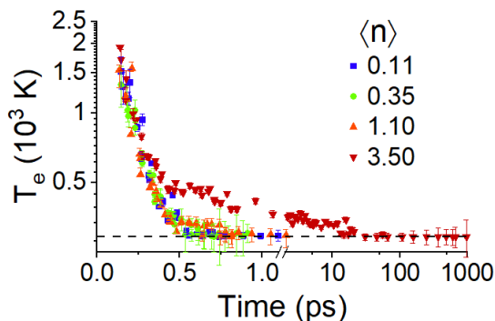
Figure 4. Electron temperature versus time for a 5.5 ML CQW sample excited at 3.10 eV. The figure label indicates the average number of electron-hole pairs generated and the dashed line indicates the ambient temperature.
