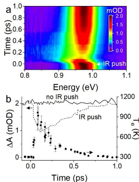
Figure 5. (a) Map of transient absorption of 5.5 ML CQW sample with a 3.10 eV pump excitation followed by a 0.35 eV push excitation of the photoexcited carriers. The time axis is defined with respect to the push-probe delay. (b) Temporal line-cuts of near-infrared absorption with (dashed line) a push pulse and without a push pulse (solid line). Data points show the electron temperature as a function of push-probe delay.
