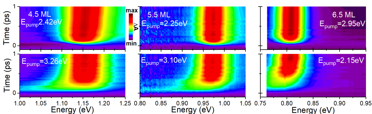
Figure 2. Near-infrared transient absorption data for (top) 4.5 ML, 5.5 ML, and 6.5 ML CdSe CQW samples with resonant excitation of the lowest excitonic absorption. (bottom) The same samples with pump photon energy above the band gap. The fluence was maintained to generate an average of less than 0.3 excitons per particle. XXX
