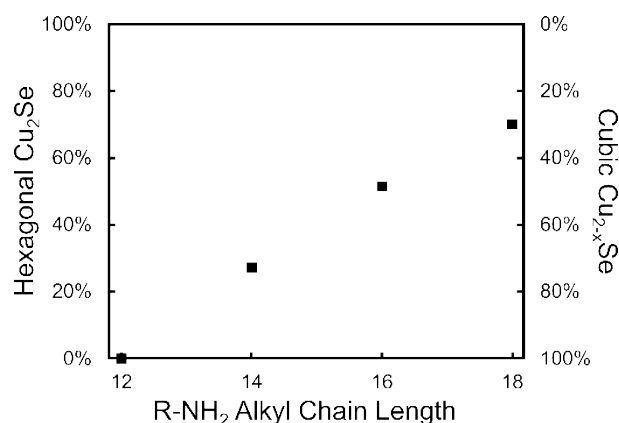
Figure 3 Fractions of nanocrystalline product phases for saturated amines of increasing length. Percentages determined by Rietveld refinement with \chi^2 < 3 .
