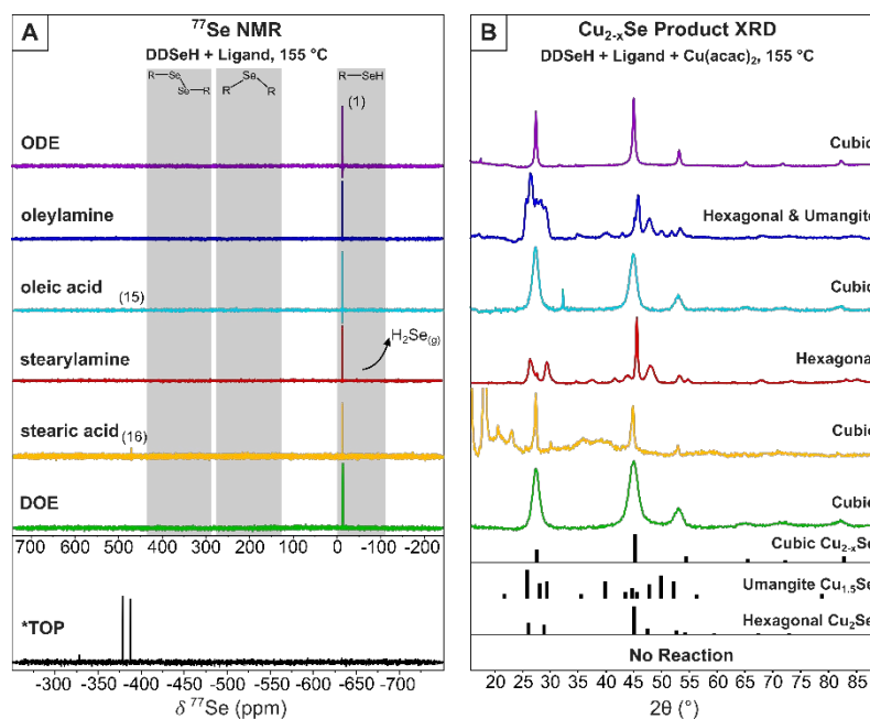
Figure 1 (A) ^{77}\text{Se} NMR of reaction mixture between \text{DDSeH} and various ligands at 155^\circ\text{C} . Major products are listed numerically and match Scheme 1. \text{H}_2\text{Se} evolution was detected qualitatively using \text{Pb}(\text{OAc})_2 strips. *TOP reacts at room temperature with \text{DDSeH} and was not heated. ODE, oleylamine, stearylamine, DOE, and TOP in \text{CDCl}_3 solvent. Oleic acid and stearic acid in \text{C}_6\text{D}_6 (B) XRD of nanocrystalline products when copper precursor was included. Dominant product phases are listed. Complete XRD data for \text{Pb}(\text{OAc})_2 tests are available in Fig. S26. Hexagonal \text{Cu}_2\text{Se} reference pattern from Manna, et al. , 19 cubic (ICSD: 181661), umangite (ICSD: 16949).
