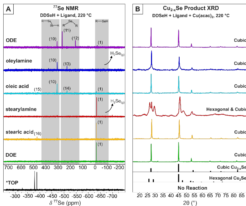
Figure 2 (A) ^{77}\text{Se} NMR of reaction mixture between \text{DDSeH} and various ligands at 220^\circ\text{C} . Major products are listed numerically and match Scheme 1. \text{H}_2\text{Se} evolution was detected qualitatively using \text{Pb}(\text{OAc})_2 strips. ODE, oleylamine, stearylamine, DOE, and TOP in \text{CDCl}_3 solvent. OA and SA in \text{C}_6\text{D}_6 . *TOP reacts at room temperature with \text{DDSeH} and was not heated. (B) XRD of nanocrystalline products when copper precursor was included. Dominant product phases are listed. Complete XRD data for \text{Pb}(\text{OAc})_2 tests are available in Fig. S27. Hexagonal \text{Cu}_2\text{Se} reference pattern from Manna, et al., 19 cubic (ICSD: 181661), umangite (ICSD: 16949).
