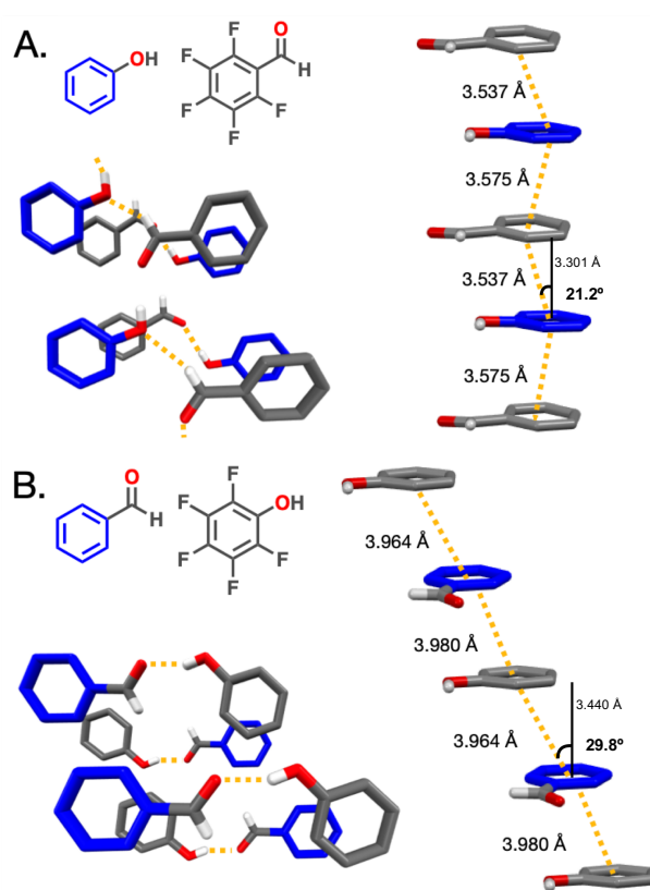
Figure 1. View of each perspective co-crystal along both the aryl:perfluoroaryl stacks and the hydrogen-bonding pattern. Shorter stacking distances and “tape-like” hydrogen-bonding patterns are observed for ArOH:ArFCHO (A) while longer stacking distances and dimer-like hydrogen-bonding patterns are observed for ArCHO:ArFOH (B).
