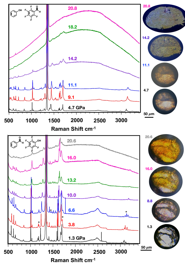
Figure 3. In situ Raman spectroscopy collected during polymerization of ArOH:ArFCHO (top) and ArCHO:ArFOH (bottom), with respective images during polymerization featured to the right. For the ArCHO:ArFOH, bands featuring the onset of the suspected phase transition at 3.8 GPa, continuing to 6.6 GPa are highlighted by an asterisk (*).
