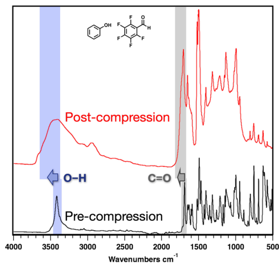
Figure 5. IR spectrum of precursor ArOH:ArFCHO co-crystal prior to compression (black, bottom) and polymer after compression (top, red), featuring the shift to higher wavenumbers of both the –OH and C=O stretching.
