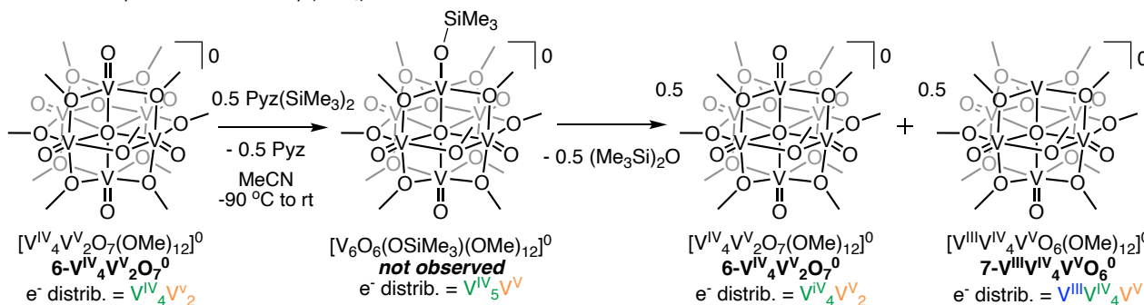
Scheme 3. Reactivity of 6-V^{IV}_4V^{VO}_2O_7^0 with Pyz(SiMe_3)_2 .
