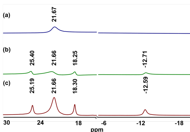
Fig. 5 ^1\text{H-NMR} (500 MHz, \text{CD}_3\text{CN} , 21 ^\circ\text{C} ) spectrum of (a) 6\text{-V}^{\text{IV}}_4\text{V}^{\text{V}}_2\text{O}_7^0 , (b) the crude reaction mixture following the addition of 0.5 equiv of \text{Pyz}(\text{SiMe}_3)_2 to 6\text{-V}^{\text{IV}}_4\text{V}^{\text{V}}_2\text{O}_7^0 in acetonitrile and (c) oxidation of 3\text{-V}^{\text{IV}}_6\text{O}_6(\text{OSiMe}_3)^1 with \text{AgOTf} in dichloromethane. Resonances located at 25.4, 18.3, -12.7 ppm correspond to 7\text{-V}^{\text{III}}\text{V}^{\text{IV}}_4\text{V}^{\text{V}}\text{O}_6^0 and the signal at 21.7 corresponds to 6\text{-V}^{\text{IV}}_4\text{V}^{\text{V}}_2\text{O}_7^0 .
