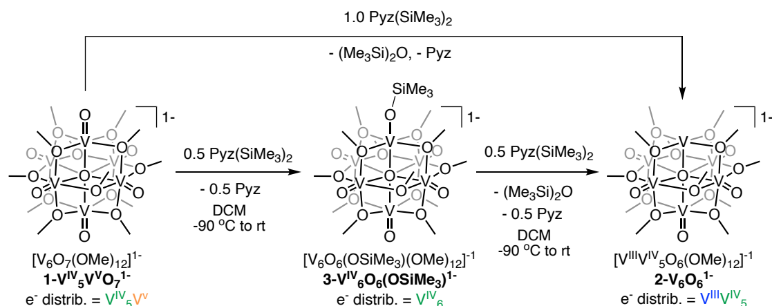
Scheme 1. Reactivity of 1-V IV 5 V V O 7 -1 with various equiv of Pyz(SiMe 3 ) 2 .
