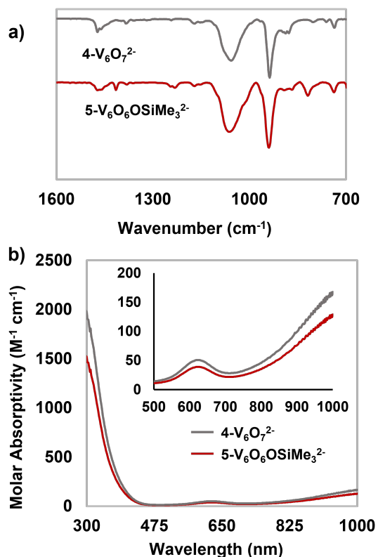
Fig. 3 Spectroscopic characterization of 4\text{-V}^{\text{IV}}_6\text{O}_7^{2-} and 5\text{-V}^{\text{III}}\text{V}^{\text{IV}}_5\text{O}_6(\text{OSiMe}_3)^{2-} : (a) IR spectrum; (b) electronic absorption spectrum collected in acetonitrile at 21 °C. The inset shows the low-energy region of the spectrum to more clearly illustrate IVCT bands.
