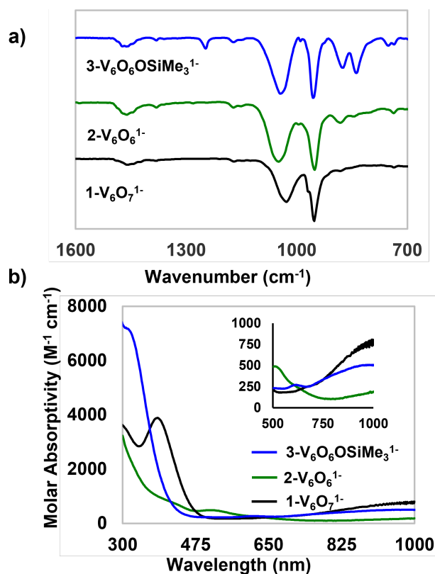
Fig. 2 Spectroscopic characterization of 1\text{-V}^{\text{IV}}_5\text{V}^{\text{VO}}_7^{1-} , 2\text{-V}^{\text{III}}\text{V}^{\text{IV}}_5\text{O}_6^{1-} , and 3\text{-V}^{\text{IV}}_6\text{O}_6(\text{OSiMe}_3)^{1-} : (a) IR spectrum; (b) electronic absorption spectrum collected in acetonitrile at 21°C. The inset shows the low-energy region of the spectrum to more clearly illustrate IVCT bands.
