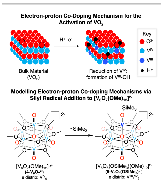
Fig. 4 Analogies between proton-electron co-doping mechanisms reported for VO_2 62-63 and silyl radical transfer to the surface of 4-V^{IV}_6O_7^{2-} .
