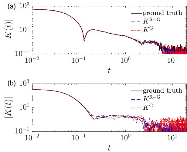
Fig. 6 Star polymer: the memory kernels K(t) predicted at (a) \mu_1^* = \gamma_1^* = 0.4 (interpolation) and (b) \mu_2^* = \gamma_2^* = 0.8 (extrapolation) by the ROM-GPR ( K^{\text{R-G}} ) and GPR ( K^{\text{G}} ) transfer learning methods, respectively, compared with the memory kernels computed from the MD simulation data (ground truth). Here, \gamma is the concentration of star polymers; the same training parameter instances \mathcal{P}_{\text{tr}}^{\text{active}} were used for both methods.
