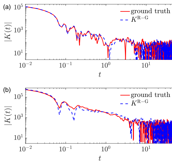
Fig. 15 Peptoid polymer: the memory kernels K^{R-G}(t) predicted by the ROM-GPR transfer learning method at (a) \mu_1^* = (307, 1) (interpolation), corresponding to T = 307 K and z = 1 and (b) \mu_2^* = (365, 6) (extrapolation), corresponding to T = 365 K and z = 6 , compared with the memory kernels directly computed from the MD simulation data (ground truth).
