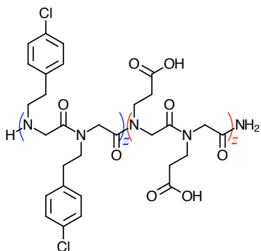
Fig. 13 Chemical structure of a peptoid polymer. z denotes the number of repeat units: N_{4-Cl}pe and Nce .
