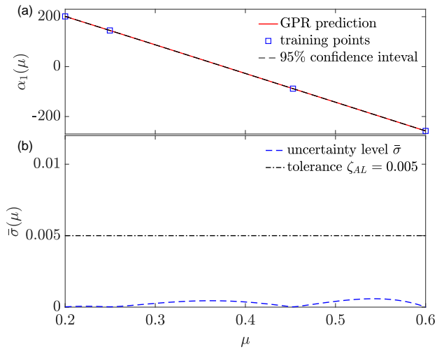
Fig. 4 The third step of active learning process: (a) GPR model for the POD parameter mode \alpha_1(\mu) inferred from 4 training data, where the fourth training data is obtained from Fig. 3. (b) Uncertainty quantified by \bar{\sigma}(\mu) of the inferred GPR model. Here, the active learning process is terminated since the maximum of uncertainty level is smaller than the preset tolerance.
