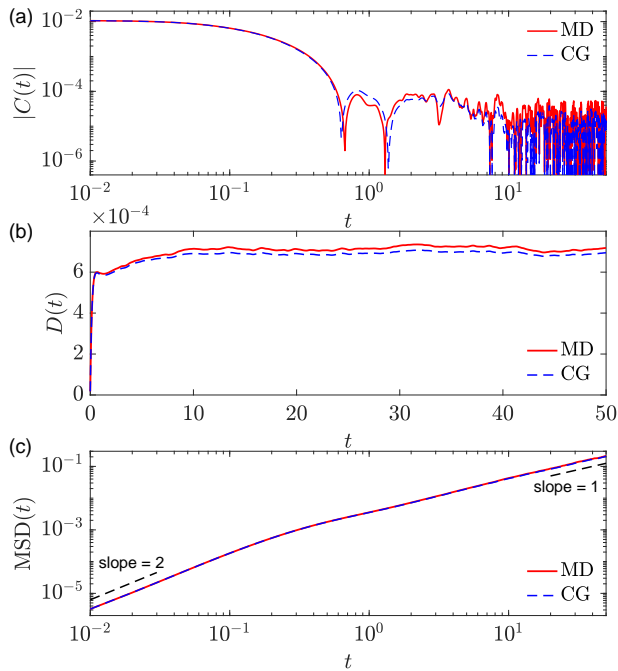
Fig. 16 VACF ( C(t) ), diffusion coefficient ( D(t) ), and MSD predicted by the CG model at T=307 K for the peptoid polymer with one N_{4-Clpe} and Nce, compared with the MD simulation results. Here, to construct the CG model, K^{R-G}(t; \mu_1^*) in Fig. 15 (a) was approximated by Eq. (7) with \mathcal{N} = 7 terms.
