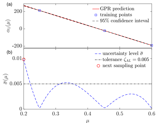
Fig. 3 The second step of active learning process: (a) GPR model for the POD parameter mode \alpha_1(\mu) inferred from 3 training data. Here the third training data is obtained from Fig. 2 (b) Uncertainty quantified by \bar{\sigma}(\mu) of the inferred GPR model and the next sampling point ( \mu_{\text{next}} = 0.2 ) determined by active learning.
