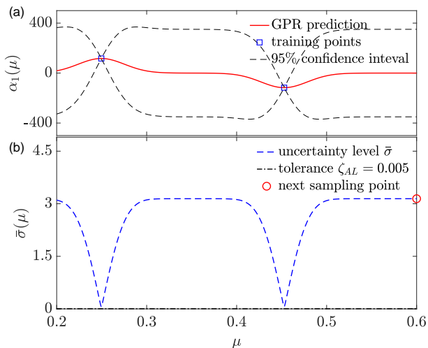
Fig. 2 The first step of active learning process: (a) GPR model for the POD parameter mode \alpha_1(\mu) inferred from 2 randomly initialized training data. (b) Uncertainty quantified by \bar{\sigma}(\mu) of the inferred GPR model and the next sampling point ( \mu_{\text{next}} = 0.6 ) determined by active learning.
