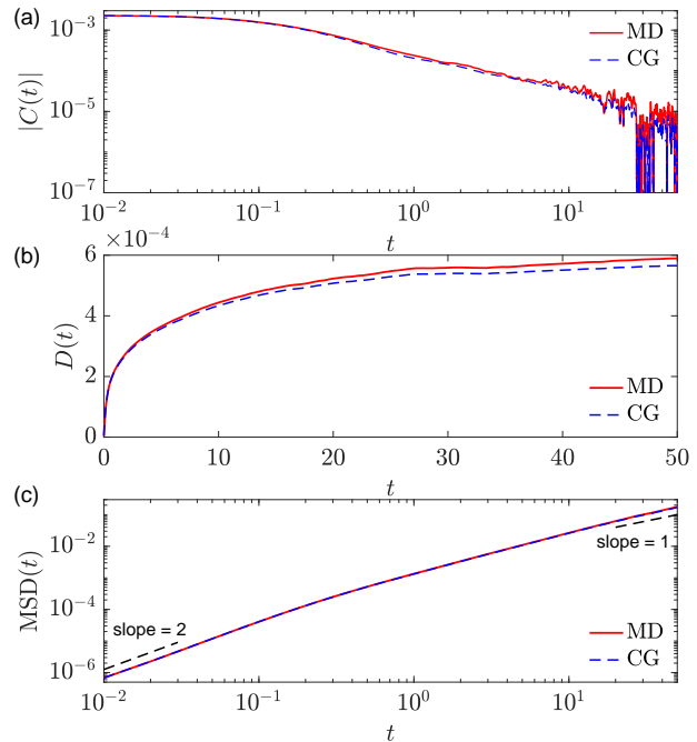
Fig. 17 VACF ( C(t) ), diffusion coefficient ( D(t) ), and MSD predicted by the CG model at T=365 K for the peptoid polymer with 6 N_{4-Clpe} and Nce (outside the training sampling space), compared with the MD simulation results. Here, to construct the CG model, K^{R-G}(t; \mu_2^*) in Fig. 15 (b) was approximated by Eq. (7) with \mathcal{N} = 8 terms.
