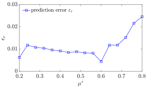
Fig. 5 The relative error \varepsilon_r(\mu^*) of the memory kernels K^{\text{R-G}}(t; \mu^*) predicted by ROM-GPR transfer learning at different testing parameter instances \mu^* \in \mathcal{P}_{\text{test}} .
