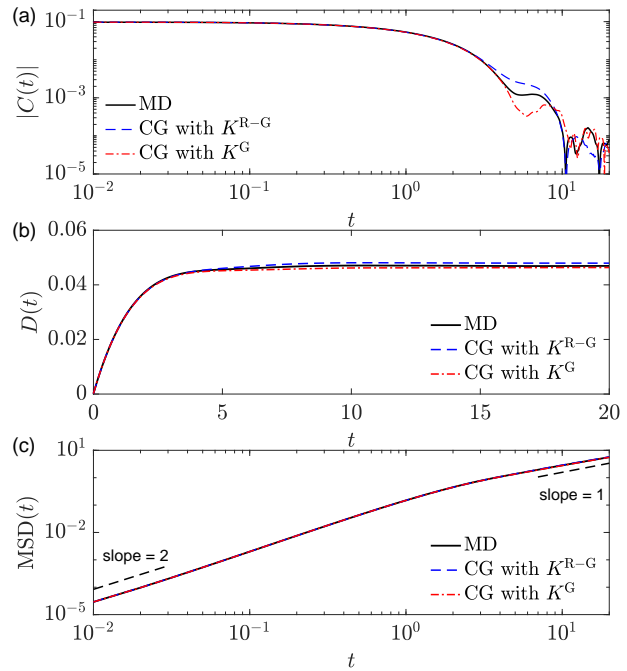
Fig. 8 VACF ( C(t) ), diffusion coefficient ( D(t) ), and MSD of the star polymer predicted by the CG models at \mu_2^* = \gamma_2^* = 0.8 (outside the training sampling space), compared with the MD simulation results. Here, \gamma is the concentration of star polymers; the memory kernel predicted by the ROM-GPR ( K^{R-G} ) or GPR ( K^G ) transfer learning method was approximated by Eq. (7) with \mathcal{N} = 7 terms.
