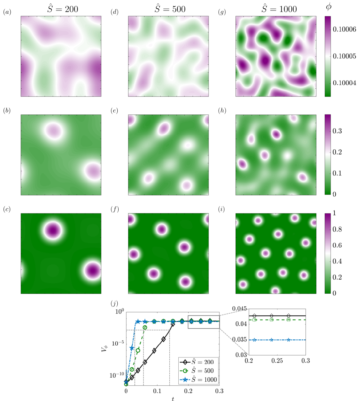
Figure 3: Temporal evolution of the protein distribution in simulations of the Cahn-Hilliard model of Equation 19 on a flat square patch of area 1 \mu\text{m}^2 for \hat{A} = 25 and three different values of \hat{S} . The three rows in panels (a-i) correspond to three distinct times: at an early time t_b = 3 \times 10^{-3} shortly after the start of the simulation, at an intermediate time t_{in} when protein density variance reaches V_\phi = 2 \times 10^{-3} , and at a late time t_s = 0.3 when the system has reached steady state. The three columns correspond to \hat{S} = 200 (a-c), \hat{S} = 500 (d-f), and \hat{S} = 1000 (g-i). Also see Movies M1-M3 in the ESI for the corresponding dynamics. (j) Temporal evolution of the variance V_\phi of the protein density for the same cases shown in (a-i). The dashed lines indicate the intermediate time t_{in} when the variance reaches V_\phi = 2 \times 10^{-3} .
