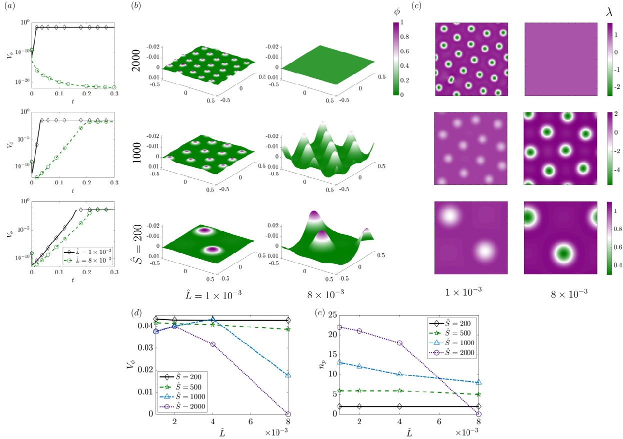
Figure 7: Effect of \hat{S} and \hat{L} on protein aggregation and membrane dynamics. (a) Temporal evolution of the protein density variance V_\phi for two \hat{L} values \hat{L} and the same three values of \hat{S} shown in (b). (b) Distribution of protein density on the deformed membrane at a long time approaching steady state ( t = 0.3 ) for various combinations of \hat{L} and \hat{S} , with \hat{A} = 25 . The corresponding dynamics are also shown in movies M4-M6 of the ESI. (c) Distribution of the local membrane tension for the same cases as in (b). (d) Variance of protein density V_\phi and (e) number of protein patches n_p at t = 0.3 as functions of \hat{L} , for various values of \hat{S} .
