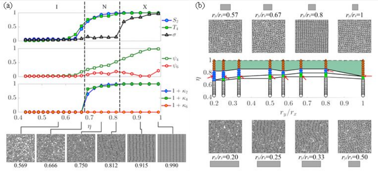
Fig. 7. For rectangles (superellipses with n=\infty ), (a) and for r_y/r_x=0.2 , as a function of area fraction ( \eta ), (top) nematic, S_2 , tetratic, T_4 , and smectic, \sigma , order parameters, (middle) symmetry via stretched four-fold ( \psi_4^s ) and six-fold ( \psi_6^s ) parameters, and (bottom) orientational order correlation function decay values ( \kappa_2 , \kappa_4 , \kappa_6 ). Phases indicated as: (I) isotropic, (N) nematic, or (X) crystal, with symmetry indicated as (4F) four-fold. (b) Phase diagram vs. r_y/r_x and \eta with phases (from Fig. S12) indicated as: (O) isotropic, (A) nematic, (S) tetratic, or (D) crystal, with symmetry indicated as (S) four-fold. Panels show characteristic configurations at (left) indicated particle concentrations, and (right) red arrows.
