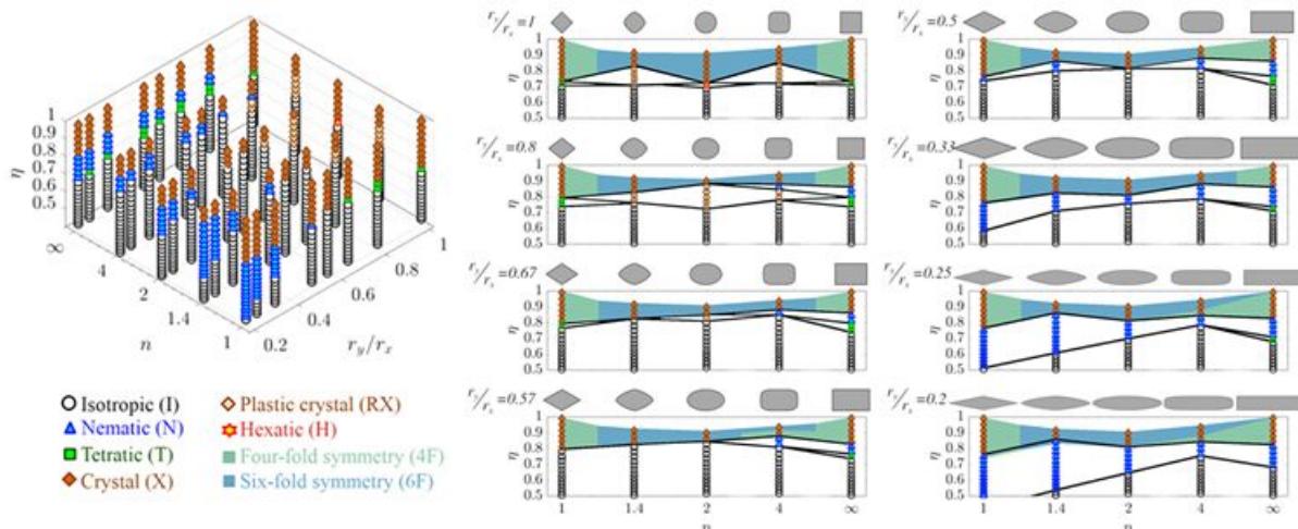
Fig. 8. Phase diagram for hard superellipses as a function of the aspect ratio ( r_y/r_x ), particle shape parameter ( n ), and area fraction ( \eta ). Phases indicated as: (○) isotropic, (△) nematic, (■) tetratic, (◇) plastic crystal, or (◆) crystal, with symmetry indicated as (■) four-fold or (■) six-fold. Hexatic phase (★) from large system size literature results. 11,12
