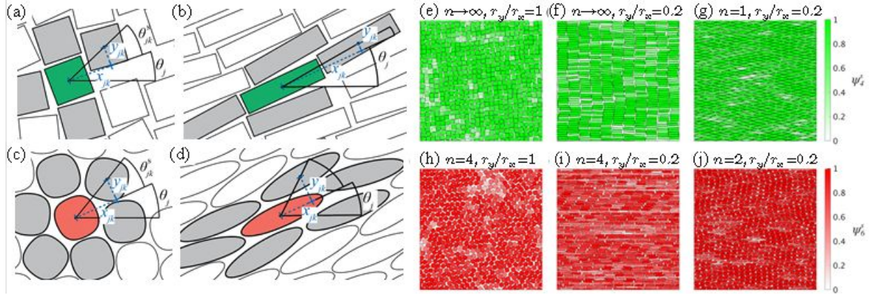
Fig. 2. Neighbor identification and stretched bond orientational order. (left) (top) In the case of \psi_{4,j} , illustration for (a) squares ( n=\infty , r_y/r_x=1 ) and (b) rectangles ( n=\infty , r_y/r_x=0.2 ), around central particle (green) and 4 neighbors (grey) by relative center position x_{jk} and y_{jk} (blue). (bottom) In the case of \psi_{6,j} , illustration for (c) rounded squares ( n=4 , r_y/r_x=1 ) and (d) ellipses ( n=2 , r_y/r_x=0.25 ) around central particle (red). (right) Various particle configurations colored by local stretched bond orientational order parameters (Eq. (4)) for (e-g) 4-fold order and (h-j) 6-fold order with shape parameters labelled on figures.
