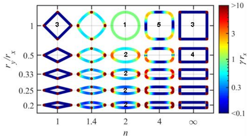
Fig. 1. Superellipse shapes vs. aspect ratio r_y/r_x and the parameter n (Eq. (1)). The outline of each shape is colored to depict the local curvature (Eq. (2)), where corner features can be considered to correspond to \gamma r_x \gtrsim 3 and sidewalls have \gamma r_x \lesssim 0.3 . Previously studied benchmark cases include: (1) disks ( n=2 , r_y/r_x=1 ), 7-12 (2) ellipses ( n=2 , r_y/r_x<1 ), 13,15 (3) squares ( n\rightarrow\infty , r_y/r_x=1 ), 16 (4) rectangles ( n\rightarrow\infty , r_y/r_x<1 ), 17,18 and (5) rounded squares ( n\approx 3-10 , r_y/r_x=1 ). 19,20
