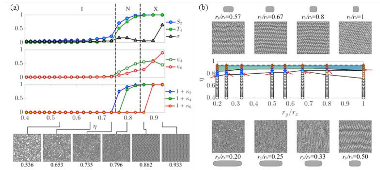
Fig. 6. For rounded rectangles (superellipses with n=4 ), (a) and for r_y/r_x=0.2 , as a function of area fraction ( \eta ), (top) nematic, S_2 , tetratic, T_4 , and smectic, \sigma , order parameters, (middle) symmetry via stretched four-fold ( \psi_4^s ) and six-fold ( \psi_6^s ) parameters, and (bottom) orientational order correlation function decay values ( \kappa_2 , \kappa_4 , \kappa_6 ). Phases indicated as: (I) isotropic, (N) nematic, or (X) crystal, with symmetry indicated as (4F) four-fold. (b) Phase diagram vs. r_y/r_x and \eta with phases (from Fig. S9 ) indicated as: (O) isotropic, ( \Delta ) nematic, ( \diamond ) plastic crystal, or ( \blacklozenge ) crystal, with symmetry indicated as ( \blacksquare ) four-fold or ( \blacksquare ) six-fold. Panels show configurations at (left) indicated particle concentrations, and (right) red arrows.
