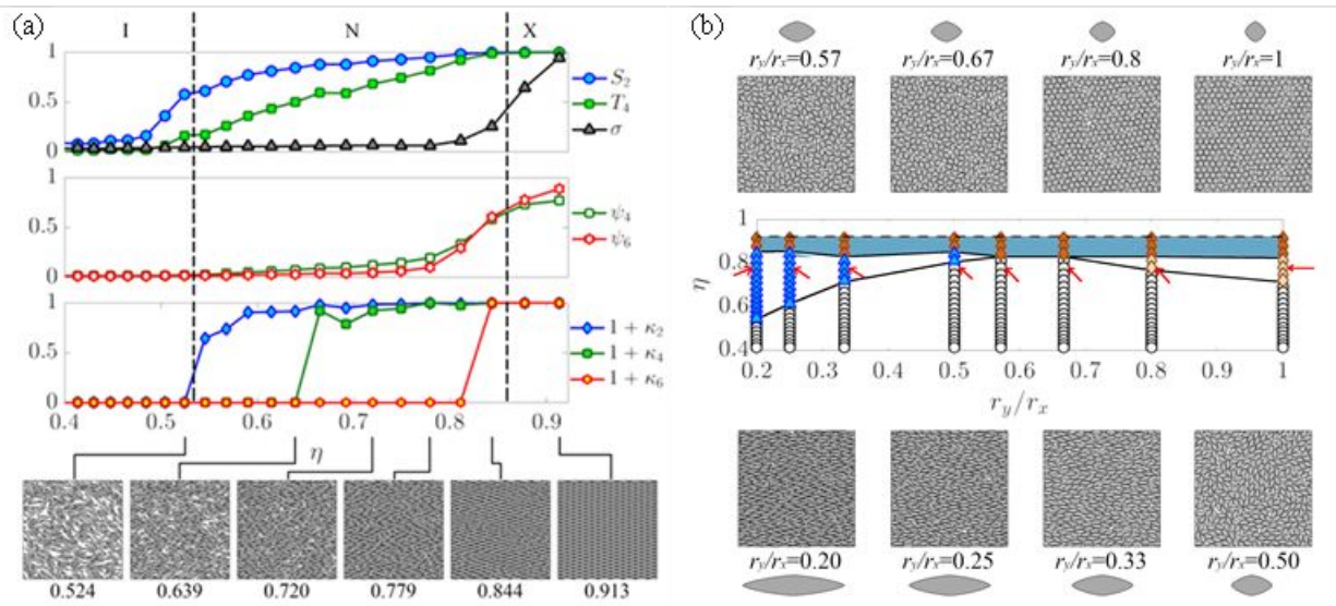
Fig. 4 For rounded rhombuses (superellipses with n=1.4 ), (a) and for r_y/r_x=0.2 , as a function of area fraction ( \eta ), (top) nematic, S_2 , tetatic, T_4 , and smectic, \sigma , order parameters, (middle) symmetry via stretched four-fold ( \psi_4^s ) and six-fold ( \psi_6^s ) parameters, and (bottom) orientational order correlation function decay values ( \kappa_2 , \kappa_4 , \kappa_6 ). Phases indicated as: (I) isotropic, (N) nematic, or (X) crystal, with symmetry indicated as (6F) six-fold. (b) Phase diagram vs. r_y/r_x and \eta with phases (from Fig. S7) indicated as: (O) isotropic, ( \Delta ) nematic, ( \diamond ) plastic crystal, or ( \blacklozenge ) crystal, with symmetry indicated as ( \blacksquare ) six-fold. Panels show characteristic configurations at (left) indicated particle concentrations, and (right) red arrows.
