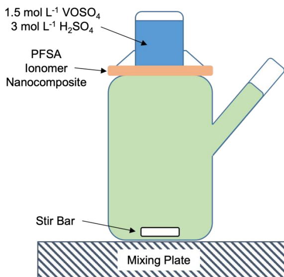
Figure 1. Schematic of the permeation cell used to measure vanadyl ion permeability through the perfluorosulfonic acid (PFSA) ionomer nanocomposites.
