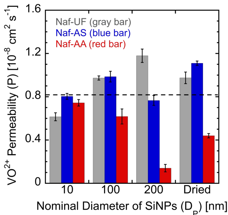
Figure 2. Vanadyl ion ( \text{VO}^{2+} ) permeability for PFSA ionomer nanocomposites containing a mass fraction of 5% SiNPs with varying nominal diameters and surface functionalities. Ionomer membranes containing UF-SiNP, AS-SiNP, and AA-SiNP are shown in solid gray, blue, and red bars, respectively. Error bars represent the standard deviation of the average \text{VO}^{2+} permeability, which was calculated from experiments on at least three separate membranes. The dashed black line represents the average \text{VO}^{2+} permeability for Pristine-Naf. Note, the data shown for membranes containing 10 nm SiNPs have been previously published. 27
