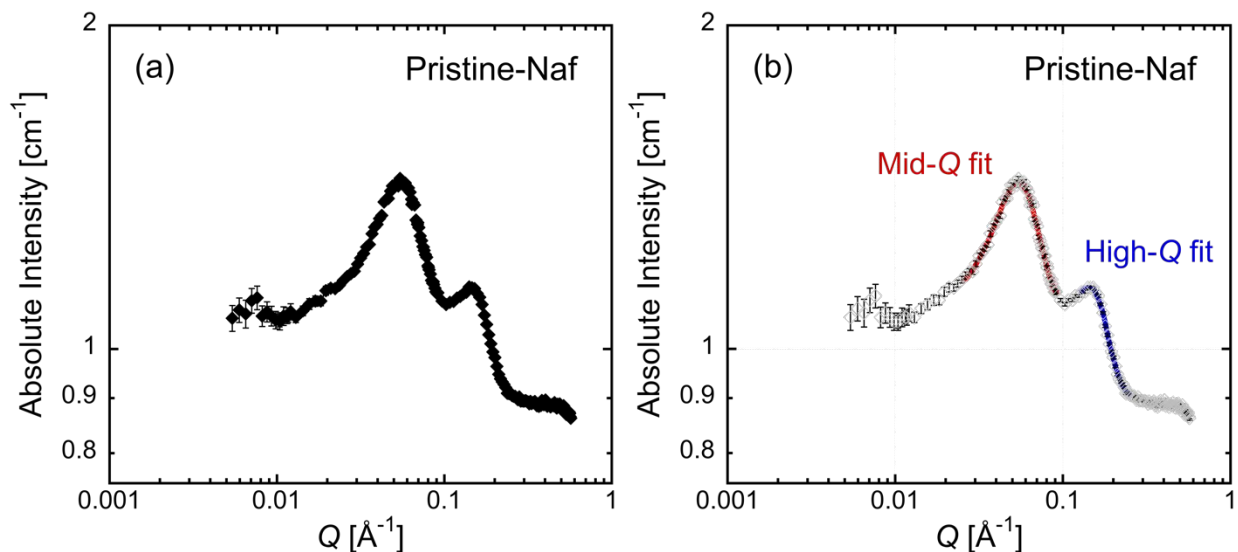
Figure 6. Small-angle neutron scattering (SANS) curve for hydrated pristine Nafion. (b) Gaussian fit of the mid- Q (hydrophobic; solid red line) and high- Q (hydrophilic; solid blue line) peaks of pristine Nafion. All membranes were hydrated in 100% \text{H}_2\text{O} for at least 24 h prior to SANS experiments. The error bars on the SANS data for each membrane represent the standard deviation in calculated intensities. Note, the scattering data shown in (a) and (b) have been previously published. 28
