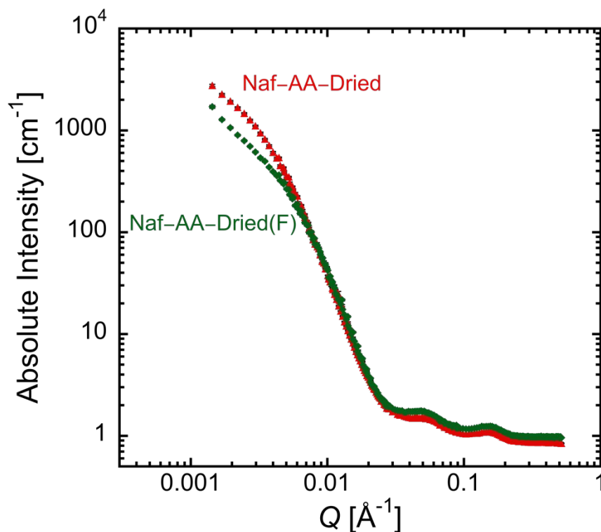
Figure 10. Small-angle neutron scattering (SANS) curves for hydrated Nafion nanocomposites containing a mass fraction of 5 % dried, amine-functionalized SiNPs that were either purchased pre-functionalized (Naf-AA-Dried; red triangles) or functionalized in-house (Naf-AA-Dried(F); green diamonds). Note, all membranes were hydrated in 100 % \text{H}_2\text{O} for at least 24 h prior to SANS experiments. The error bars on the SANS data for each membrane represent the standard deviation in calculated intensities.
