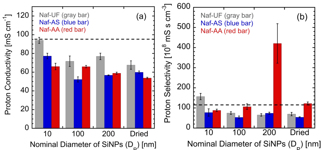
Figure 4. (a) Proton conductivity of Nafion nanocomposites. The dashed black line represents the calculated average proton conductivity of Pristine–Naf. (b) Proton selectivity (i.e., proton conductivity divided by vanadyl ion permeability) of Nafion nanocomposites. The dashed black line represents the calculated average ion selectivity of Pristine–Naf. Error bars in each plot represent the standard deviation of the average value, which was calculated from experiments on at least three separated membranes.
