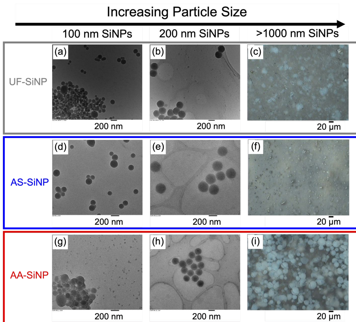
Figure 5. (a, b, d, e, g, h; first two columns) Transmission electron and (c, f, i; far right column) optical microscopy images of PFSA nanocomposite membranes containing a mass fraction of 5% SiNPs with various surface functionalizations. The microscopy images are organized in rows according to their surface chemistry, where top, middle, and bottom rows represent Naf-UF (outlined in gray), Naf-AS (outlined in blue), and Naf-AA membranes (outlined in red), respectively. As seen at the top of the images, the images are organized in columns according to the sizes of the SiNPs, which increase from left to right. Note, the scale bars for all TEM images are 200 nm, while the scale bars for all optical microscopy images are 20 \mu m. The optical microscopy images were obtained with a polarized lens.
