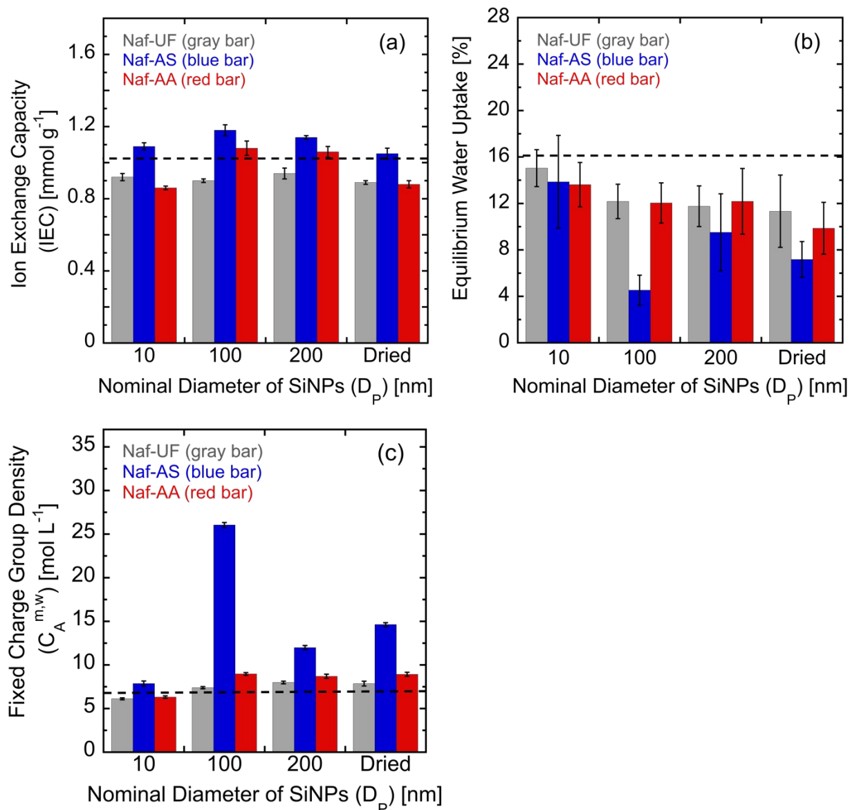
Figure 3. (a) Ion exchange capacity (IEC), (b) equilibrium water uptake, and (c) fixed charge group density for Nafion nanocomposites containing a mass fraction of 5% SiNPs with varying nominal diameters and surface functionalities. Ionomer membranes containing UF-SiNP, AS-SiNP, and AA-SiNP are shown in solid gray, blue, and red bars, respectively. The dashed black lines represents the calculated average IEC and equilibrium water uptake of Pristine-Naf. The error bars in each figure represent the standard deviation of the average value, which was calculated from experiments on at least three separate membranes.
