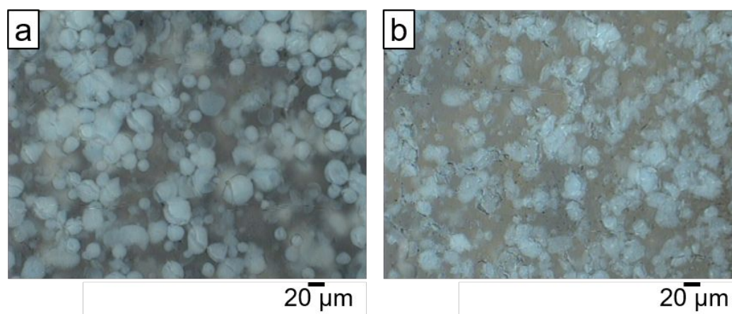
Figure 9. Optical microscopy images of PFSA ionomers containing a mass fraction of 5 % dried, amine-functionalized particles that were (a) purchased pre-functionalized (Naf-AA-Dried) or (b) functionalized in-house (Naf-AA-Dried(F)). Note, the image shown in (a) is identical to the image shown in Figure 4i. It has been included here for direct comparison. The scale bars of all optical microscopy images are 20 \mu\text{m} , and all images were obtained using polarized lens.
