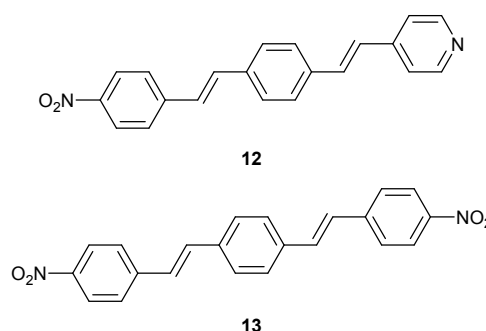
Fig. 8 Structures of nitroaromatics 12 and 13 .
