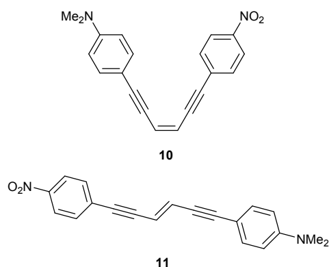
Fig. 5 Structures of the push-pull chromophores 10 and 11 .
