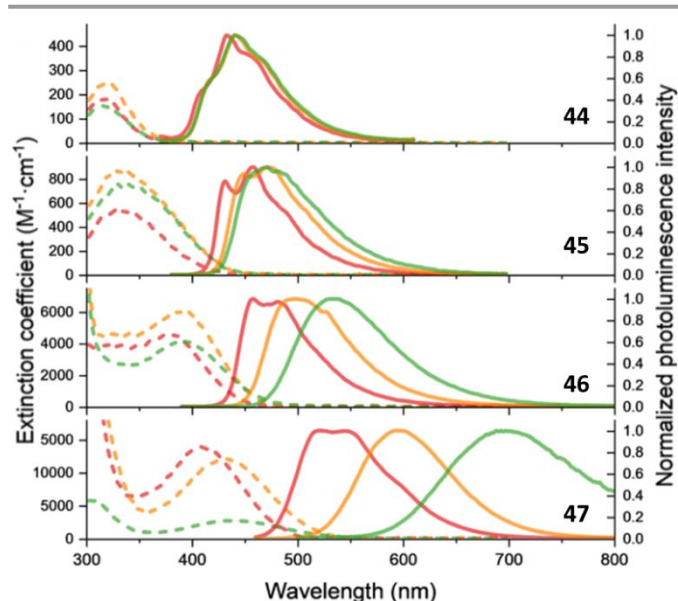
Fig. 19 The absorption (dashed) and the fluorescence (solid) of the phenothiazines 44–47 . Copyright 2020 Wiley. Used with permission from Ref. 25
