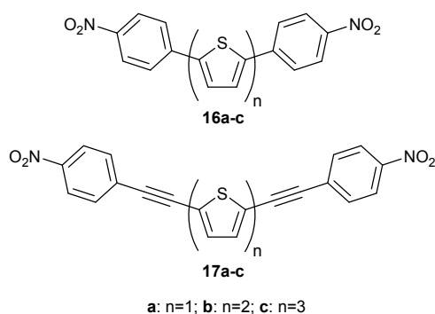
Fig. 11 Structures of dyes 16a-c and 17a-c .
