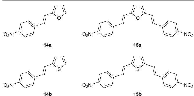
Fig. 10 The structure of heterocyclic analogues of nitrostilbenes 14a,b and 15a,b .
