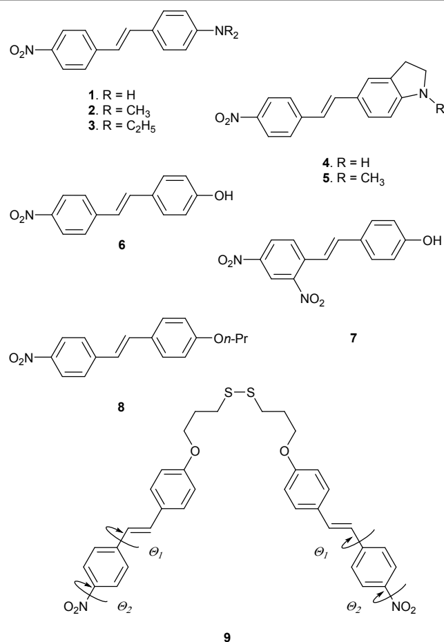
Fig. 2 Structures of nitrostilbenes 1-9 possessing different electron donors
