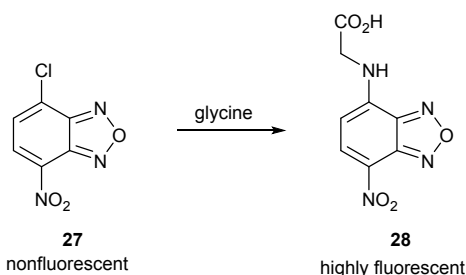
Scheme 1 Transformation of 4-chloro-7-nitrobenzooxadiazole 27 into the fluorescent derivative 28 .
