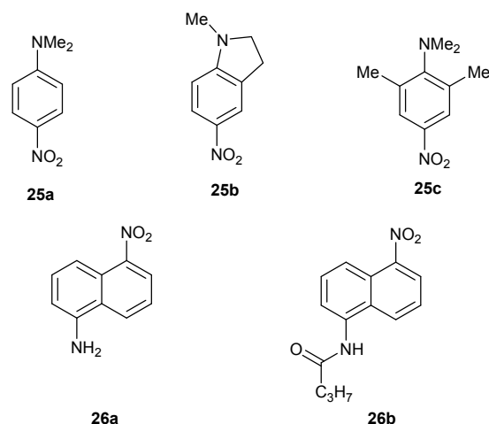
Fig. 15 The structures of nitrobenzenes 25a-c and nitronaphthalenes 26a,b .
