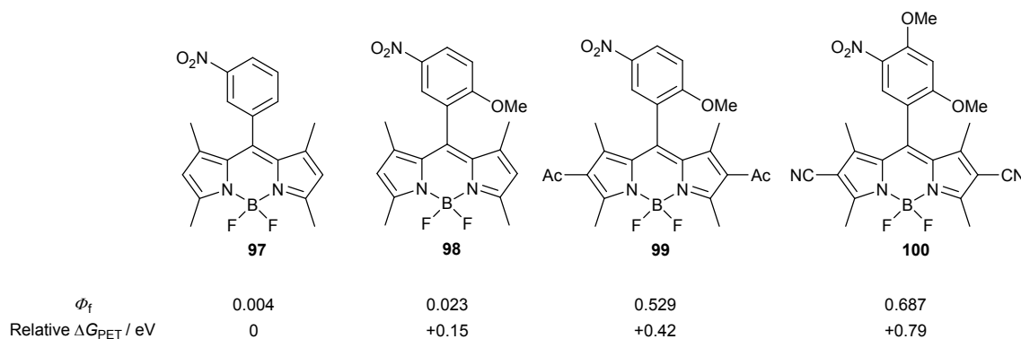
Fig. 32 Structures of 5-(nitrophenyl)BODIPYs 97-100 .
