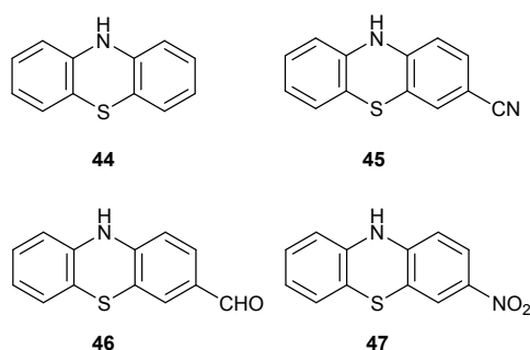
Fig. 18 Structures of phenothiazine derivatives 44–47 .
