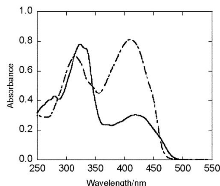
Fig. 6 The absorption spectra of 10 (solid line) and 11 (dot-dash line). Reproduced from Ref. 71
