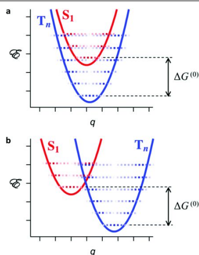
Fig. 1 State diagrams depicting ISC under: (a) weak vibronic coupling, where the nested geometry leads to an overlap between the lowest energy vibrational wavefunction of the S_1 electronic state with the central region of the upper vibrational wavefunctions of the triplet state. (b) Strong vibronic coupling, where vibrational wave functions from the S_1 and T_n electronic states overlap at the crossings of the potential energy surfaces of the electronic states. Reproduced from ref. 18
