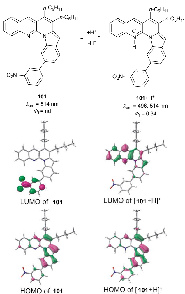
Fig. 33 Chemical structures as well as HOMOs and LUMOs of 101 and its 14-N protonated cation [ 101+H + ]. nd – not determined. Adapted with permission from Ref. 147 Copyright 2014 American Chemical Society.
