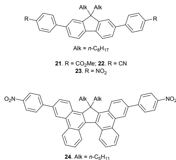
Fig. 13 Structures of dyes 21-24 .
