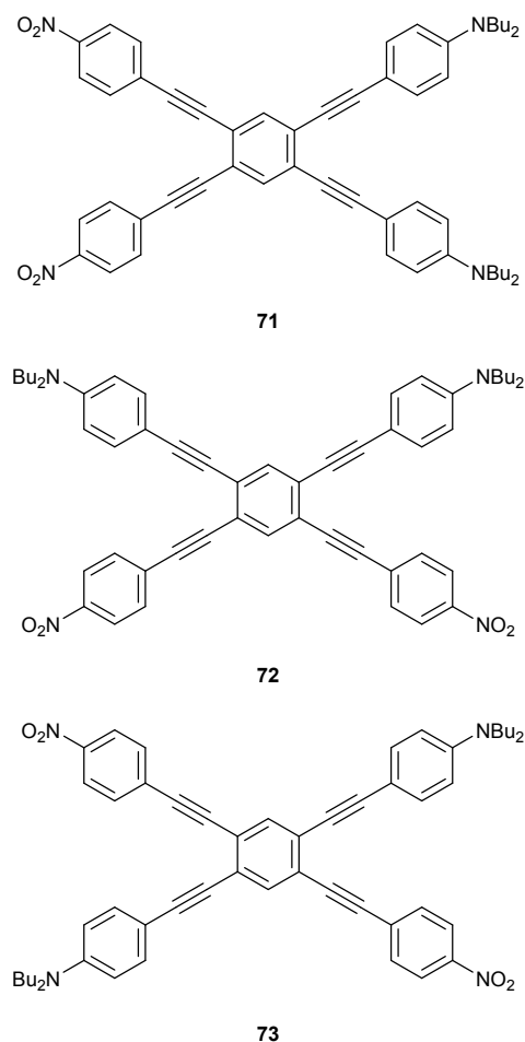
Fig. 24. Structure of cross-shaped chromophores 71-73.
