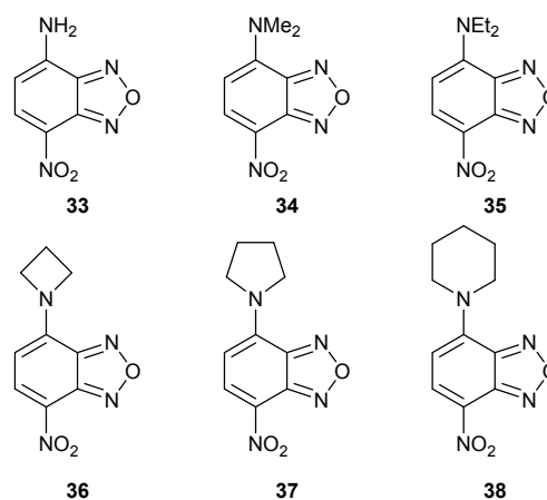
Fig. 17 The structures of nitro-NBDs 33-38 possessing various amino groups.
