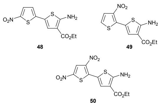
Fig. 20 Structures of nitro-thienylthiophenes 48-50 .
