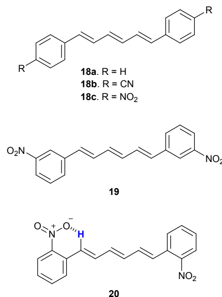
Fig. 12 Structures of dyes 18-20 .
