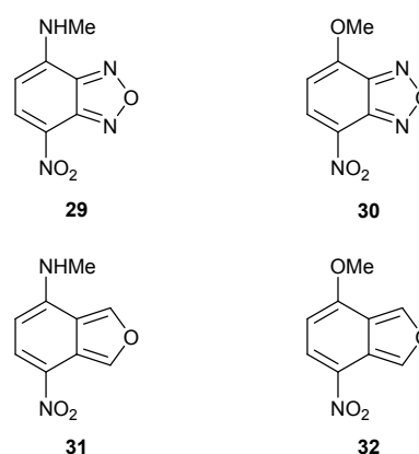
Fig. 16 The structures of nitrobenzo-2-oxa-1,3-diazoles 29 and 30 and the corresponding isobenzofuran derivatives 31 and 32 .
