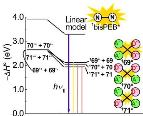
Fig. 23. Energy level diagram for radiolysis induced chemiluminescence of dyes 69-71. Adapted with permission from Ref. 114 Copyright 2007 American Chemical Society.
