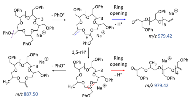
Scheme 2. Homolytic ring-opening of sodiated C_7 ( m/z 1073.47), initiated by \text{PhO}^\bullet loss. Smaller fragment ions are attributed to the ring-opened structures (Schemes 3-4).
