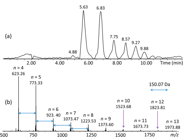
Fig. 2. (a) LC-MS total ion chromatogram (TIC) of pGPE; the LC-MS spectra acquired at 4.88 and 5.63 min are depicted in Fig. S2. (b) Summed ESI-MS spectrum of the TIC. The observed ions correspond to sodiated (C 9 H 10 O 2 ) n oligomers with n = 4–13, this composition is common to the cyclic (C) as well as the tadpole (TP-OH) architecture.
