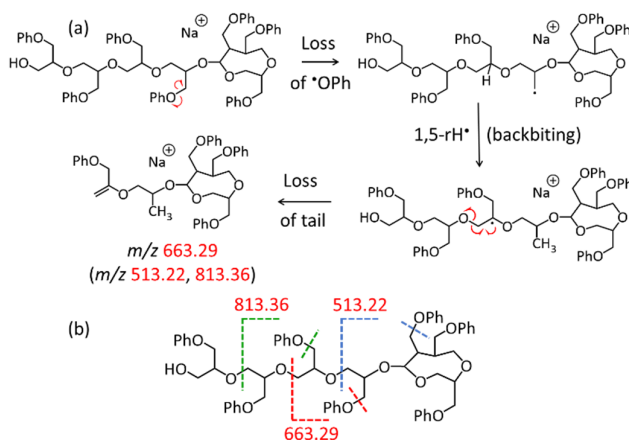
Scheme 1. (a) Fragmentation pathway to the fragment ion series [150n + 40 + \text{Na}]^+ , illustrated for the formation of the fragment at m/z 663.29; (b) similar fragmentation pathways lead to the fragments at m/z 513.22 and 813.36.
