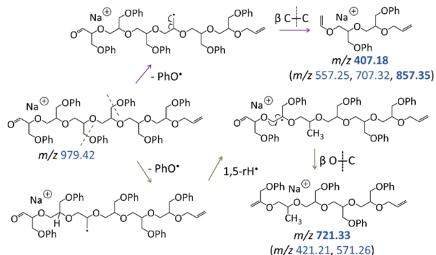
Scheme 4. Dissociation of the ring-opened intermediate with aldehyde and vinyl end groups ( m/z 979.42), leading to m/z 407.18, 721.33, and analogous fragments with the 150-Da repeat unit (i.e., series [150n + 84 + \text{Na}]^+ and [150n + 98 + \text{Na}]^+ , respectively). The m/z values of intense ions are indicated in boldface.
