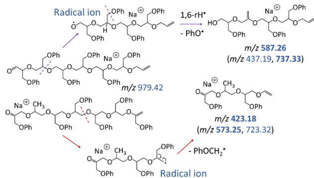
Scheme 3. Dissociation of the ring-opened intermediates with aldehyde and vinyl or keto and vinyl end groups (both at m/z 979.42), leading to the fragments at m/z 587.26 and 423.18, respectively. Fragments with the same substituents, i.e. series [150n + 114 + \text{Na}]^+ and [150n + 100 + \text{Na}]^+ , respectively, arise through analogous bond cleavages; their m/z values are given in parenthesis, with intense ions indicated in boldface.
