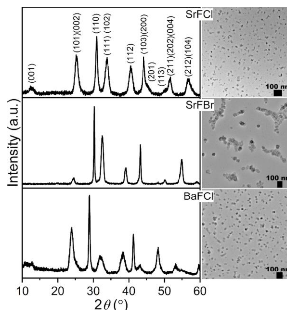
Figure 1. Indexed PXRD patterns and TEM images of SrFCl, SrFBr, and BaFCl nanocrystals codoped with \text{Yb}^{3+} and \text{Er}^{3+} .
