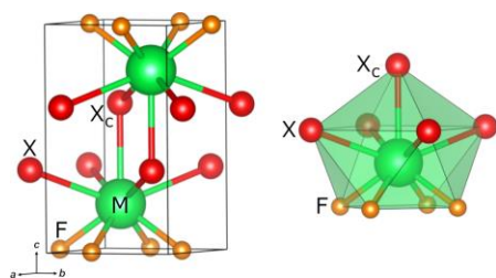
Figure 2. Unit cell of MF x (left) and view of the first coordination shell of M 2+ as an MF 4 X 5 polyhedron (right).
