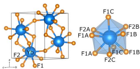
Figure 4. Unit cell of \text{YbF}_3 (left) and view of the first coordination shell of \text{Yb}^{3+} as an \text{YbF}_9 polyhedron (right).
