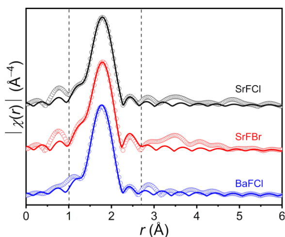
Figure 7. Fits of an YbO_4F_3 cluster to the radial structure functions of Yb:Er:SrFX and Yb:Er:BaFCl nanocrystals. Experimental (hollow circles) and calculated functions (solid lines) are shown. \chi(r) functions were fit in the 1.0–2.7 Å r range (depicted with vertical dashed lines).
