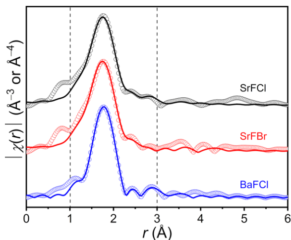
Figure 3. Fits of an YbF 4 X 5 monometallic cluster to the radial structure functions of Yb:Er:SrFX and Yb:Er:BaFCl nanocrystals. Experimental (hollow circles) and calculated functions (solid lines) are shown. \chi(r) functions were fit in the 1.0–3.0 Å r range (depicted with vertical dashed lines).
