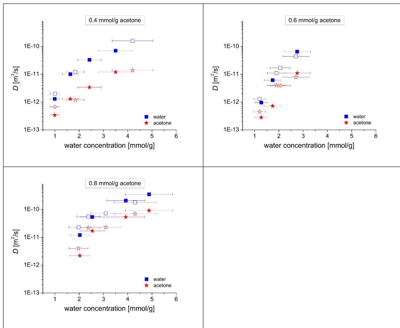
Figure 4 Self-diffusivities of water in the limit of short diffusion times (blue squares) and acetone (red stars) measured as a function of water concentration in non-functionalized Nafion (filled points) and in VA-functionalized Nafion (empty points). The measurements were performed by PFG NMR at 296 K for three constant, within uncertainty, acetone concentrations shown in the figure. The size of the points indicates uncertainty in the self-diffusion coefficients ( D ).
