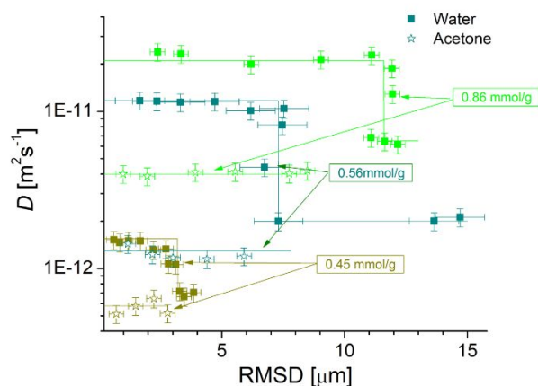
Figure 2 Dependence of the measured self-diffusivities of acetone (stars) and water (squares) on root MSD in VA-functionalized Nafion membranes at 296 K. Water concentration in Nafion was held constant at \sim 2 mmol/g. Solid lines are guidelines shown as visual aids.
