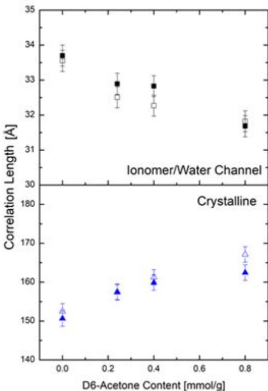
Figure 5 SAXS correlation lengths averaged over 3 water concentrations (see Fig. S4) as a function of acetone concentration in non-functionalized Nafion (filled points) and VA functionalized Nafion (empty points) at 296 K.
