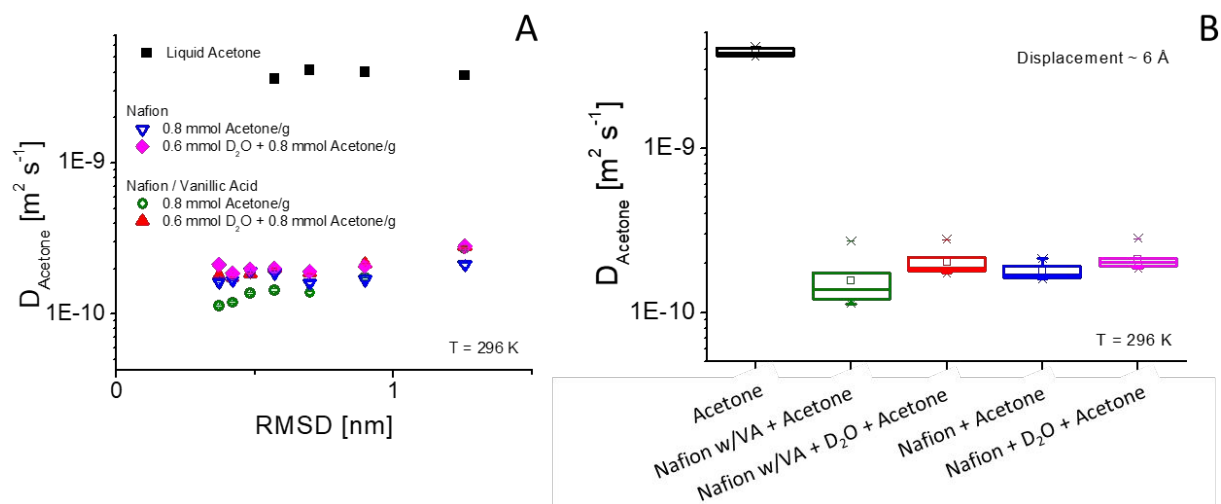
Figure 7 Acetone self-diffusion coefficients from QENS measurements presented as a function of RMSD (A), and acetone self-diffusion coefficients averaged for the full QENS range (B). Each box in (B) represents one standard deviation with the internal line denoting the mean, open symbols represent the mode, the 'x' symbols denote the extremes.
