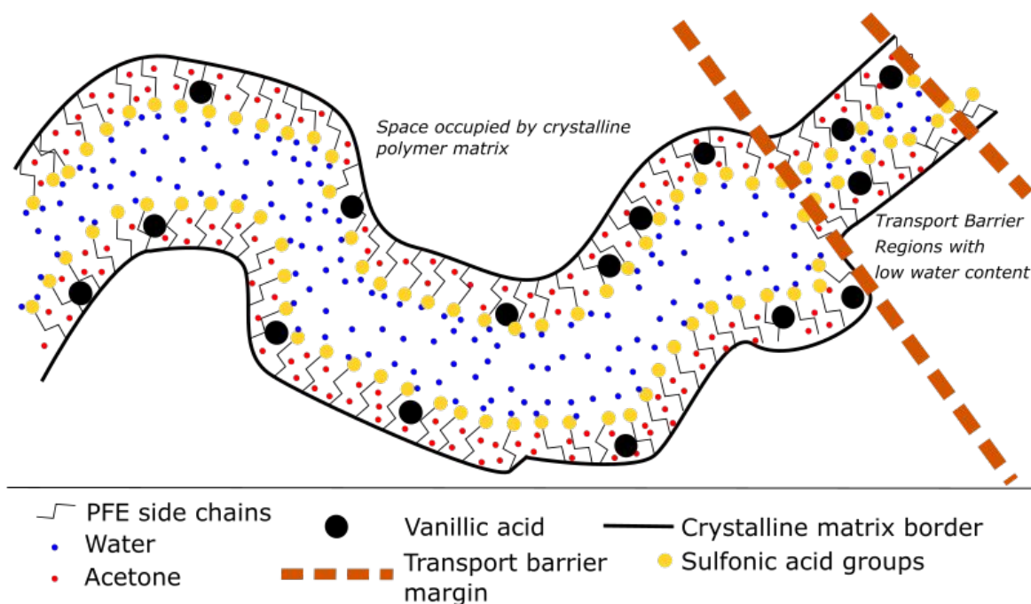
Figure 6 Schematic presentation of the microscopic structure of Nafion with the preferred locations of water, acetone, and vanillic acid.
