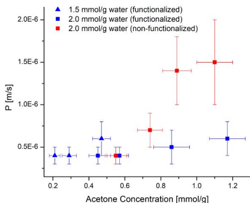
Figure 3 Estimated values for domain boundary permeance for water with changing acetone concentration at 1.5 mmol/g water (blue triangles) and 2 mmol/g water (blue and red squares). Red points indicate values of P estimated for non-functionalized Nafion membranes 19 , while blue points indicate P estimates for Nafion functionalized with VA.
