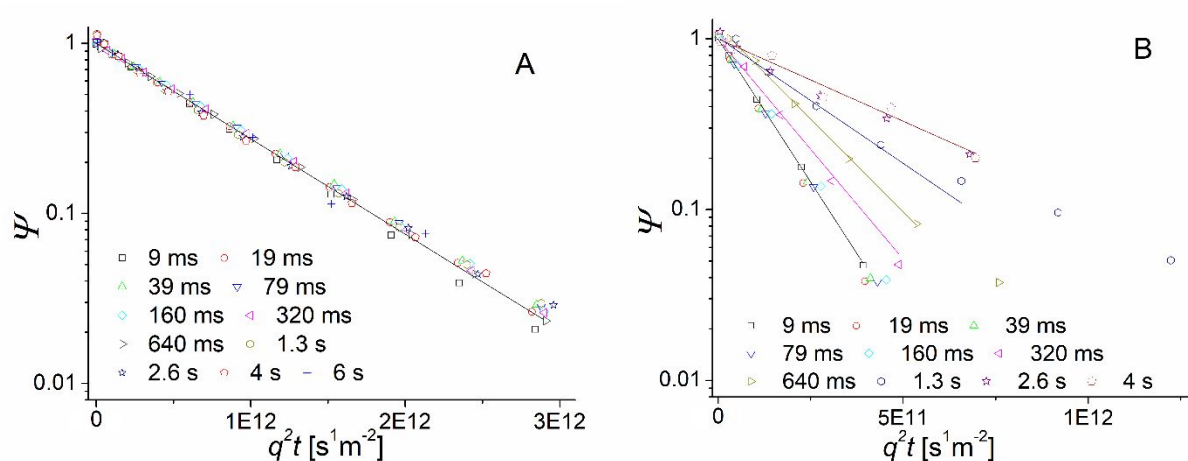
Figure 1 Examples of 1 H PFG NMR attenuation curves for acetone (A) and water (B) in a VA functionalized Nafion membrane at 296 K. The intramembrane concentrations of acetone and water were 0.47 mmol/g and 1.4 mmol/g, respectively. Solid lines represent the best fit lines using Eq.1 for the range of the diffusion times showing coinciding data, within uncertainty. Dotted lines are the best fit lines using Eq.1 of the initial parts of the attenuation curves, which show deviations from the monoexponential behavior. These initial parts correspond to an essentially monoexponential behavior, within uncertainty.
