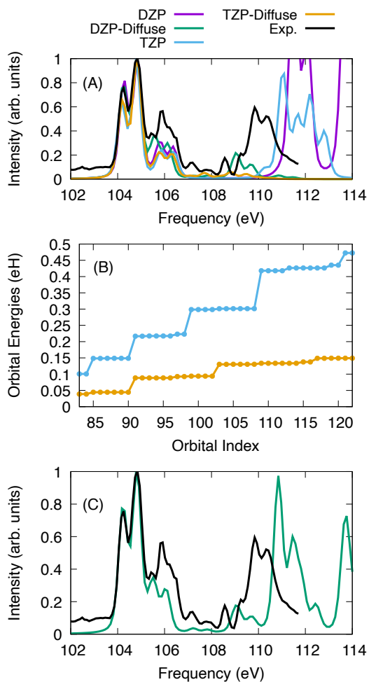
Fig. 3 (A): L 2,3 edge X-ray absorption spectroscopy for SiCl 4 using only 241 determinants for all basis sets. The X2C-NOCI results were shifted and normalized to coincide with the tallest peak of the experimental spectrum. (B): X2C-HF Orbital energies of the reference target orbitals used in the gBLW optimization using the Sapporo triple zeta basis with and without diffuse functions. (C): L 2,3 -edge experimental spectrum and NOCI computed with the Sapporo-DZP basis with diffuse functions with a larger X2C-NOCI space (409 determinants).
