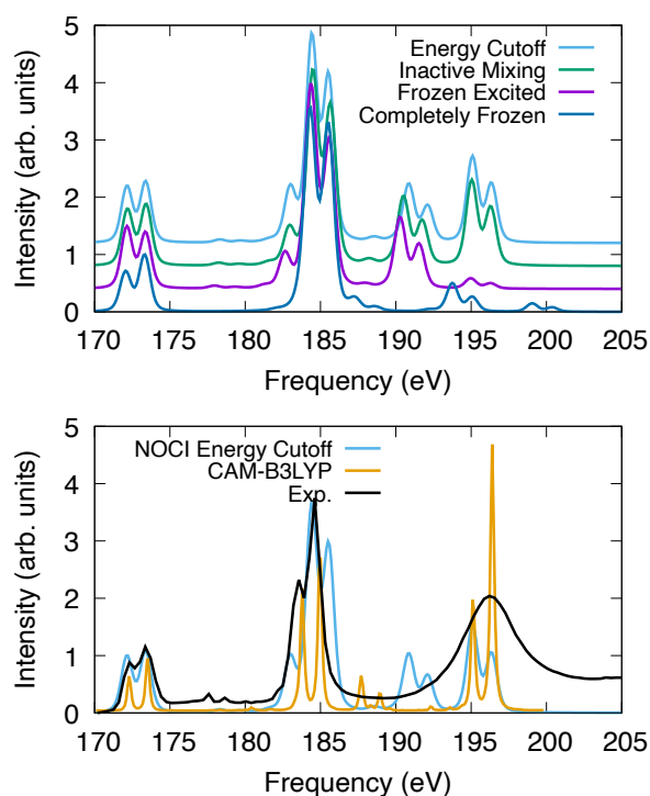
Fig. 2 L_{2,3} edge X-ray absorption spectroscopy for \text{SF}_6 . The spectra were shifted and normalized to coincide with the peak at 173 eV. X2C-NOCI was performed using the Sapporo double zeta basis. The bottom plot also has the experimental spectrum, 90 and one computed using response theory with CAM-B3LYP. 91
