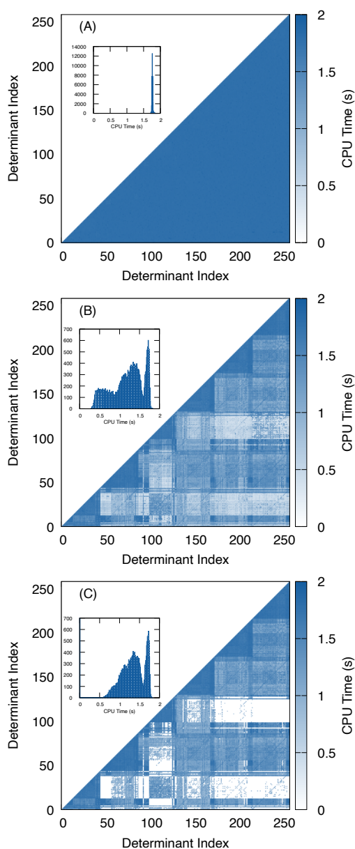
Fig. 6 Heat maps of the time to compute each of the two electron terms (CPU Time) with respect to the determinant index using the unscaled density (A) vs the overlap-scaled density algorithm (B) and the overlap-scaled density with the Slater-Condon screening (C). A histogram of each set of timings (summed over all respective elements) are included in the inset.
