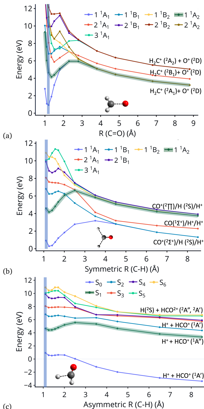
Fig. 4 Energies of singlets calculated at the geometries produced with LIIC along C=O stretch (a); symmetric C-H stretch with both bonds being stretched (b); asymmetric C-H stretch where only one CH is stretched (c). The calculations were done at CASSCF(8,9)/cc-pVDZ level of theory. The region of vertical excitation is highlighted with blue. The curve representing the S_1 state is highlighted with green thick line. In panels (a) and (b) that use symmetry this is the 1^1A_2 state, while for panel (c) it is the first excited S_1 across the whole curve.
