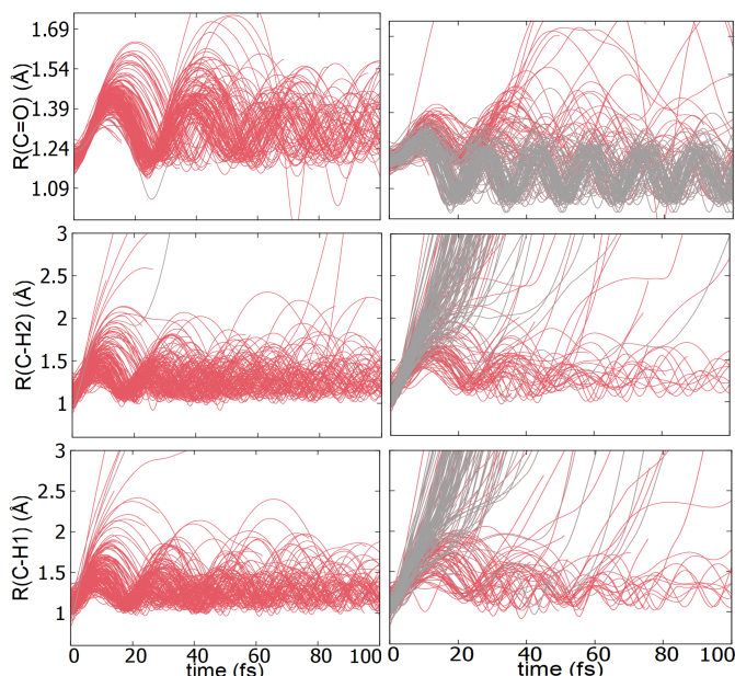
Fig. 3 Plots of internal coordinates vs time for the dynamics ran on the S 1 (left) and S 2 (right) states. The trajectories dissociating to 3 fragments such as CO + H + + H + and CO + + H + + H are shown in grey.
