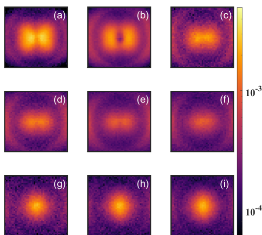
Fig. 5 Two dimensional projection of the momentum distribution for O^+(CD_2O^{2+}) produced with various laser intensities. The laser polarization is along horizontal direction in all the panels. The momentum range of \pm 40 a.u. are displayed at each intensity. The subpanels are ordered with laser peak intensity at (a)-(i) 43, 67, 96, 120, 144, 168, 192, 216, 240 TW/cm^2 , respectively. The low KE (center region) change its shape and relative amplitude dramatically as the intensity changes. This change in angular distribution indicates that at different intensity, the low KE O^+(CD_2O^{2+}) are coming from different mechanism.
