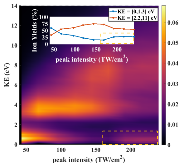
Fig. 6 KE distribution of O^+(CD_2O^{++}) fragment as function of laser power (peak intensity). The single ionization's contribution is mostly at the low KE low intensity region (0 to 1.3 eV). The double ionization is thought to be higher KE higher intensity region (2.2 to 11 eV). The even higher ionization channels are showing in the even higher KE even higher intensity. And at really high intensity, low KE region, we see ion yields which are presumably from the non-dissociative double ionization CD_2O^{++} , which coincides at the same mass-to-charge ratio with the O^+ fragment.
