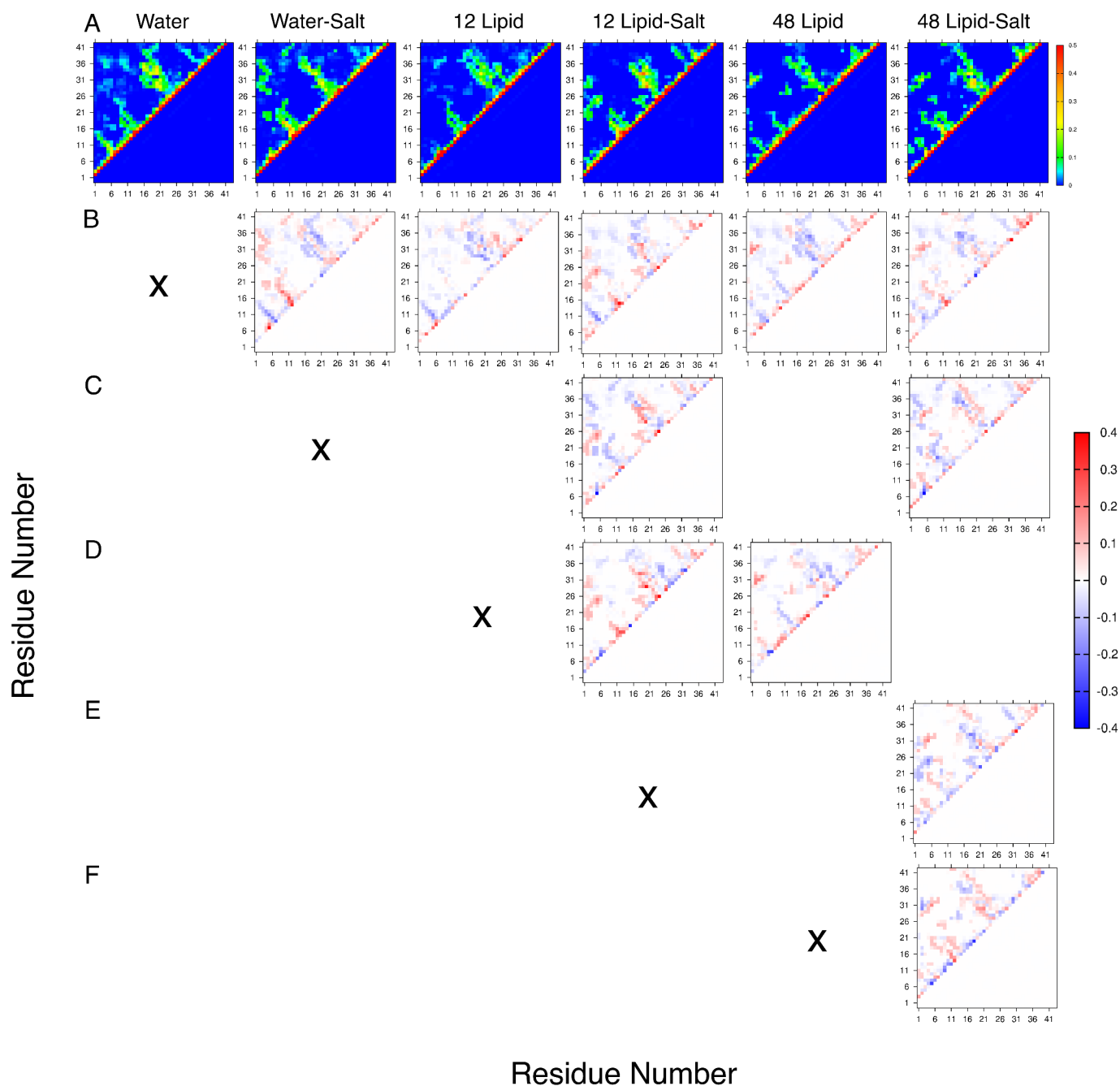
Fig. 6 (A) Tertiary contact maps of A \beta 42, showing the probability (color bar) that pairs of C \alpha atoms are within a distance of 6 Å for each of the six different conditions under study. (B-F) Pairwise difference contact maps indicating stronger (red) and weaker (blue) contacts relative to the reference contact map indicated by X.
