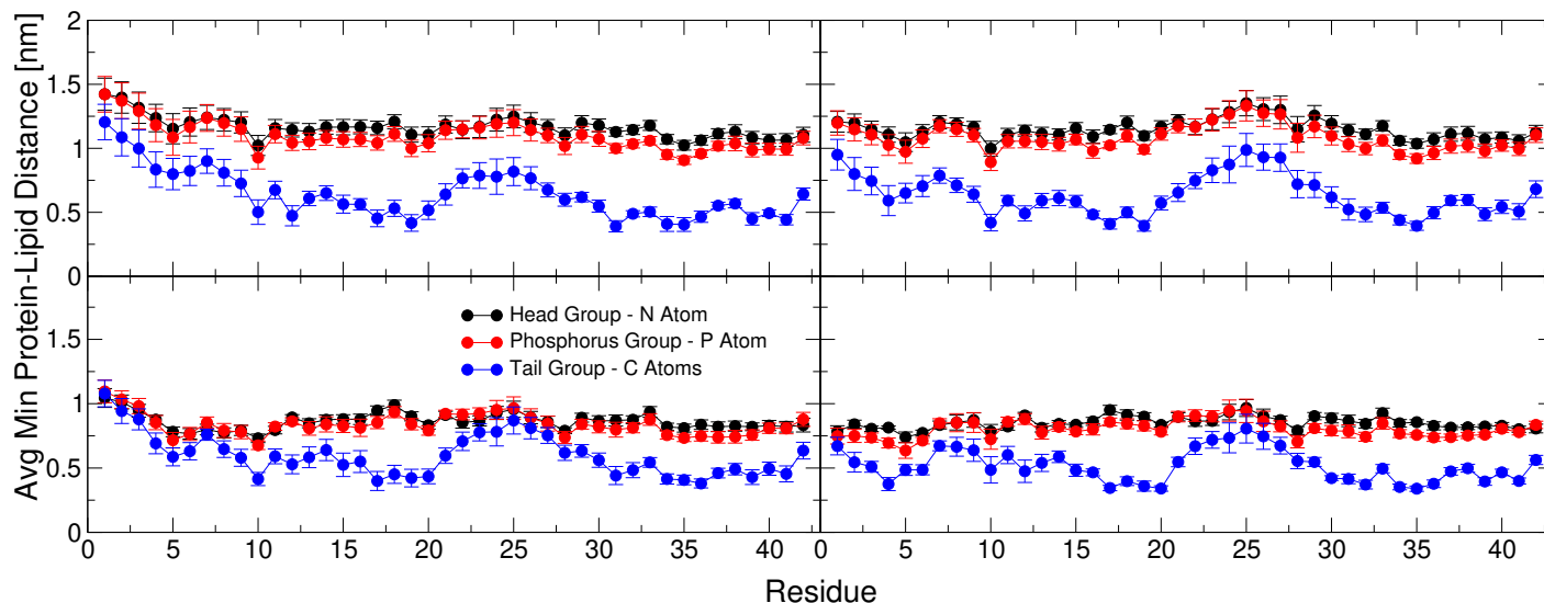
Fig. 7 A minimum average distance between A\beta 42 residues and DMPC head groups, the N atom (black) and the P atom (red), and any carbon atom of DMPC tails (blue) for the following conditions: (A) 12 lipids and pure water, (B) 12 lipids and 150 mM salt, (C) 48 lipids and pure water, and (D) 48 lipids and 150 mM salt. For each of the four conditions, the averages are calculated using 50-250 ns of the respective 10 replica trajectories and error bars are calculated as SEM values reflecting trajectory-to-trajectory variability.
