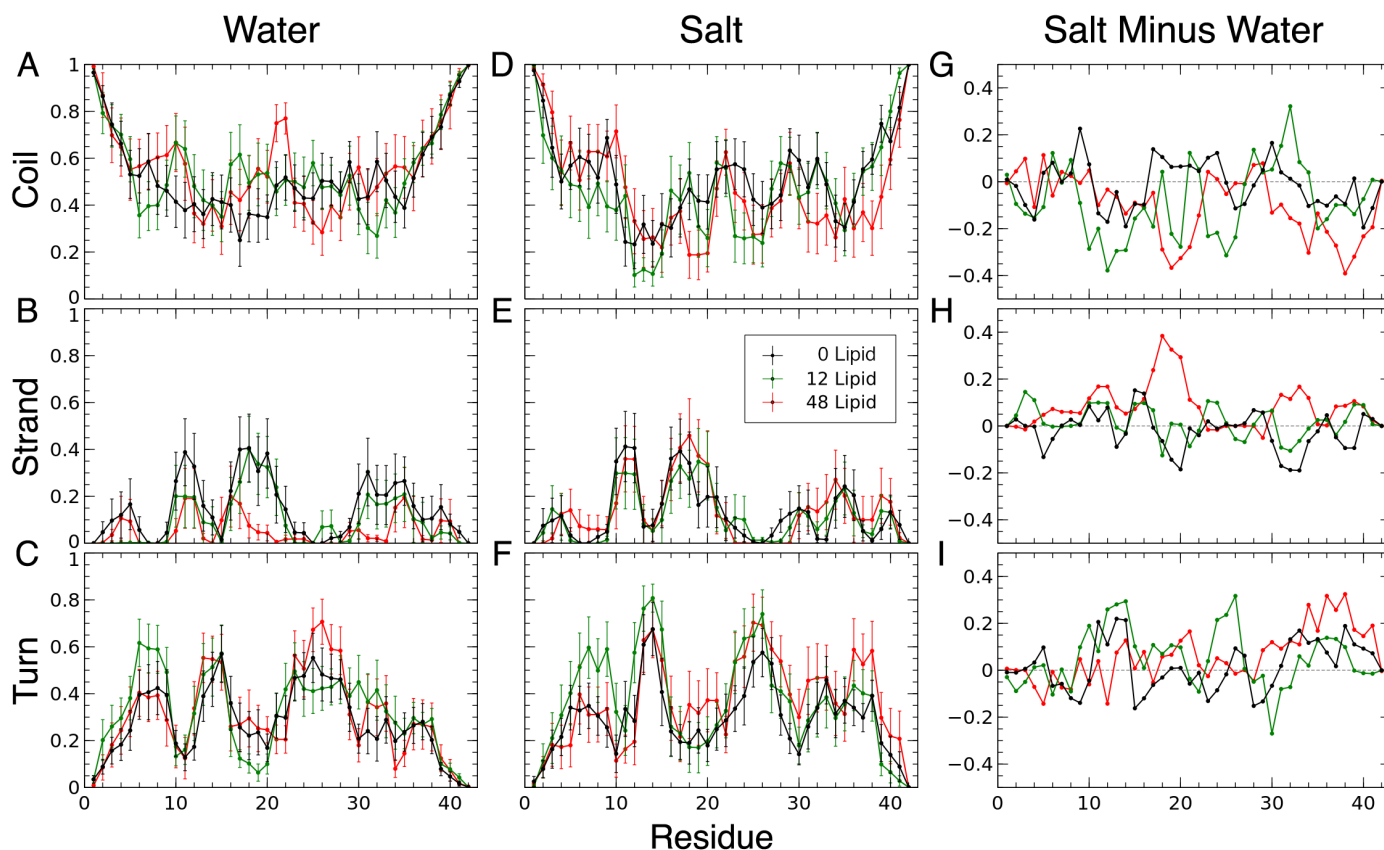
Fig. 5 STRIDE-based per-residue coil, \beta -strand, and turn secondary structure propensities of A \beta 42 monomer in the presence of 0, 12, and 48 DMPC molecules (0, 27, and 109 mM) in (A, B, C) pure water and (D, E, F) water with 150 mM NaCl. (G, H, I) Propensity differences between water with salt and water without salt are shown for three DMPC concentrations. Error bars correspond to SEM values and reflect trajectory-to-trajectory variability as described in Methods .
