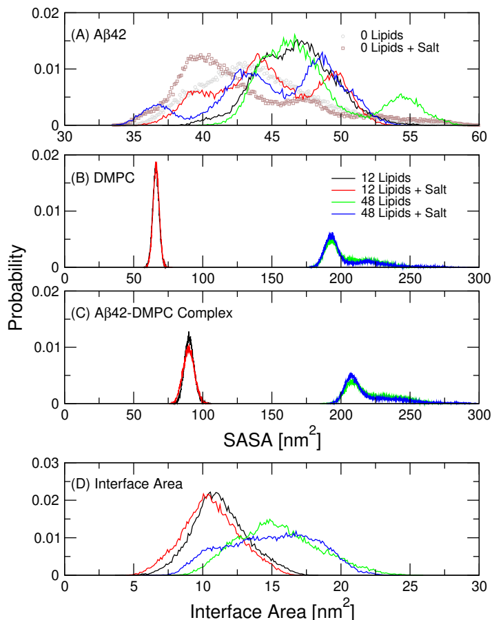
Fig. 8 Normalized distributions of the SASA of (A) A\beta 42 monomer, (B) DMPC cluster, (C) A\beta 42 -DMPC complex, and (D) the interface area between A\beta 42 and the DMPC cluster, as described in Methods . Additional distributions of the SASA values of A\beta 42 in the absence of lipids are included in panel (A) for reference and are also displayed in Fig. S10 to facilitate a better comparison among the distributions.
