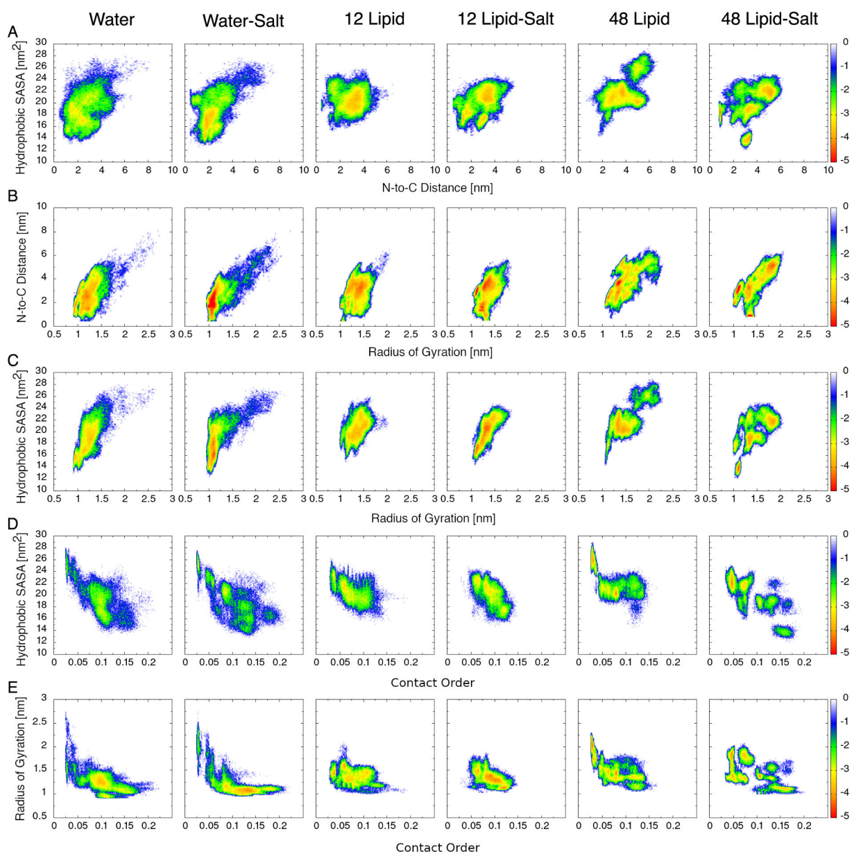
Fig. 3 Free energy landscapes of A\beta 42 monomers for the following pairs of reaction coordinates: (A) hydrophobic SASA vs. N2CD, (B) N2CD vs. R_g , (C) hydrophobic SASA vs. R_g , (D) hydrophobic SASA vs. contact order, and (E) R_g vs. contact order. Each column corresponds to a different MD trajectory set corresponding to six different conditions under which A\beta 42 conformational dynamics is examined.
