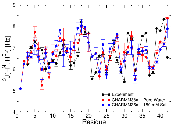
Fig. 2 {}^3J(\text{H}^N, \text{H}^{C\alpha}) coupling constants for each amino acid residue of an A\beta 42 monomer from experiment 71 and calculated from MD trajectories (see Methods ), using the Hu and Bax Karplus parameter set 57 , in the absence and presence of 150 mM NaCl. Error bars for MD-derived coupling constants are calculated as SEM using the averages of the corresponding set of 10 replica trajectories. Results with other Karplus parameter sets are shown in Tables S2 and S3 and Fig. S5
