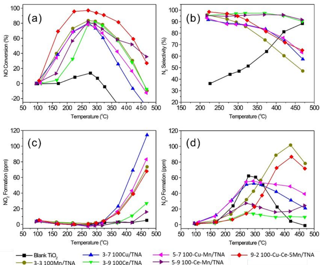
Fig. 1 Catalytic performance of the selected transition metal (i.e., Cu, Mn, and Ce) doped \text{TiO}_2 nanoarray based monolithic catalysts: (a) NO conversion, (b) \text{N}_2 selectivity, (c) \text{NO}_2 formation, and (d) \text{N}_2\text{O} formation. Feed gas: 500 ppm NO + 500 ppm \text{NH}_3 + 5 vol.% \text{O}_2 balanced with \text{N}_2 and space velocity of 15,000 /h.
