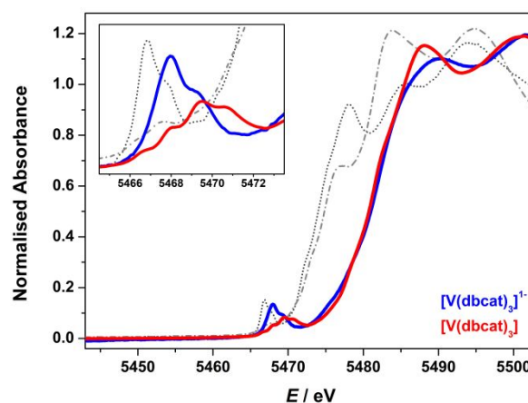
Fig. 2 Overlay of the normalised V K-edge X-ray absorption spectra of [\text{V}(\text{dbcats})_3] and \text{Na}[\text{V}(\text{dbcats})_3] . The inset shows expansion of the pre-edge region. The spectra for [\text{V}(\text{edt})_3] (dotted line) and [\text{V}(\text{bpy})_3] (dash-dot line) are provided for reference.
