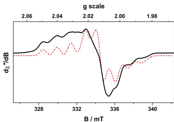
Fig. 1 X-band EPR spectrum of [\text{V}(\text{dbcats})_3] recorded in toluene solution at 30 K. The simulation is shown in red with the experimental spectrum in black (experimental conditions: frequency, 9.4206 GHz; power, 0.63 mW; modulation, 0.2 mT).
