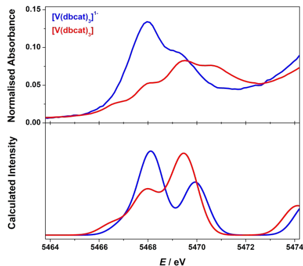
Fig. 3 Experimental (top) and calculated (bottom) V K-pre-edge spectra for [\text{V}(\text{dm}(\text{cat})_3)] and [\text{V}(\text{dm}(\text{cat})_3)]^{1-} obtained from B3LYP TD-DFT calculations. Calculated intensity in arbitrary units.
