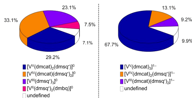
Fig. 4 Configurational ground state compositions from analysis of CAS wavefunctions for [\text{V}(\text{dm}(\text{cat})_3)] and [\text{V}(\text{dm}(\text{cat})_3)]^{1-} .
