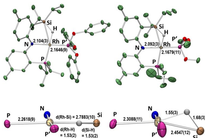
Figure 2. ORTEP drawings (50% probability ellipsoids) of 6 (left) and 10 (right). Selected atom labelling is shown (except for C = green and O = red). The hydrogen atoms except for SiH are omitted for clarity in the top view and only one of the two crystallographically independent molecules of 10 is shown. The bottom view shows only the immediate coordination sphere about Rh in 6 and 10 .
