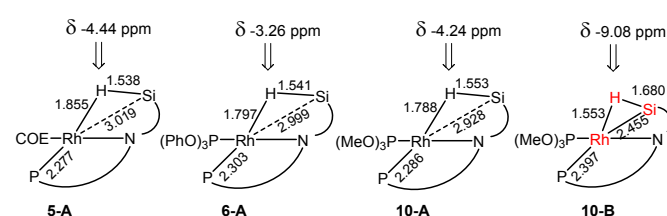
Figure 3. Key interatomic distances and 1 H NMR chemical shifts for SiH in the DFT-calculated structures of 5-A , 6-A , 10-A , and 10-B . The atoms whose positions were restricted in the optimization of 10-B are shown in red.
