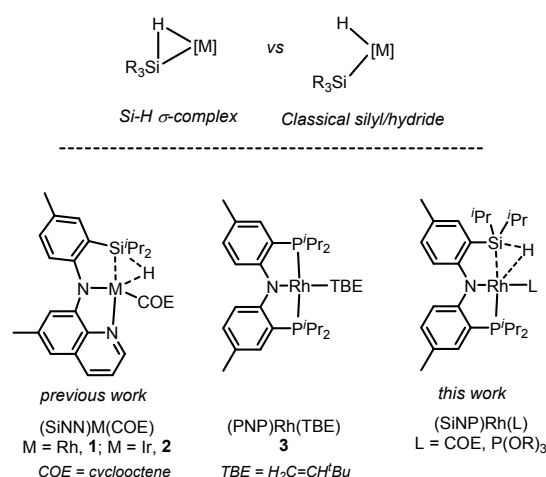
Figure 1. Top: the two extremes of a continuum of interactions of an R 3 Si-H bond with a transition metal. Bottom: the previously reported complexes of the SiNN and PNP pincer ligands, along with the SiNP complexes studies in this work.
