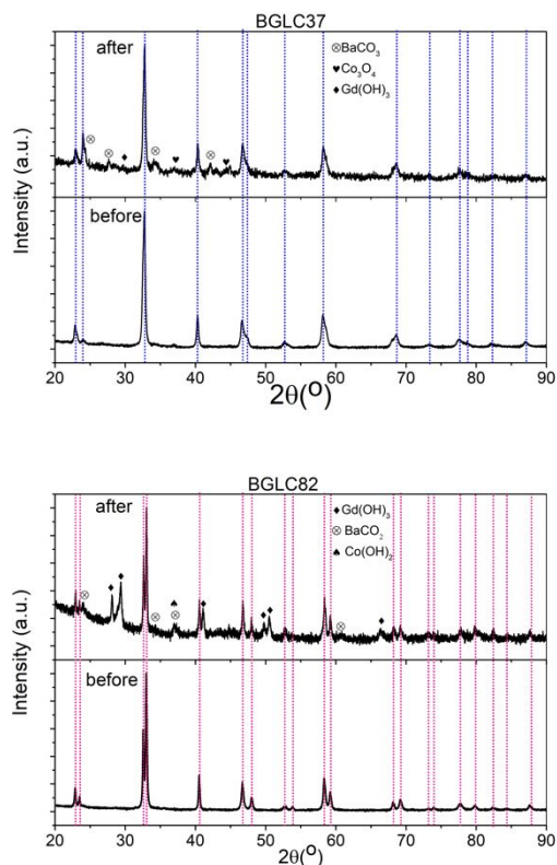
Figure 6. PXRD patterns of BGLC37 and BGLC82 before and after the water vapor treatment at 300 °C and 10.5 bar of p H2O for at least 96 hours.
