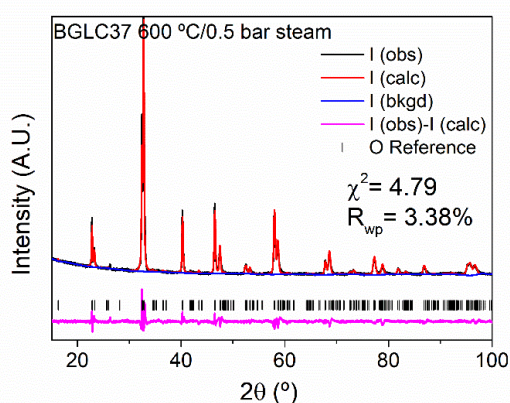
Figure 7. PXRD patterns of BGLC37 after the water vapor treatment at 600 °C and 0.5 bar of p H2O for 72 hours.
