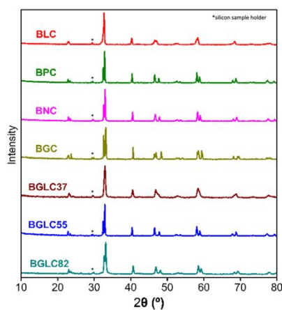
Figure 1. X-ray diffractograms of BLnCs and BGLCs as-prepared samples. Marked peak stems from the silicon XRD sample holder.
