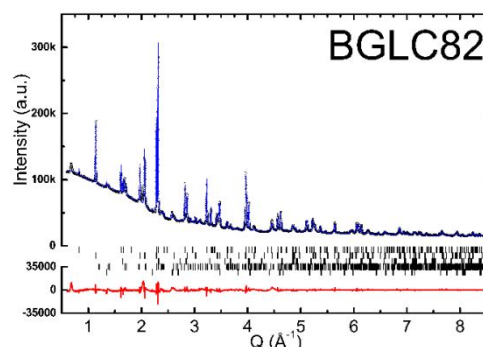
Figure 8. SR-PXRD pattern with the Rietveld refinement of BGLC82 sample exposed at 300 °C and 10.5 bar of H 2 O for 100 hours.
