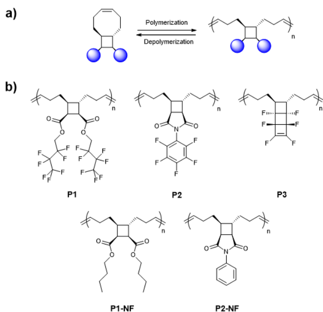
Fig. 1 Depolymerizable polymers based on trans -cyclobutane fused cyclooctene ( t CBCO) monomers. (a) Installing a trans -cyclobutane ring on a 5,6-positions of cyclooctene renders the resulting ROMP polymer depolymerizable, and a diverse range of functional groups can be attached to the cyclobutane to tune the material properties of the polymer. (b) Semi-fluorinated polymers ( P1 , P2 , and P3 ) and the non-fluorinated counterparts for P1 ( P1-NF ) and P2 ( P2-NF ) prepared and studied in this work.
