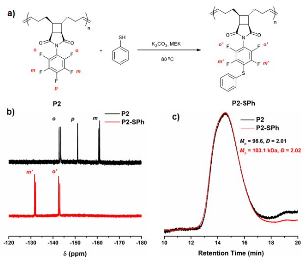
Fig. 7 Post-polymerization functionalization of P2 via para -fluoro thiol ligation. (a) Synthetic scheme for the nucleophilic aromatic substitution of thiophenol on P2 . ^{19}\text{F} NMR spectra (b) and GPC traces for P2 before and after functionalization ( M_n was calculated based on polystyrene standards).
