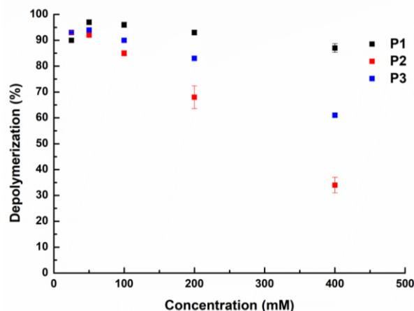
Fig. 4 The extent of depolymerization obtained at various concentrations for the semi-fluorinated depolymerizable polymers P1 , P2 and P3 . Reaction time: 16h.
