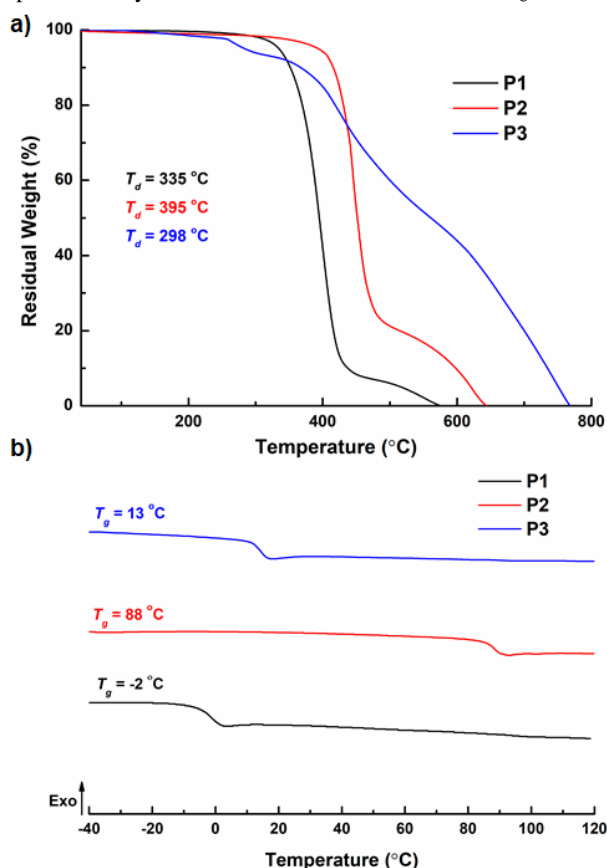
Fig. 3 Characterization of the thermal properties of the semi-fluorinated depolymerizable polymers P1 , P2 , and P3 . (a) Thermogravimetric analysis. (b) Differential scanning calorimetry. T_g is the glass transition temperature while T_d is the temperature at which the polymer experiences 5% weight loss.
