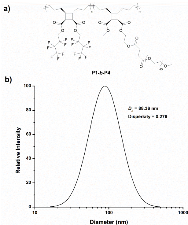
Fig. 6 The structure (a) and dynamic light scattering spectrum for block copolymer P1-b-P4 .
