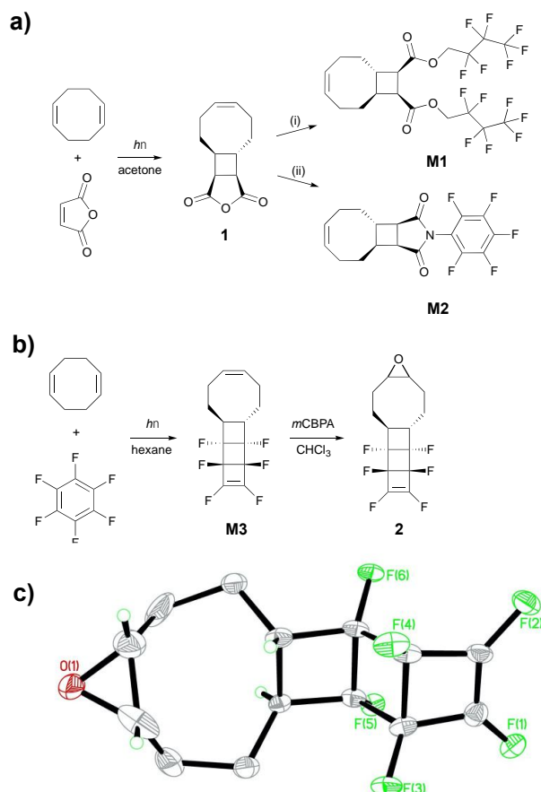
Fig. 2. Synthesis of t CBCO-based semi-fluorinated monomers. (a) Synthetic scheme for semi-fluorinated monomers M1 and M2 . Anhydride 1 , prepared through [2+2] photocycloaddition of 1,5-cyclooctadiene and maleic anhydride, is converted to M1 and M2 via conditions (i), and (ii), respectively. (i) MeOH, reflux; NaOH, H 2 O, 60 °C; 2,2,3,3,4,4,4-heptafluoro-1-butanol, EDC, DMAP, DCM. (ii) Pentafluoroaniline, toluene, 90 °C; sodium acetate, acetic anhydride, 100 °C. (b) Synthetic scheme for M3 and its epoxide 2 . (c) The structure of 2 with 35% thermal ellipsoids; methylene hydrogen atoms have been omitted for clarity.
