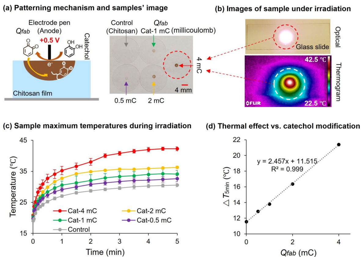
Fig. 1 Photothermal properties of patterned catechol films. (a) Catechol dots (2mm diameter) were electrochemically 'written' onto cast chitosan films. (b) The temperature during NIR irradiation was determined by thermal imaging. (c) The increase of temperature (measured as
