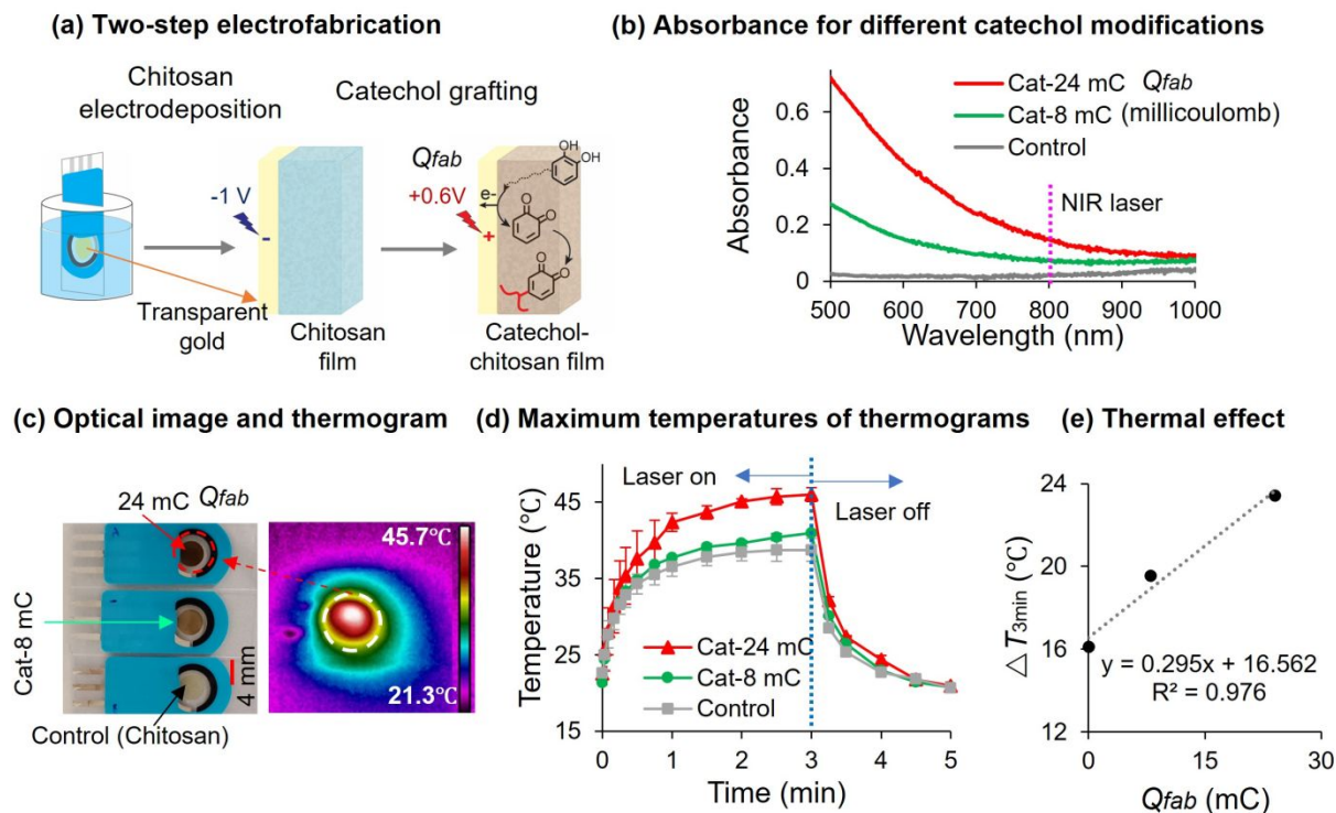
Fig. 2 Photothermal properties of catechol-chitosan coated electrodes. (a) Catechol-chitosan films are electrofabricated on transparent gold electrodes (4mm diameter). (b) UV-Vis spectra of coated-electrodes with different extents of catechol modification (spectra were corrected from the blank signal of uncoated electrode). (c) Optical images and thermogram of film-coated electrode. (d) Maximum temperatures of the coated electrodes (808 nm laser; 0.75 \text{ W/cm}^2 ; data represent mean values \pm SD ( n=3 )). (e) Catechol coatings show a thermal effect which is quasi-linearly correlated to extent of catechol modification ( \Delta T_{3min} is the temperature difference between 0 and 3 min). [Note: “mC” is an abbreviation for millicoulomb.]
