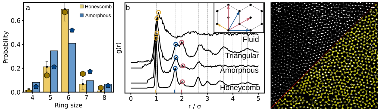
FIG. 2. Structural analysis. (a) Ring size distribution in the honeycomb phase (yellow, determined from 8 representative images) and amorphous phase (blue, determined from 2 representative images). The histogram shows experimental results, the dots the results from simulations. (b) Radial distribution function, g(r) of the three different condensed phases, honeycomb (solid line), amorphous (dotted line), and triangular (dashed line). The g(r) has been normalized to the height of its nearest-neighbour peak as well as shifted along the y -axis. The vertical dotted lines indicate theoretical peak locations, full analysis can be found in the SI. The inset shows a schematic drawing of the three smallest typical distances in our system, 1\sigma (yellow), 1.74\sigma (blue) and 2\sigma (red). The corresponding peaks in the g(r) are highlighted. (c) Triangular lattice: confocal image and bonding network. The top-left half of the image shows the glass-bound patches, indicating the particle centres, while the bottom-right shows the overlaid bonding network where the patches and their bonds are highlighted in yellow.
