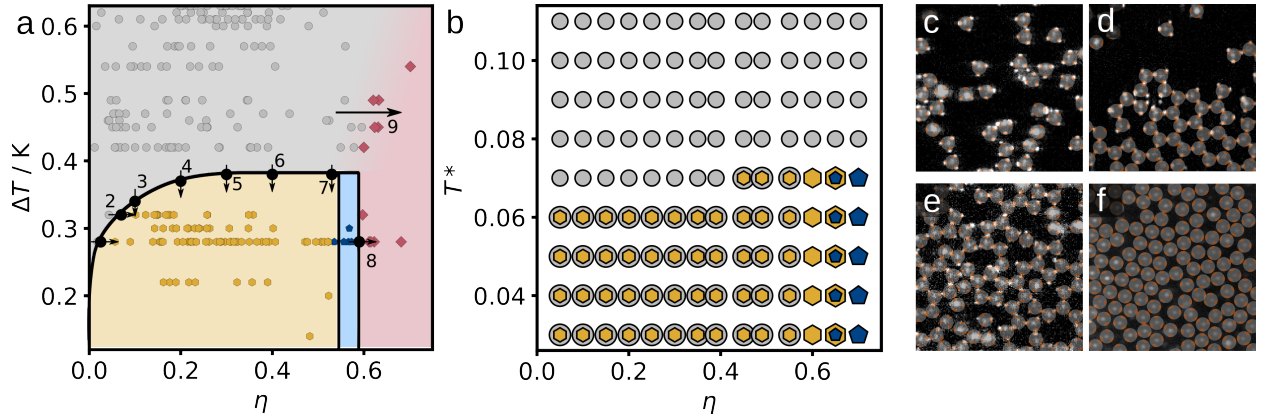
FIG. 4. Phase diagrams (a) Experimental phase diagram constructed from the order parameters in Fig. 3. The fluid phase is indicated in grey, the honeycomb-fluid coexistence in yellow, the amorphous network phase in blue and the triangular phase in red. Black arrows and dots indicate scans and estimated transitions shown in Figure 3. (b) Corresponding phase diagram from simulations. Each point corresponds to a separate simulation. Gray circles indicate fluid, yellow hexagons indicate honeycomb, blue heptagons indicate amorphous network. Note that coexistence points have 2 symbols. (c-f) Illustrations of the experimentally observed phases: fluid (c), honeycomb-fluid coexistence (d), amorphous network (e) and triangular lattice (f). Here, patchy particle sketches are overlaid on small sections of confocal microscope images (insets of Figure 1d-g) to illustrate the assembled structures most clearly.
