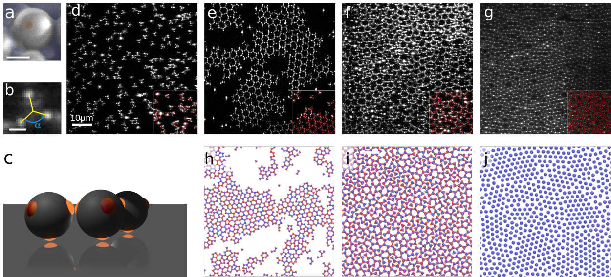
FIG. 1. Pseudo-trimeric tetrahedral particles and their phases: fluid, honeycomb, amorphous and triangular (a-c) Tetrahedral particles become trivalent upon attachment of one patch to the substrate. (a) Scanning electron microscopy (SEM) image of a patchy particle with patch highlighted in orange. (b) Confocal microscope image of a particle taken under fluorescence. The projected angle between the patches is indicated by \alpha , corresponding to 120^\circ . The scale bar in both panels is 1\mu m . (c) Reconstruction of surface-bound particles, exhibiting three remaining patches to bind to other particles. (d)-(g) Confocal microscopy images of experimentally observed phases: fluid (d), honeycomb-fluid coexistence (e), amorphous network (f), and triangular phase (g). Inset shows part of the image with particles superimposed in red. (h)-(j) Snapshots of the phases observed in the simulations, corresponding to the experimental phases in (d)-(g). In panel (j), the red patches are hidden to highlight the triangular packing of particles.
