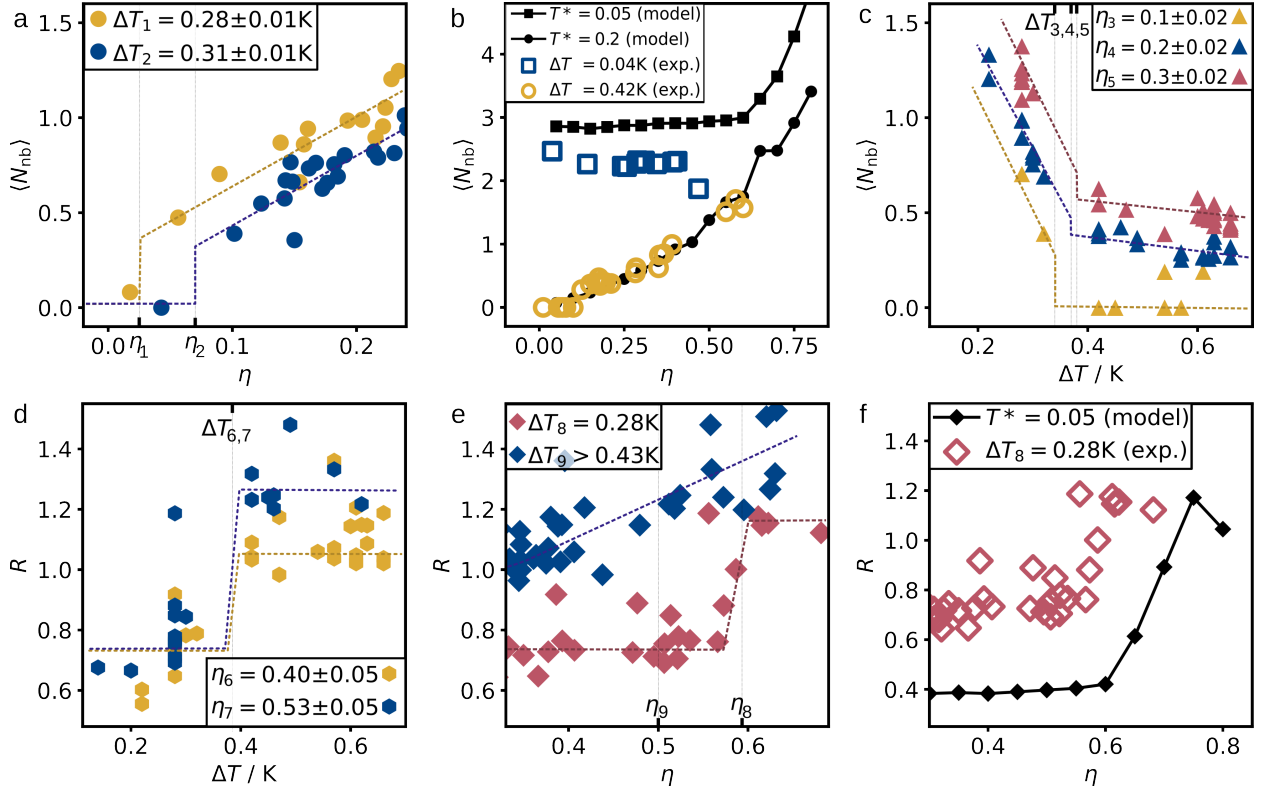
FIG. 3. Structural order parameters as a function of density and temperature. (a-c) Average number of neighbours \langle N_{nb} \rangle as a function of surface coverage \eta (a,b) and \Delta T (c). Panel (a) shows experimental data for two different attractive strengths (along arrows 1 and 2 in Fig. 4a, see legend), while (b) compares data from simulations in the fluid and honeycomb phase (black solid symbols and lines) with experimental data at corresponding attractive strength (coloured open symbols). Panel (c) shows \langle N_{nb} \rangle as a function of \Delta T for three densities (along arrows 3, 4 and 5 in Fig. 4a). (d,e) Height ratio R of characteristic g(r) peaks as a function of \Delta T (d) and \eta (e). Panel (d) shows R as a function of \Delta T for two high surface coverages (arrows 6 and 7 in Fig. 4a.), while panel (e) show R as a function of \eta for experiments along arrow 8 and simulations at T^* = 0.05 . The latter reveals good qualitative agreement of R in experiment and simulations. In all Figure panels, dotted lines are guides to the eye.
