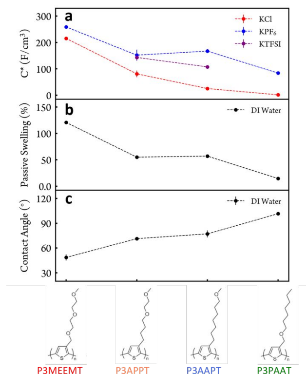
Figure 4. (a) Volumetric capacitance C* in 100 mmol/L KCl (aq) (red), KPF 6(aq) (blue) and KTFSI (purple). (b) Passive swelling of polymers in DI water. We did not observe significant difference of passive swelling in KCl (aq) , KPF 6(aq) or DI water. (c) Water contact angle of polymers. Dash lines are guide for the eye.
