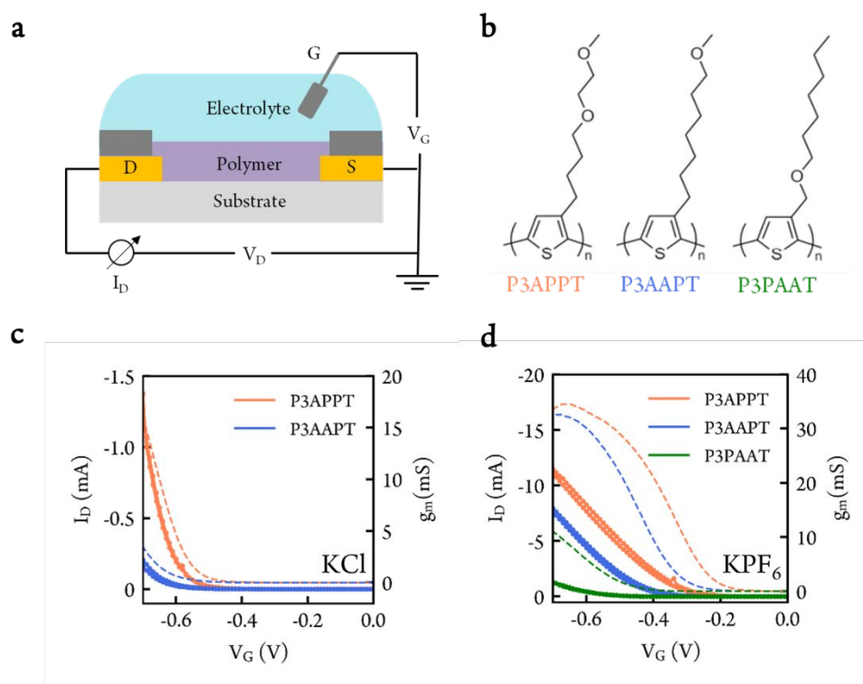
Figure 1. (a) OEET device schematic. S and D represent source and drain electrode, respectively. Insulating layer (dark grey) was applied on top of gold electrode to prevent direct contact between gold and electrolyte. A Ag/AgCl pellet was used as gate electrode (G). (b) Chemical structure of reduced-oxygen-content side chain polymers. An example OEET transfer curve (dot line) and transconductance (dash line) of reduced-oxygen-content side chain polymers in 100 mmol/L (c) KCl (aq) and (d) KPF 6(aq) . Transistor channel width/length = 4000 \mu m /10 \mu m. V_D = -0.6 V for all measurements.
