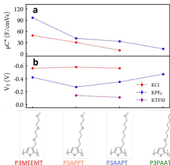
Figure 2. (a) OECT material figure of merit \mu C^* and (b) OECT threshold voltage ( V_T ) in 100 mmol/L \text{KCl}_{(\text{aq})} (red), \text{KPF}_{6(\text{aq})} (blue) and KTFSI (purple). Dash lines are guide for the eye.
