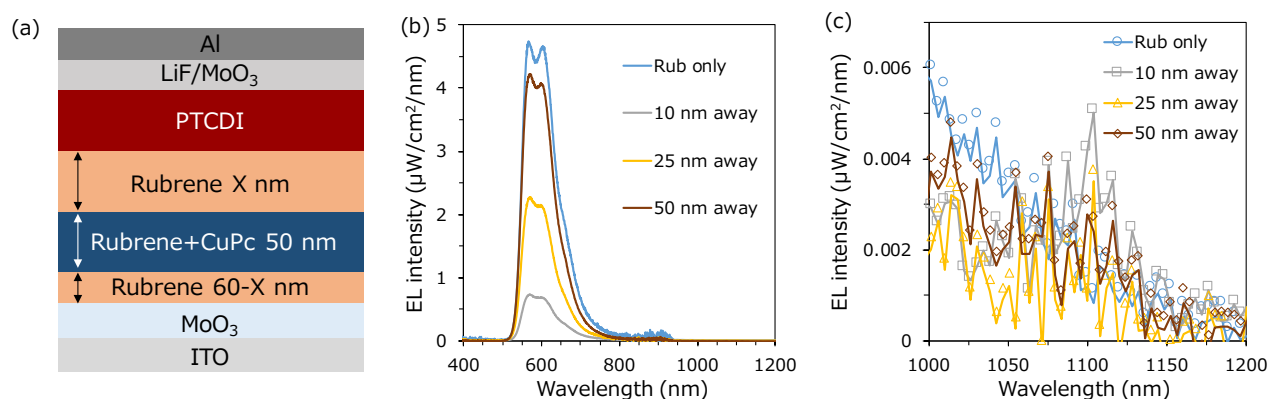
Fig. 3 (a) Schematic of the device with 50 nm of CuPc-doped rubrene layer away from the D/A interface. (b, c) EL emission spectra with a constant current flow ( 1000 \text{ mA/cm}^2 ) for the devices without CuPc doping (blue) and with 50 nm of CuPc-doped rubrene layer away from the D/A interface. The thicknesses of rubrene interlayers at the D/A interface are 10 nm (grey), 25 nm (yellow), and 50 nm (brown).
