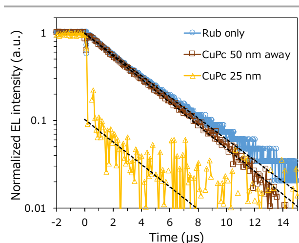
Fig. 4 EL decay for the device without CuPc doping (blue circle), with 50 nm of CuPc-doped rubrene layer at 50 nm away from the D/A interface (brown square), and with 25 nm of CuPc-doped layer at the D/A interface (yellow triangle). Voltages of 4.6, 6.0, and 11 V were applied to each device. Curves were fitted to the EL decay using single exponential functions (broken lines).
