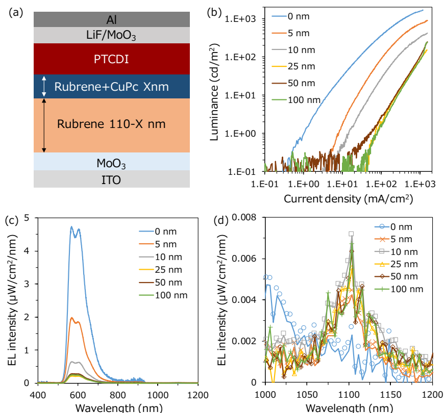
Fig. 2 (a) Schematic of the device with CuPc-doped rubrene layer at the D/A interface. (b) L–J curves and (c, d) EL emission spectra with a constant current flow (1000 mA/cm 2 ) for the devices with 0 nm (blue), 5 nm (orange), 10 nm (grey), 25 nm (yellow), 50 nm (brown), 100 nm (green) of CuPc-doped rubrene layers at the D/A interface.
