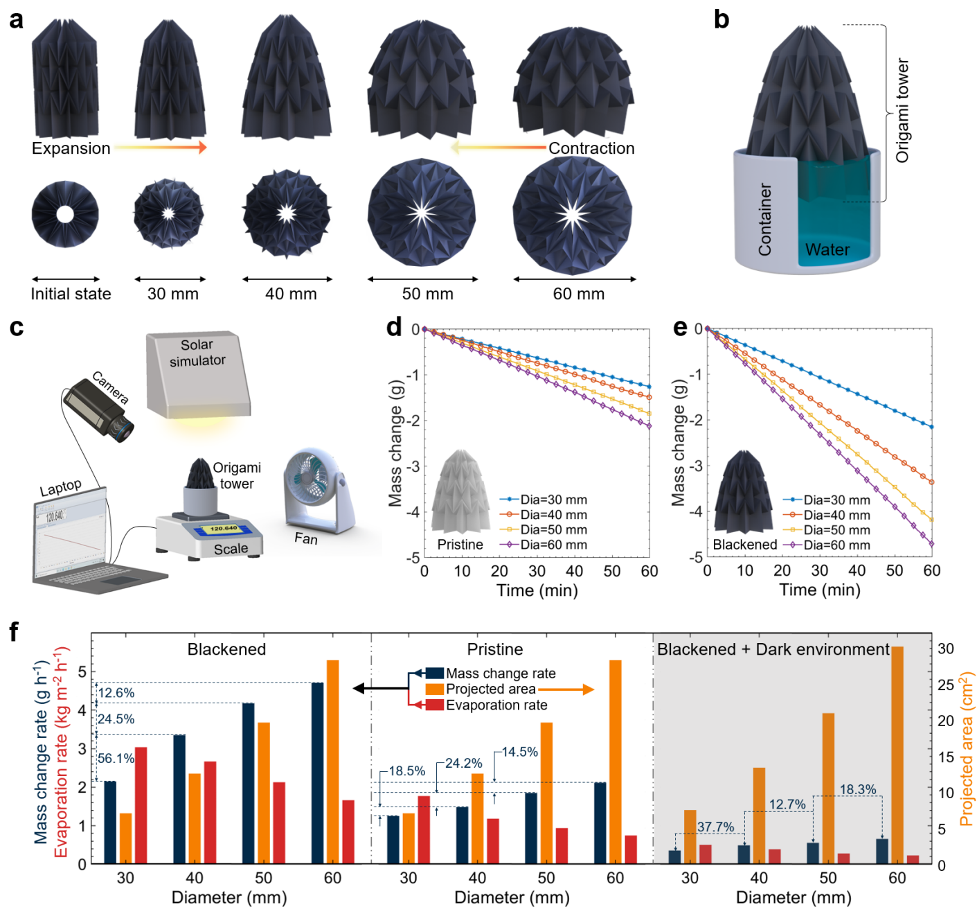
Fig. 4 Convertible origami tower in the solar steam generation measurement. (a) Schematic representations of the expansion process (from left to right) and contraction process (from right to left) of the convertible origami tower in the side view (the first row) and top view (the bottom row), respectively. The marked dimensions at the bottom refer to the maximum diameter of the origami tower. (b) Schematic of the evaporation device for solar steam generation in the measurement of water evaporation rate. The origami tower float on water with one-eighth length immersing in water. The 3D printed cup with different inside diameters functions as the container. (c) Schematic illustration of the experimental setup for the steam generation experiment, involving the solar simulator, infrared thermal camera, electrical scale, electrical fan, laptop, and origami tower evaporator. Mass changes of water with pure cellulose paper-based origami tower (d) and blackened cellulose paper-based origami tower (e) in different diameters under one sun illumination. Insets show the pristine cellulose paper-based origami tower and blackened cellulose paper-based origami tower in the diameter of 40 mm, respectively. (f) The dependence of mass change rate (black bar, left y-axis) and evaporation rate (red bar, left y-axis) with corresponding projected area (orange bar, right y-axis) for the pristine and blackened origami tower with different diameters under solar illumination, and for the blackened ones in the dark environment, respectively. The projected area refers to the area of the origami tower seen from the top view.
