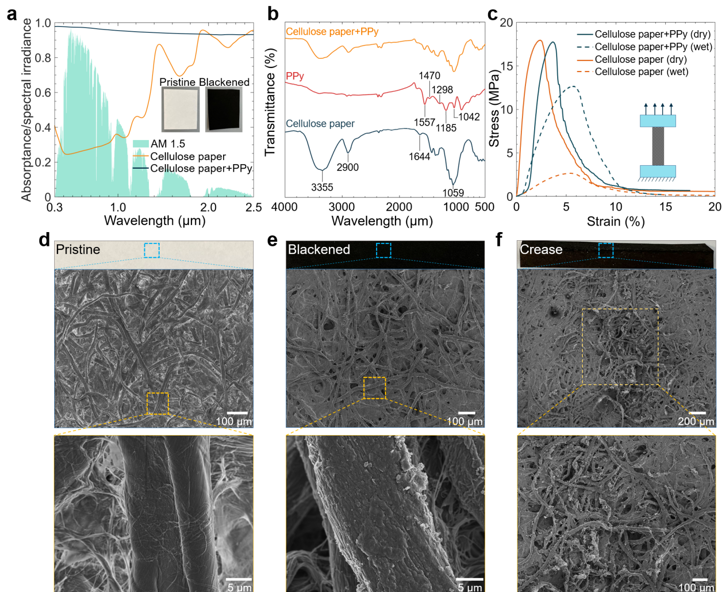
Fig. 3 Characterizations of the composite membrane. (a) The absorbance spectra of the pristine cellulose paper and the PPy-compounded cellulose paper in wet state displaying against the AM 1.5 spectral solar irradiance spectrum. (b) FTIR spectra of pristine cellulose paper, PPy powder, and PPy-compounded cellulose paper showing the responding chemical composition. (c) Tensile stress-strain curves of pristine cellulose paper and PPy-compounded cellulose paper in the dry state and wet state, respectively. (d,e) Photographs and scanning electron microscopy (SEM) images display the surface morphology of unfolded pristine cellulose paper and PPy-compounded cellulose paper at different magnifications. (f) Optical image and SEM images of the crease of PPy-compounded cellulose paper at different magnifications.
