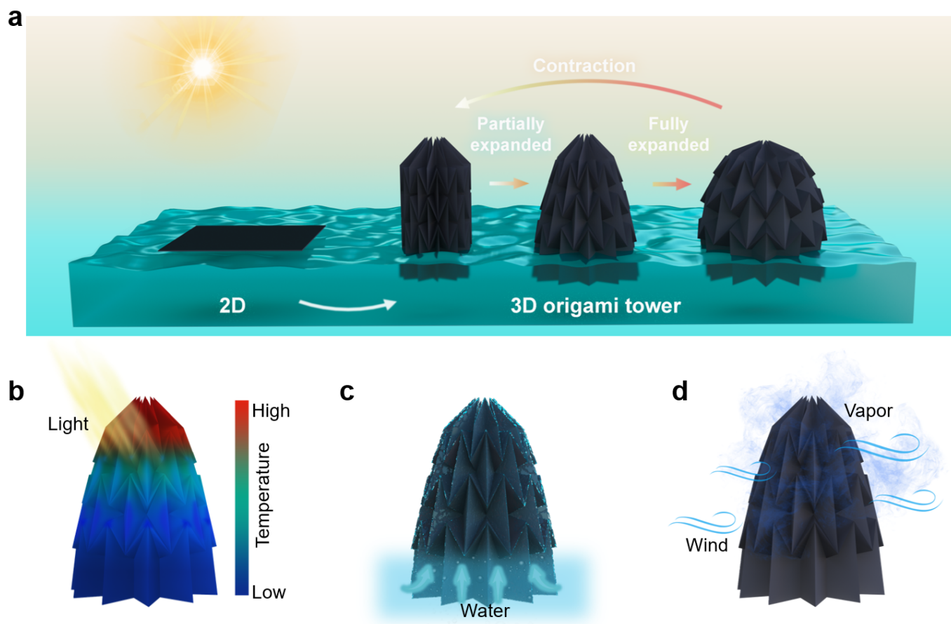
Fig. 1 Schematic illustration of the portable origami tower working as a convertible solar-driven steam generator. (a) Schematic showing the solar-driven evaporators are designed in the form of floating 2D membrane and convertible 3D origami towers. (b-d) Schematic demonstration of light absorption, water transportation, and vapor diffusion of origami tower during the desalination process.
