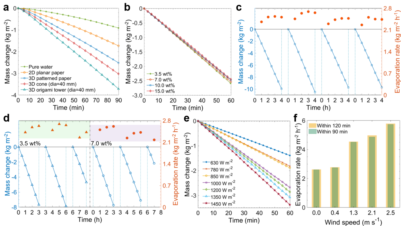
Fig. 6 Solar desalination performance of the origami tower and enhanced evaporation rate under convective flow. (a) Mass changes of water with different shape of evaporators under one sun irradiation. (b) Mass changes of saline solution with different salinities applying an origami tower in the diameter of 40 mm. (c) The mass changes and the corresponding evaporation rates of water for an origami tower with the diameter of 40 mm using the 3.5 wt% NaCl solution in the repeating long-term desalination tests. (d) The mass changes and the corresponding evaporation rates of water for an origami tower with the diameter of 40 mm using the 3.5 wt% and 7.0 wt% NaCl solutions in the continuous long-term desalination tests. (e) The mass changes of 3.5 wt% NaCl solution for an origami tower with the diameter of 40 mm under different solar intensities. (f) The average overall water evaporation rates with an origami tower (40 mm diameter) applying various airflow speeds.
