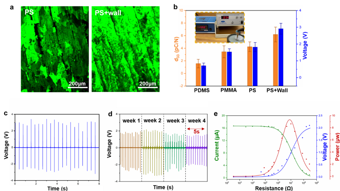
Figure 4. Piezoelectric properties of the (001)-oriented glycine-PVA films. (a) SHG images of the glycine surface from the (001)-oriented glycine-PVA films (PS+wall) and mis-oriented glycine-PVA film (PS). (b) Comparison of d_{33} coefficients and piezoelectric voltage output measured of glycine-PVA films grown on different substrates with different crystal orientations. (c) Piezoelectric voltage output of the (001)-oriented glycine-PVA film measured under a 30-N impulse force. (d) Long-term time-dependent piezoelectric outputs. (e) Load-resistance curve of the (001)-oriented glycine-PVA film.
