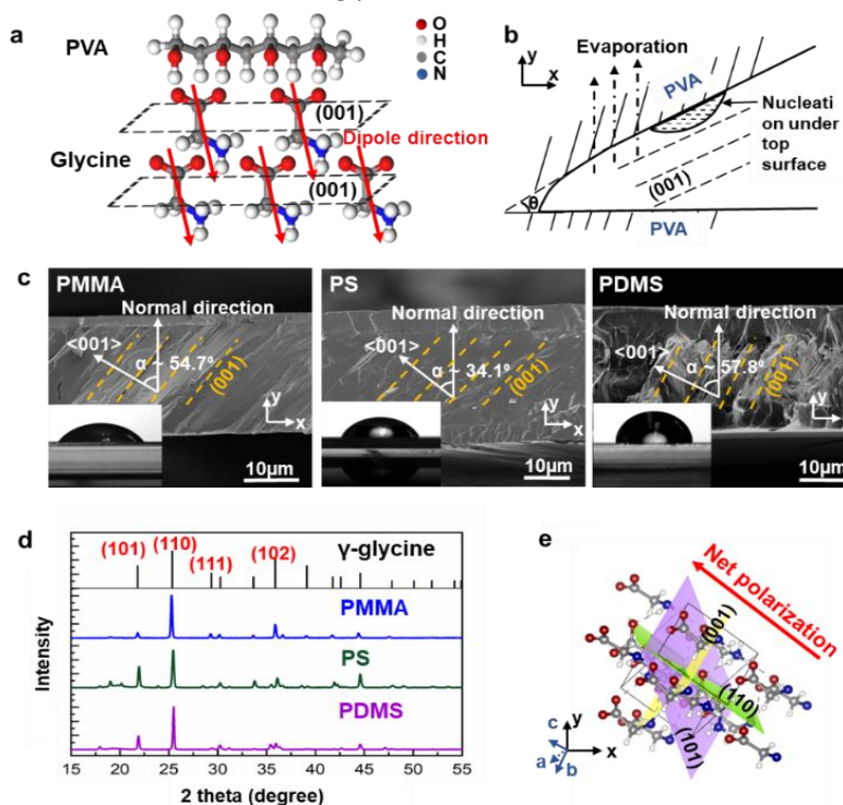
Figure 1. PVA-glycine films grown on different substrates. (a) Schematic of the hydrogen binding between glycine molecules and PVA chains. (b) Schematic illustration of the initial nucleation sites at the curved edge of the liquid film. (c) Cross-sectional SEM images of PVA-glycine films on PMMA, PS and PDMS substrates. Insets are corresponding contacting angle test. (d) XRD spectra of glycine-PVA films on PMMA (blue), PS (green) and PDMS (purple) substrates. (e) Schematic crystal structure of glycine crystal revealing the arrangement of (001), (101) and (110) planes.
