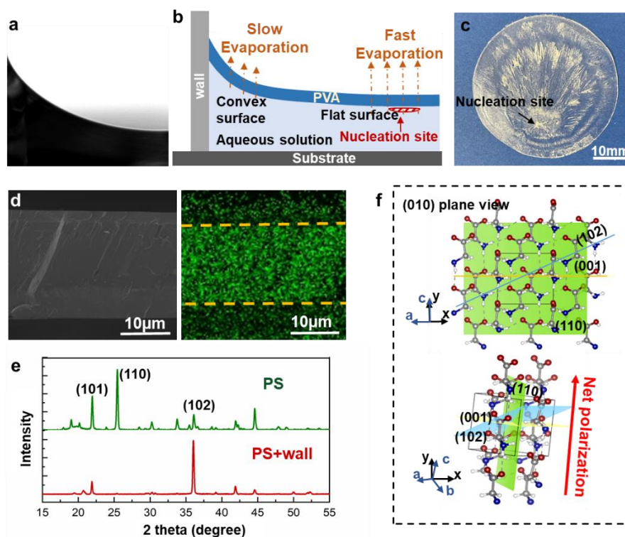
Figure 2. Growth of PVA-glycine films with a normal \langle 001 \rangle orientation. (a) Optical image showing the concaved solution surface along the edge when a vertical wall was applied. (b) Schematic illustration of nucleation site at the center flat area of the film. (c) Digital photograph of an as-grown film showing the nucleation spot and wafer scale size. (d) Cross-sectional SEM image (left) and corresponding EDS map of N (right) confirming the same PVA-glycine-PVA sandwiched structure. (e) XRD spectra of films grown on PS (green) and PS plus wall (red) substrates confirming the switching of film crystal orientation. (f) Schematic glycine crystal structure showing the direction relationship of (001) and (102).
