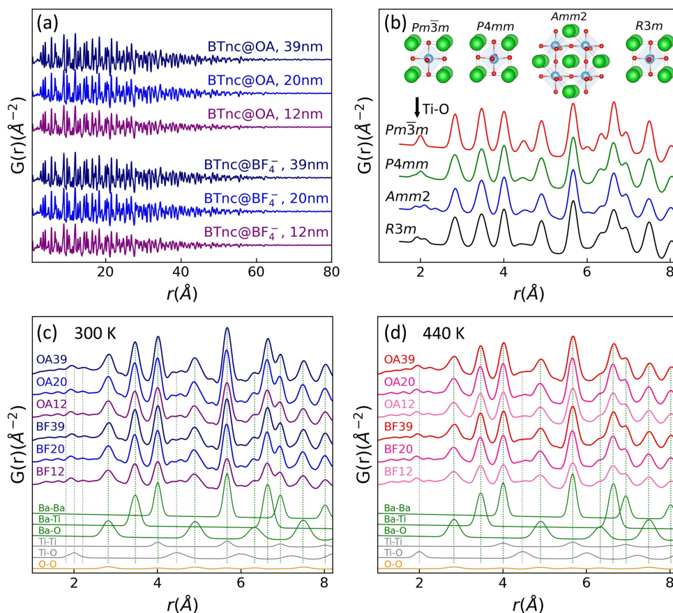
Fig. 3 (a) Comparison of the G(r) for different \text{BaTiO}_3 nanocubes over 80 \text{\AA} distance range. (b) Calculated PDFs from four crystallographic phases (cubic Pm\bar{3}m , tetragonal P4mm , orthorhombic Amm2 and rhombohedral R3m ) with a fixed U_{iso} value = 0.005 \text{\AA}^2 for all atoms, with corresponding models shown above. (c, d) The experimental local r range PDFs at 300 K and 440 K, along with simulated partial PDFs computed from P4mm and Pm\bar{3}m models, respectively.
