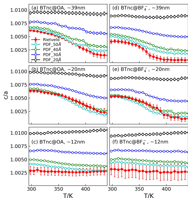
Fig. 5 Temperature dependence of tetragonality ( c/a ) ratios resulting from Rietveld and various real-space range PDF refinements for (a, d) \sim 39 nm, (b, e) \sim 20 nm, and (c, f) \sim 12 nm \text{BaTiO}_3 nanocubes capped with (a-c) OA and (d-f) \text{BF}_4^- .
