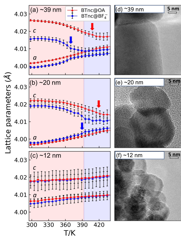
Fig. 2 Lattice parameters resulting from Rietveld refinement of 300 K to 440 K X-ray diffraction data using a P4mm model phase for average \text{BaTiO}_3 nanocube sizes of (a) \sim 39 nm, (b) \sim 20 nm and (c) \sim 12 nm. The color boundary shows the phase transition temperature of bulk \text{BaTiO}_3 while arrows have been added to call attention to inflection points in the nanocube data, indicating the temperature regimes of the diffuse phase transitions of the \text{BaTiO}_3 nanocubes. (d–f) show the high resolution TEM images corresponding to the various particle size samples.
