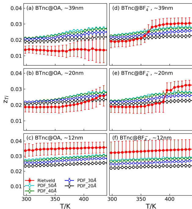
Fig. 6 Temperature dependence of z_{Ti} resulting from Rietveld and various real-space range PDF refinements for (a,d) \sim 39 nm, (b,e) \sim 20 nm, and (c,f) \sim 12 nm \text{BaTiO}_3 nanocubes capped with (a-c) OA and (d-f) \text{BF}_4^- .
