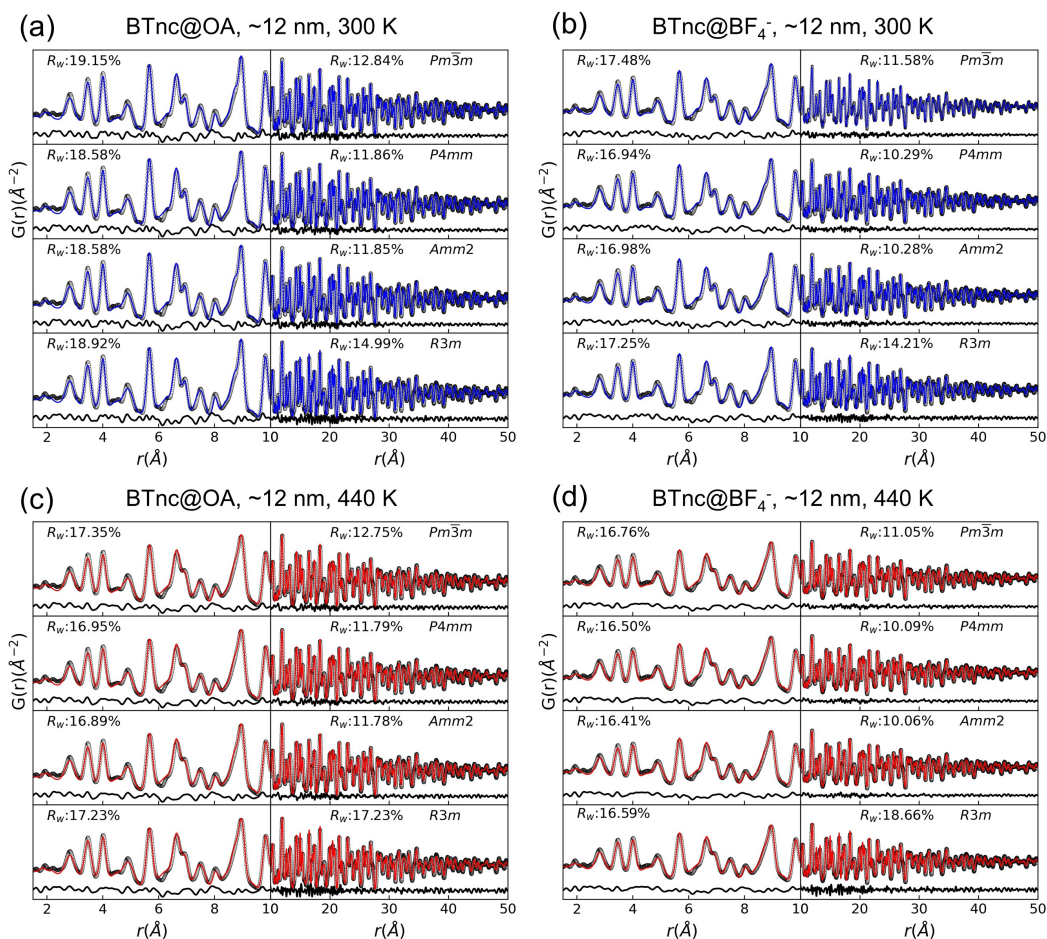
Fig. 4 PDF refinements of synchrotron X-ray data using centrosymmetric cubic Pm\bar{3}m , and non-centrosymmetric (tetragonal P4mm , orthorhombic Amm2 and rhombohedra R3m ) at (a, b) 300 K and (c, d) 440 K for BaTiO 3 \sim 12 nm nanocubes with OA and BF_4^- ligand capping.
