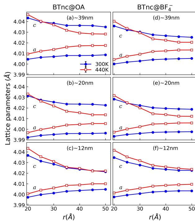
Fig. 7 The lattice parameters a and c resulting from PDF refinement with varying r_{max} range from 20 \text{ \AA} to 50 \text{ \AA} . Blue symbols correspond to 300 K data and red symbols correspond to 440 K data.
