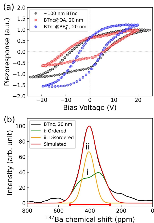
Fig. 8 (a) Normalized piezoresponse hysteresis loops of 20 nm BaTiO 3 nanocubes capped with OA and BF 4 - compared with the hysteresis loops of 100 nm BaTiO 3 nanocubes capped with OA. (b) Example deconvolution of 137 Ba NMR spectra (black). Curve i represents the ordered component (green line) and curve ii the disordered component (orange line). The red bar represents the range of the fitting algorithm.
