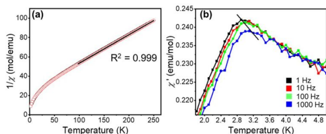
Figure 5. The temperature dependence of inverse DC magnetic susceptibility (a) and of in-phase AC susceptibility (b) for the bulk sample of \text{MnIn}_2\text{Se}_4 . The Curie-Weiss fit is shown with a solid black line in panel (a), while the black line in panel (b) is used to emphasize the frequency-dependent maximum characteristic of the spin-glass state.
