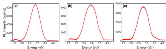
Figure 3. Photoluminescence spectra of bulk \text{MnIn}_2\text{Se}_4 (a) and of sheets collected at 5000 rpm (b) and 7500 rpm (c).
