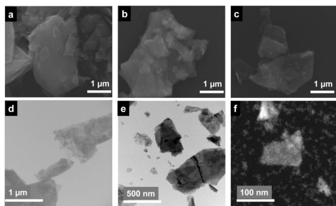
Figure 2. SEM images of exfoliated \text{MnIn}_2\text{Se}_4 samples isolated at 2000 rpm (a), 5000 rpm (b), and 7500 rpm (c), respectively, and the corresponding TEM images of sheets collected at 2000 rpm (d) and 5000 rpm (e) and an annual dark-field STEM image of sheets collected at 7500 rpm (f).
