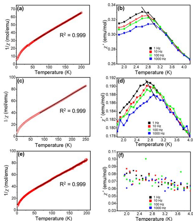
Figure 6. The temperature dependence of inverse DC magnetic susceptibility (left) and of in-phase AC magnetic susceptibility (right) for the sheets isolated at 2000 rpm (a, b), 5000 rpm (c, d), and 7500 rpm (e, f). The Curie-Weiss fits are shown with solid black lines in panels (a), (c), and (e), while in panels (b) and (d) the lines are used to emphasize the frequency-dependent maxima characteristic of the spin-glass state.
