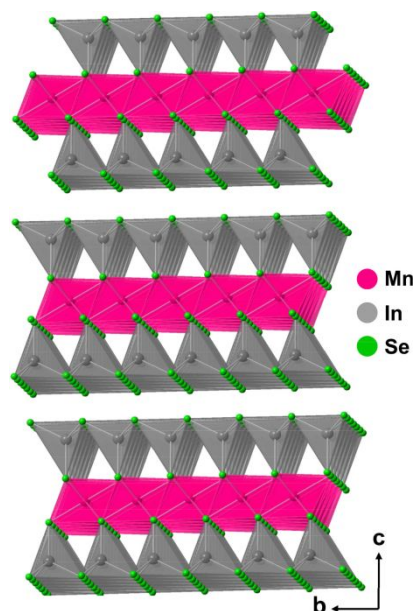
Figure 1. The layered crystal structure of MnIn 2 Se 4 , showing the van-der-Waals gaps between 7-atom-thick layers. The Se–Se distance between the layers is 3.868 Å.
