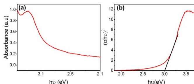
Figure 4. (a) UV-Vis absorption spectrum of the \text{MnIn}_2\text{Se}_4 sheets collected at 7500 rpm. (b) The Tauc plot used to evaluate the direct band gap of the material.
