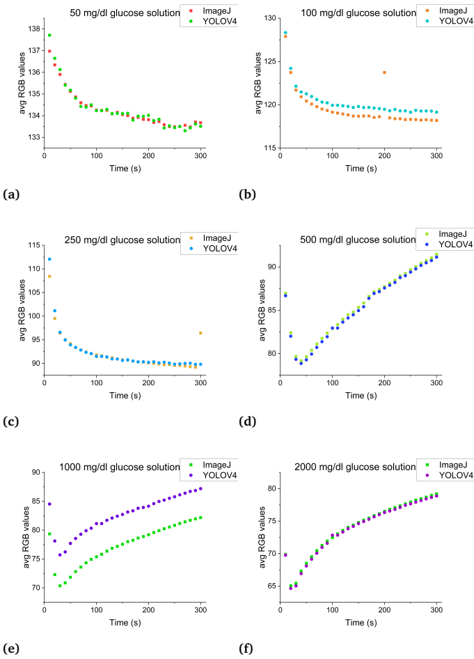
Fig. 6 Correlation between time and measured average RGB values and the comparison between ImageJ and Glucose detector measurements. a) 50 mg/dL glucose concentration. b) 100 mg/dL glucose concentration. c) 250 mg/dL glucose concentration. d) 500 mg/dL glucose concentration. e) 1000 mg/dL glucose concentration. f) 2000 mg/dL glucose concentration.
