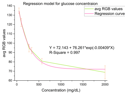
Fig. 7 Regression curve based on Glucose detector measurements
