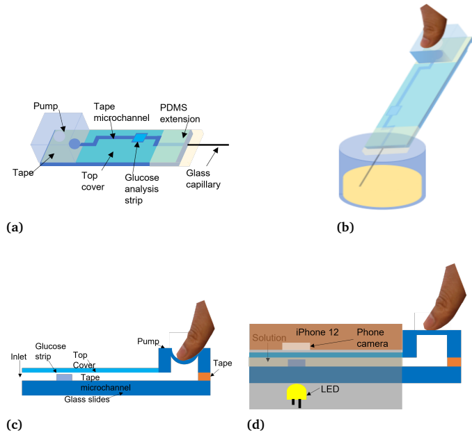
Fig. 3 Conceptual pictures of the principle of a microfluidic channel. a) Microfluidic device. b) Dip the microfluidic device into a container of solution. c) Apply pressure down the micropump to create a negative pressure environment. d) Microfluidic device in 3D printed phone holder after adsorption.
