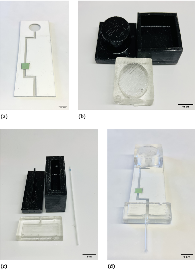
Fig. 2 Actual pictures of a microfluidic channel and molds for the PDMS components. a) Microfluidic channel. b) PDMS micropumps and 3D-printed molds. c) PDMS extension part, capillary and 3D-printed molds. d) Microfluidic device after assemble of all components.
