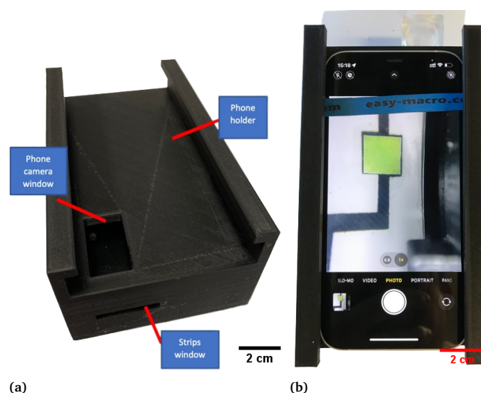
Fig. 1 Smartphone-based glucose detection platform. a) 3D-printed smartphone box. b) Actual image was taken after sliding the microfluidics device into the platform.
