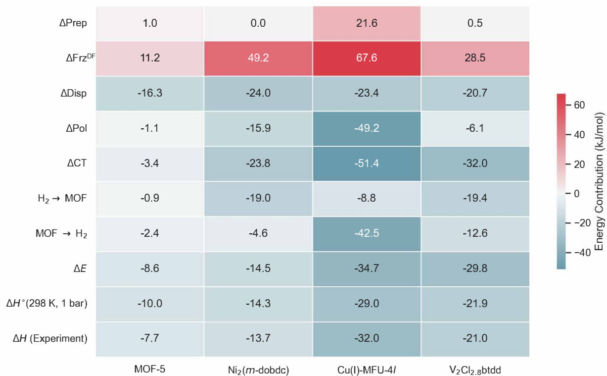
Fig. 9 A comparative summary of Energy Decomposition Analysis (EDA) (see Eq. 2 for definition of terms) of \text{H}_2 binding to four MOFs. \Delta\text{CT} contains forward ( \text{H}_2 \rightarrow \text{MOF} ) and back-donation ( \text{MOF} \rightarrow \text{H}_2 ) contributions. The MOFs are MOF-5, a material with no open metal sites (see Fig. 5), the Lewis acidic Ni(II) site in \text{Ni}_2(m\text{-dobdc}) (see Fig. 6), and \pi -basic Cu(I) and V(II) sites in \text{Cu(I)-MFU-4l} (see Fig. 7) and \text{V}_2\text{Cl}_{2.8}(\text{btdd}) (see Fig. 8) respectively. \Delta H^\circ(\text{T}) values are reported at 298 K and 1 bar, and compared to experimental values.
