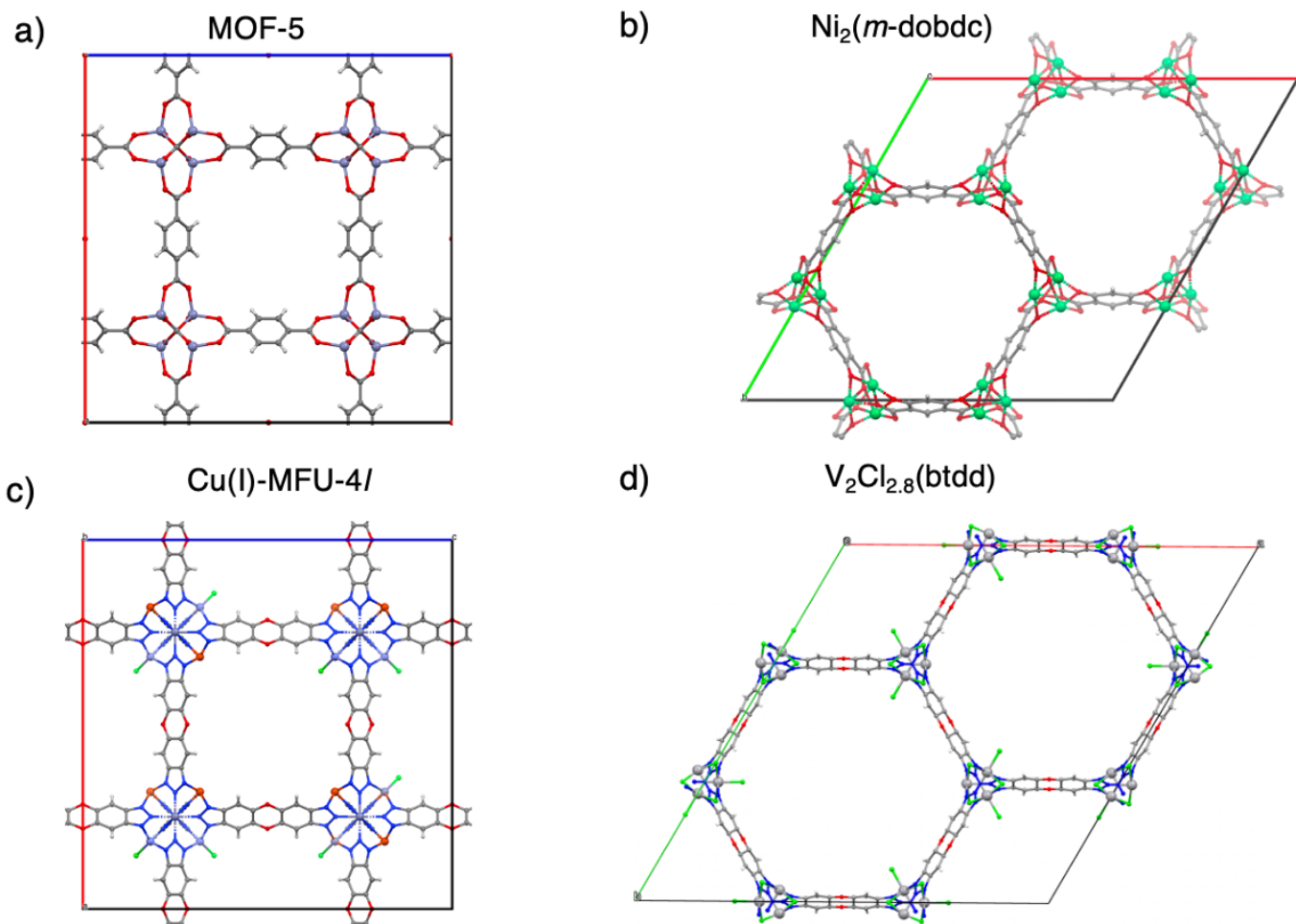
Fig. 1 Metal organic frameworks (MOFs) are promising materials for H_2 storage because they combine 3-d pore structure with enormous scope for chemical tailoring of H_2 binding sites, as illustrated by the crystal structures shown here. a) MOF-5, b) Ni_2(m\text{-dobdc}) , c) Cu(I)\text{-MFU-4l} and d) V_2Cl_{2.8}(btdd) . Grey, blue, red, and light green represent carbon, nitrogen, oxygen, and chlorine, respectively. Zinc sites are shaded blue-grey in a), nickel rendered green in b), copper rendered orange in c), and vanadium grey in d).
