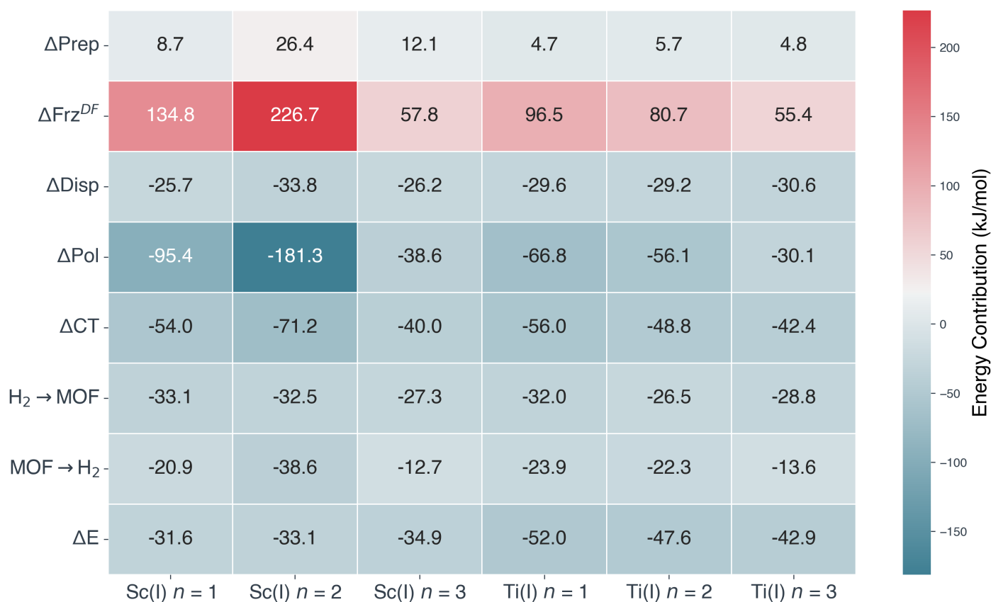
Fig. 15 Binding energies and their EDA (see Eq. 2) for the binding of three equivalents of \text{H}_2 at Sc(I) and Ti(I) sites in MFU-4l. The Sc(I) sites demonstrate a weak dependence of binding on the number of bound \text{H}_2 , which is desirable for \text{H}_2 storage purposes. By contrast, the Ti(I) sites show fall-off in binding with number of bound \text{H}_2 . See text and Fig. 16 for the origin of the remarkable change in the \Delta\text{Frz}^{\text{DF}} and \Delta\text{Pol} EDA components for the Sc(I) site with 2 bound \text{H}_2 .
