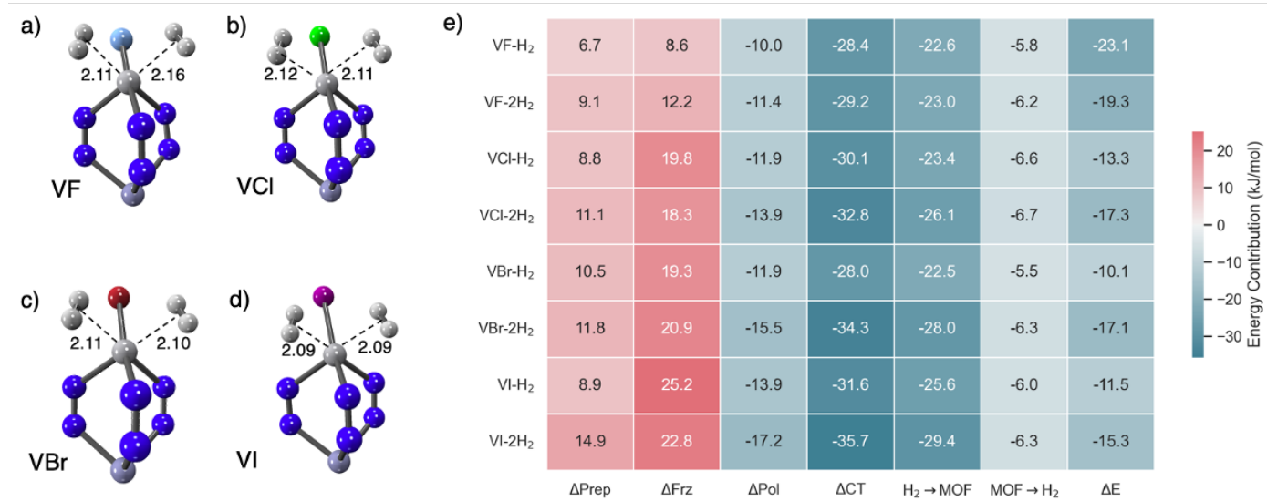
Fig. 13 Multiple H 2 ligations in V(II)-X-MFU-4l, (X = F, Cl, Br, I) (a-d) and EDA of the quite wide range of adsorption behaviour as a function of the halide counterion (e). Dative effects, particularly forward donation, dominate the binding energy. Distances are reported in Å, and energy contributions in kJ/mol in (e).
