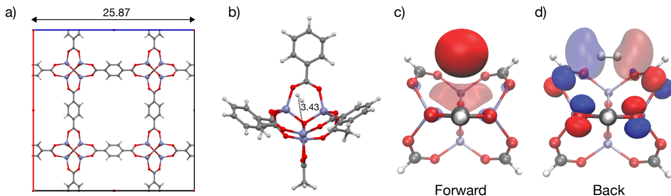
Fig. 5 Illustration of hydrogen binding at the the cup site in MOF-5, a framework without open metal sites. a) Cubic unit cell of MOF-5. b) Cluster model for MOF-5 depicting relatively weak \text{H}_2 binding at the \alpha (cup) site, as implied by the long coordination distance. Dative contributions to \text{H}_2 binding are very weak in this dispersion-dominated interaction, consistent with the delocalized character of the framework acceptor and donor COVP orbitals shown in c) and d) together with the corresponding \text{H}_2 \sigma donor and \sigma^* acceptor orbitals. Distances are labelled in Å with Zn(II) rendered in blue-grey, O in red, H in light grey and C in dark grey. The orbitals were plotted with an isosurface of \pm 0.07\text{\AA} . The smaller formate model was used to visualize charge transfer COVP orbitals.
