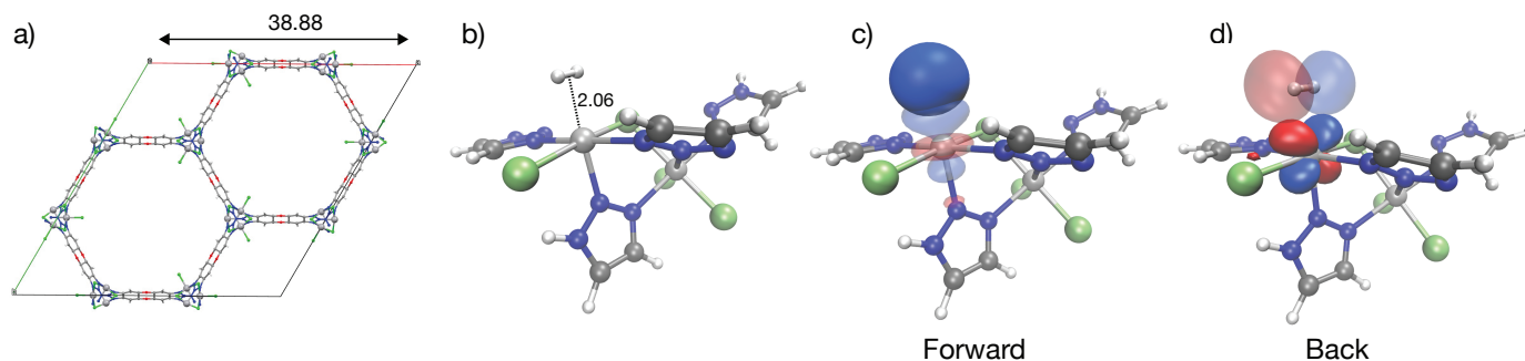
Fig. 8 Illustration of \text{H}_2 binding at the V(II) site in \text{V}_2\text{Cl}_{2.8}(\text{btdd}) . Panel a) shows the unit cell and b) shows the DFT optimized geometry for a two-site cluster model representation of \text{H}_2 binding to the OMS in the material. Significant charge transfer orbitals for forward and back-donation are depicted in c) and d). V(II)- \text{H}_2 backbonding at this site is attenuated in comparison to Cu(I)- \text{H}_2 interactions in Cu(I)-MFU-4l. Distances are labelled in Å with V(II) rendered in grey, N in blue, Cl in green, H in light grey and C in black. The orbitals were plotted with an isosurface of \pm 0.07 \text{ \AA} .
