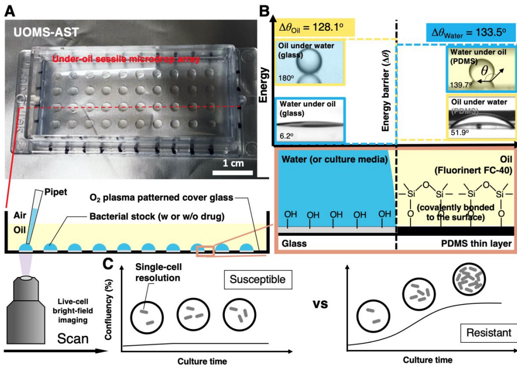
Fig. 1 The configuration and physics of UOMS-AST. (A) A UOMS-AST device fabricated with a 1-well chambered coverglass (Nunc Lab-Tek - borosilicate glass #1.0 - medical grade silicone adhesive, 6 cm × 2.4 cm, 0.13-0.17 mm in bottom thickness). The glass surface was patterned for an array (4 × 10) of under-oil (Fluorinert FC-40, or FC40, 1.5 mL per 1-well chambered coverglass) sessile (i.e., surface-attached) microdroplets (2 mm in diameter). 2 \mu L of bacterial stock with or without antimicrobial was inoculated to each spot under oil by regular single-channel pipetting. (B) A schematic shows the surface chemistry contrast for liquid confinement with the energy (or virtual) barrier. The glass surface was modified by a monolayer of covalently bonded, polydimethylsiloxane (PDMS)-silane molecules and then selectively patterned by oxygen plasma (Fig. S1). (C) A schematic shows the live-cell, bright-field imaging in UOMS-AST and the detection of antimicrobial susceptibility/resistance based on confluency of bacterial cells in the field of view.
