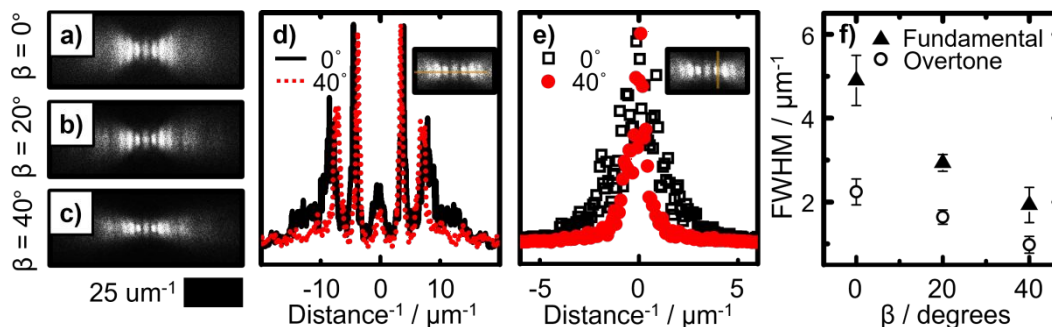
Figure 2. (a)-(c) 2D FTs generated from SEM data of the deposits depicted in Figure 1(b)-(d) respectively. (d) Fourier spectra representing the intensity along the horizontal centerlines of the 2D FTs depicted in (a) and (c). (e) Fourier spectra representing the intensity along the vertical centerlines of the positive fundamental modes in the 2D FTs in (a) and (c). (f) FWHM of fit curves of spectral profiles similar to those in (e) for the positive fundamental and first overtone modes in the 2D FTs in (a)-(c) as a function of \beta .
