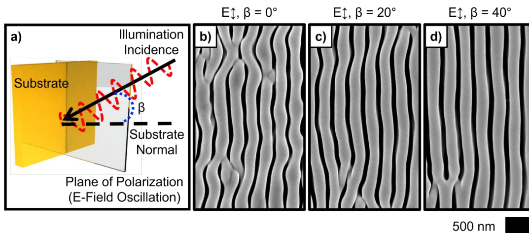
Figure 1. (a) Schematic illustration of electrode substrate illumination with linearly polarized light inclined in the plane of the polarization. (b)-(d) Representative SEMs of deposits generated with vertically polarized ( E \uparrow ) \lambda_{\text{avg}} = 626 nm illumination with the indicated inclination ( \beta ) from the substrate normal in the plane of the polarization.
