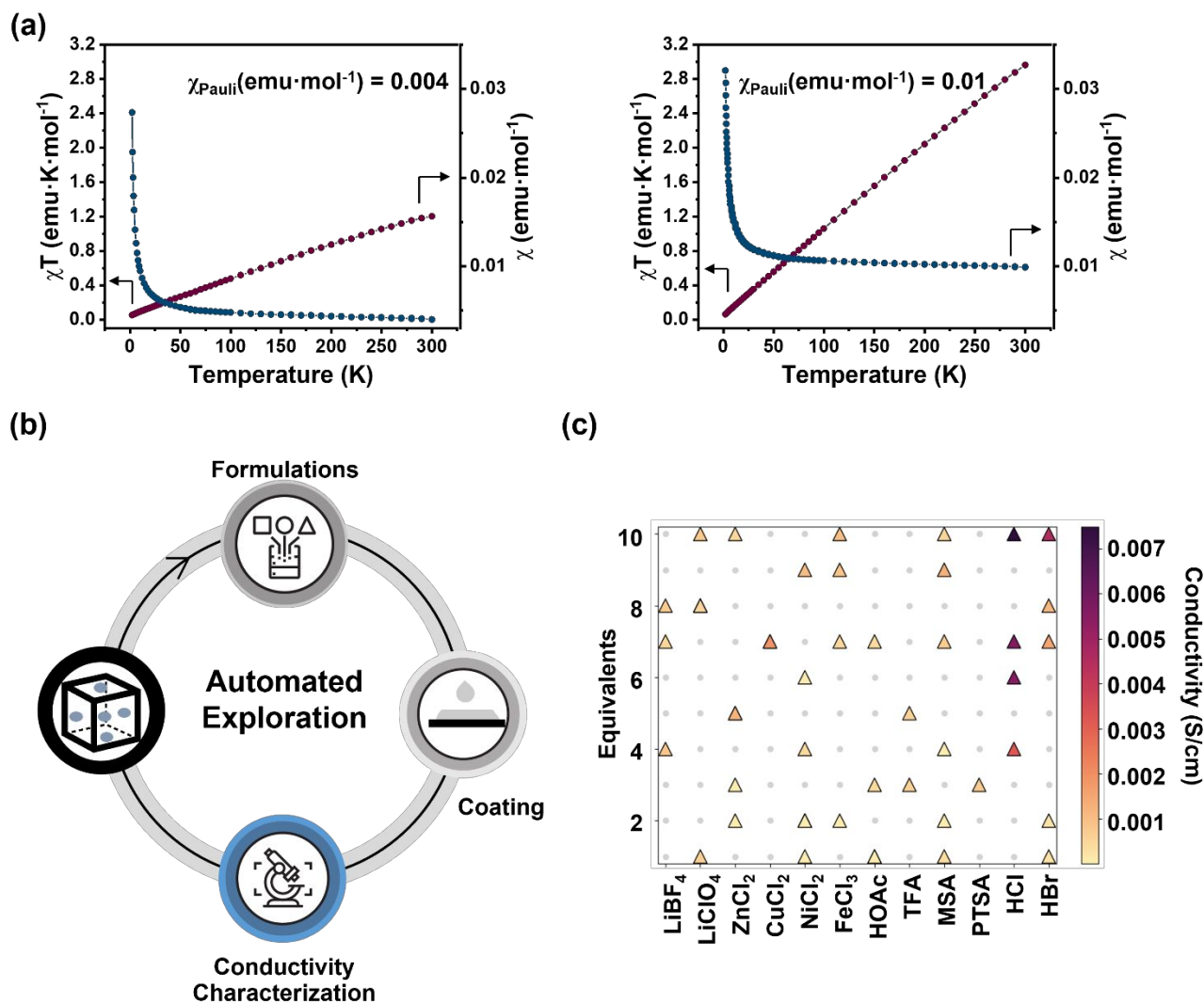
Figure 4. (a) Temperature-varied magnetic susceptibility of 2 equivalents PTSA mixed 1a _PS (left) and 1a _PS (right); (b) Workflow of the automated conductivity screening by Polybot; (c) Plot of conductivity data points measured by Polybot.
