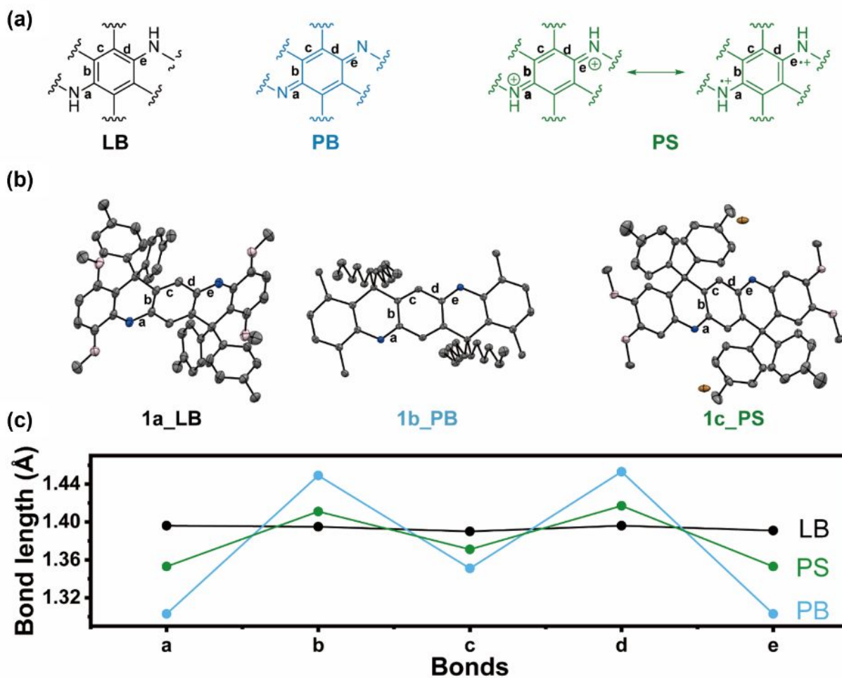
Figure 2. (a) Structures and bond labeling of the LB, PB and PS forms; (b) Single-crystal structures
