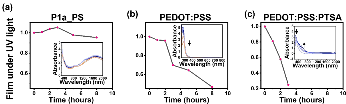
Figure 5. Plots of UV-vis-NIR absorbance intensity at \lambda_{\max} as a function of time under 254 nm and 365 nm UV irradiation (10 mW cm -1 ): (a) P1a_PB + 4 equivalents of PTSA ( P1a_PS ); (b) PEDOT:PSS; and (c) PEDOT:PSS + 4 equivalents of PTSA film. The insets are the corresponding UV-vis-NIR absorption spectra over time.
