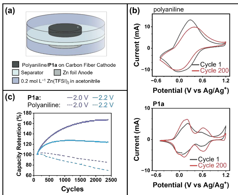
Figure 6. (a) Setup of supercapacitor for measurements. (b) 3-electrode cyclic voltammetry (CV) of polyaniline and P1a over a 1.7 V window. (c) Plot of capacity against number of cycles of 2-electrode polyaniline and P1a devices over a 0.2 ~ 2V and 0.2 ~ 2.2V range, respectively.
