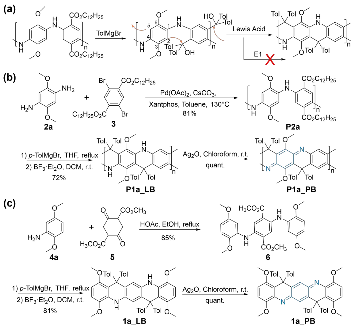
Scheme 1. (a) Key steps during the synthesis: Grignard reaction to generate the tertiary alcohol groups followed by Lewis acid catalyzed intramolecular Friedel-Crafts cyclization. (b) Synthesis of P1a_LB and P1a_PB . (c) Synthesis of 1a_LB and 1a_PB .
