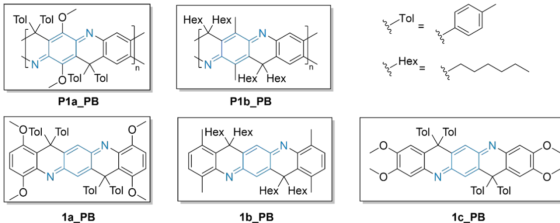
Figure 1. (a) Structural formulas of the previously reported ladder polymer f-LPANI and small molecule TolMSQ . (b) Structural formulas of ladder polymers P1a and P1b , as well as small molecule model compounds 1a , 1b , and 1c , all studied in this work. The suffix “ PB ” in these labels indicates that these structures are shown in the form of pernigraniline base.
