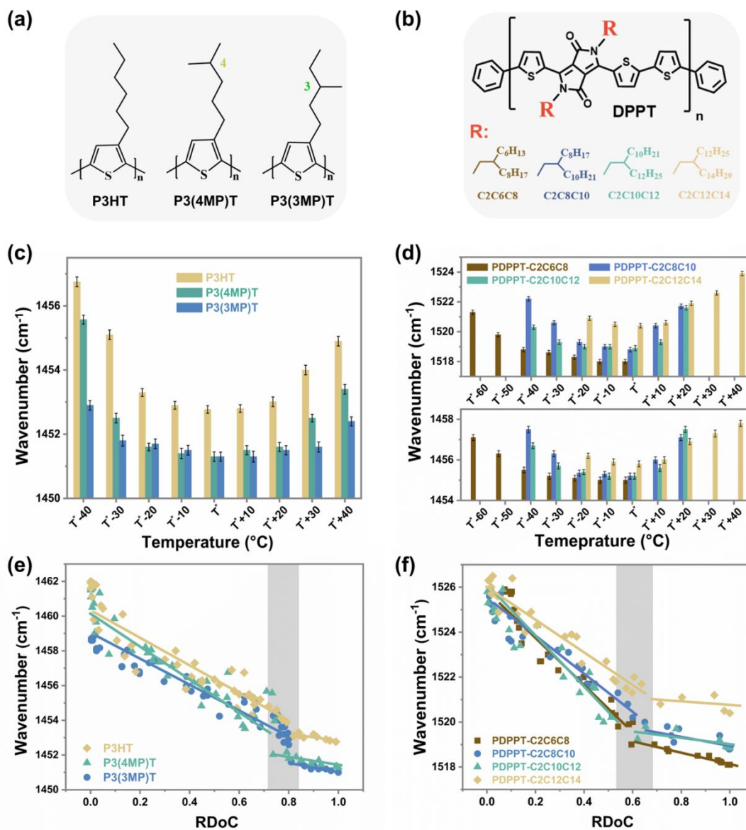
Fig. 3 The disparity between the crystallization and the segmental order of PDPPT-based and P3AT films with different side chain structures. Chemical structures of (a) P3AT polymers and (b) PDPPT-based polymers with different side chain structures. The variations of saturated wavenumbers of C=C modes of (c) P3AT polymers and (d) PDPPT-based polymers with different crystallization temperatures. The variations of wavenumbers of C=C modes of (e) P3AT polymers and (f) PDPPT-based polymers with different RDoC.
