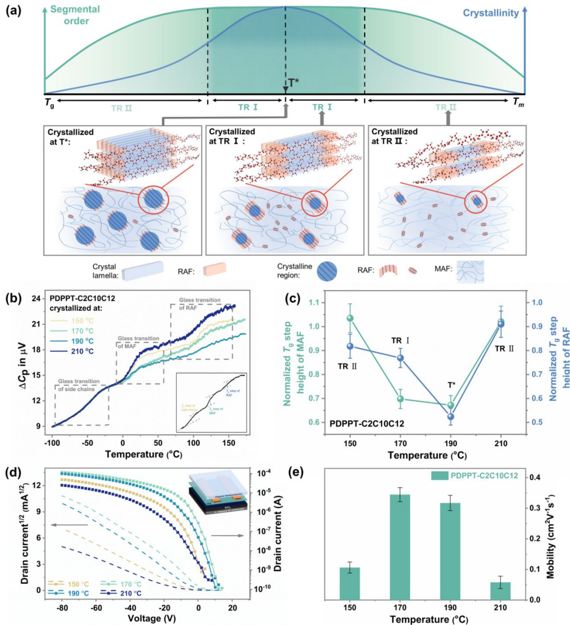
Fig. 4 The influence of segmental order and crystallization on the chain dynamics and electrical performance. (a) Schematic of microstructure evolution in CP films when crystallized at three different temperature regions. (b) Glass transition behavior of the PDPPT-C2C10C12 film after crystallized at 150 °C, 170 °C, 190 °C and 210 °C. (c) Normalized T_g step heights of MAF and RAF in the PDPPT-C2C10C12 film after crystallizing at different temperatures. (d) Transfer characteristics for OFET devices of PDPPT-C2C10C12 annealed at different temperatures, and (e) average charge-carrier mobilities of PDPPT-C2C10C12 film calculated in saturation mode ( V_d = - 80 V ).
