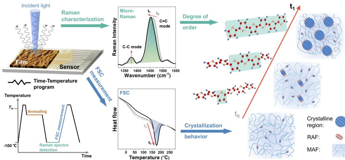
Fig. 1 Modulating and probing microstructure of conjugated polymers by integrated ultrafast calorimetry and micro-Raman spectroscopy. Left: schematic of this integrated technique. The time-temperature program used in this study was carried out by the chip sensor temperature controller. The growth of crystalline domain was identified by the evolution of melting peak collected through FSC. The degree of segmental order was analyzed by the Raman shift of C=C modes through resonant micro-Raman spectroscopy.
