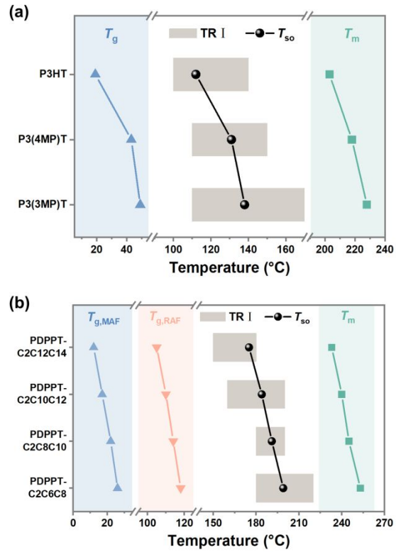
Fig. 5 The relationship between TR I, T_g and T_m . (a) T_g and T_m , T_{so} and TR I of various P3ATs films. (b) T_g and T_m , T_{so} and TR I of various PDPPT-based films.
