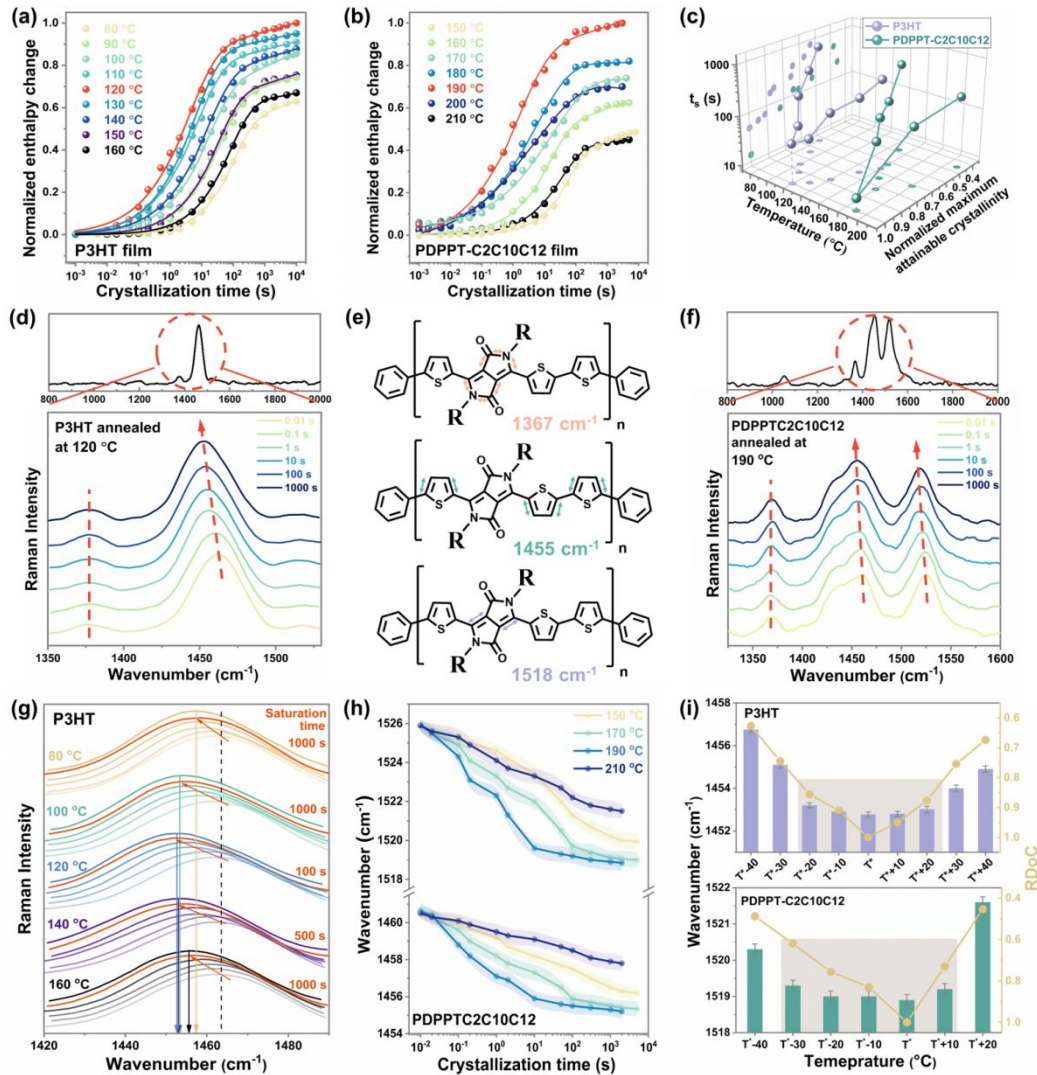
Fig. 2 The evolution of the segmental order of P3HT and PDPPT-C2C10C12 during the isothermal crystallization. Normalized melting enthalpy change of (a) P3HT film and (b) PDPPT-C2C10C12 film as a function of the crystallization time. (c) The variations of t_s and normalized maximum attainable crystallinity of P3HT and PDPPT-C2C10C12 films with crystallization temperatures. (d) Raman spectra of P3HT film crystallized at 120 °C. (e) Diagram illustrating the dominant bond stretches associated with the main Raman active vibrational modes of PDPPT-based polymers centered around 1367, 1455 and 1518 \text{cm}^{-1} . (f) Raman spectra of PDPPT-C2C10C12 film crystallized at 190 °C for different time. (g) The shifts of C=C mode of P3HT film with crystallization time when crystallized at different temperatures. The gradient in color from light to deep indicates the crystallization time from 0.01 s to 3000 s. The dashed line and solid lines indicate the wavenumber of C=C mode at a fully amorphous state and final saturation state at different crystallization temperatures, respectively. (h) The variations of C=C modes of PDPPT-C2C10C12 film with crystallization time when crystallized at different temperatures. (i) The saturated wavenumbers of C=C modes and RDoC of P3HT and PDPPT-C2C10C12 films at different crystallization temperatures.
