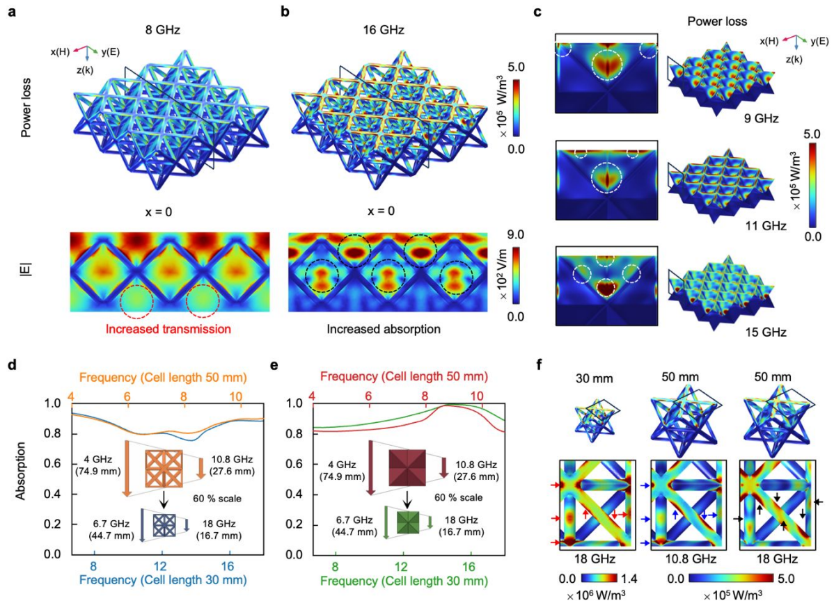
1 2 Fig 3. EM wave absorbing mechanisms of octet-truss and octet-foam. Power loss density and electric field plot on a 50 mm 3 octet-truss structure at (a) 8 GHz and (b) 16 GHz. (c) Power loss density plot across a 50 mm octet-foam at 9 GHz (top), 11 4 GHz (middle), and 15 GHz (bottom). (d)-(e) Exploring EM wave absorption in correlation to the relative cell length of octet- 5 truss and octet-foam. (f) A comparative assessment of power loss density plot of octet-truss under equal relative cell length 6 conditions against equal incident wavelength conditions. 7
