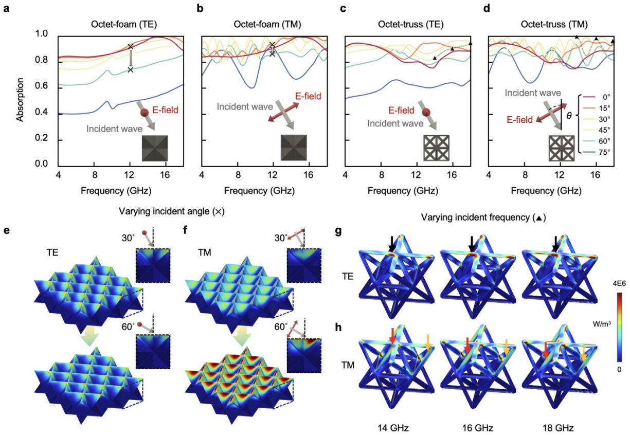
1 2 Fig 5. Comparative examination of electromagnetic wave absorption in octet-truss and octet-foam with varied incident 3 wave angles and polarization. Depicting the EM wave absorptions of (a), (b) octet-foam and (c), (d) octet-truss with respect 4 to transverse electric (TE) and transverse magnetic (TM) polarizations. Analyzing the power loss density plot of octet-foam at 5 incident angles of 30° and 60° for (e) TE and (f) TM polarization and octet-truss at 14 GHz, 16 GHz, and 18 GHz under a 45° 6 incident angle for both (g) TE and (h) TM polarizations. 7
